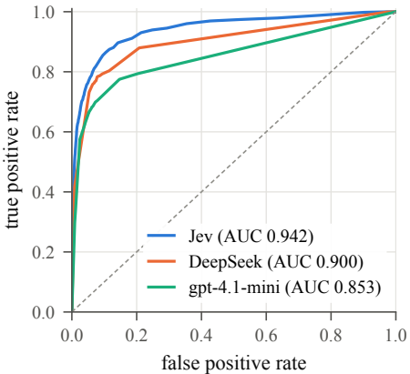
(a) separating gold evidence
