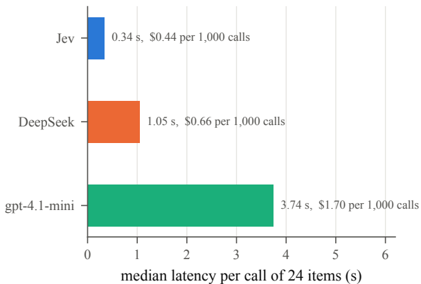
(b) latency and price of one call
