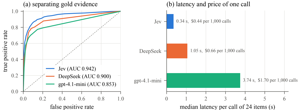
Figure 3: Jev and two LLM judges on the same 14,359 records: (a) ROC curves for separating gold evidence, pooled over records; (b) median latency and list price of one call on 24 records, in which Jev also answers whether each is no longer current.
