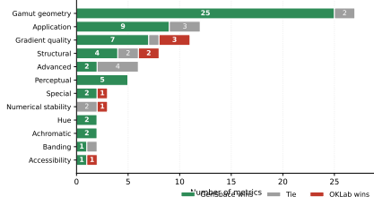
Figure 6: GenSpace v0.11.1 vs OKLab — per-category breakdown of the 83 internal ColorBench metrics. Headline tally including the 7 independent gradient/palette metrics is 66W / 9L / 15T (Table 5). Categories ordered by total metric count.
