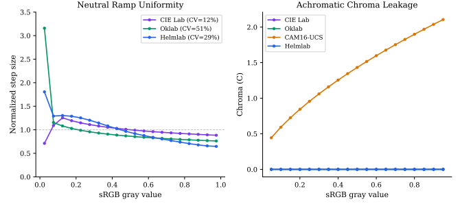
Figure 5: Left: neutral ramp step uniformity. Right: achromatic chroma leakage. HELMLAB’s NC guarantees C < 10^{-6} for all grays.
