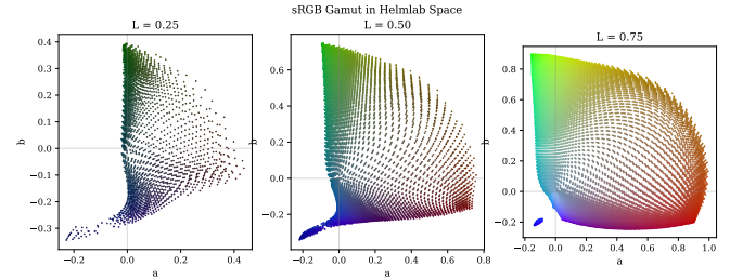
Figure 7: sRGB gamut in HELMLAB a - b plane at three L levels. Points colored by their sRGB values.
