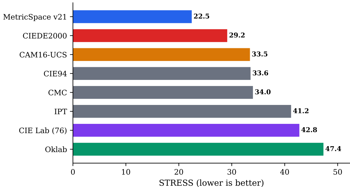
Color Difference Prediction — COMBVD (3813 pairs)
