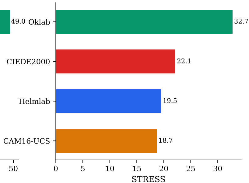
MacAdam 1974 (128 pairs)
