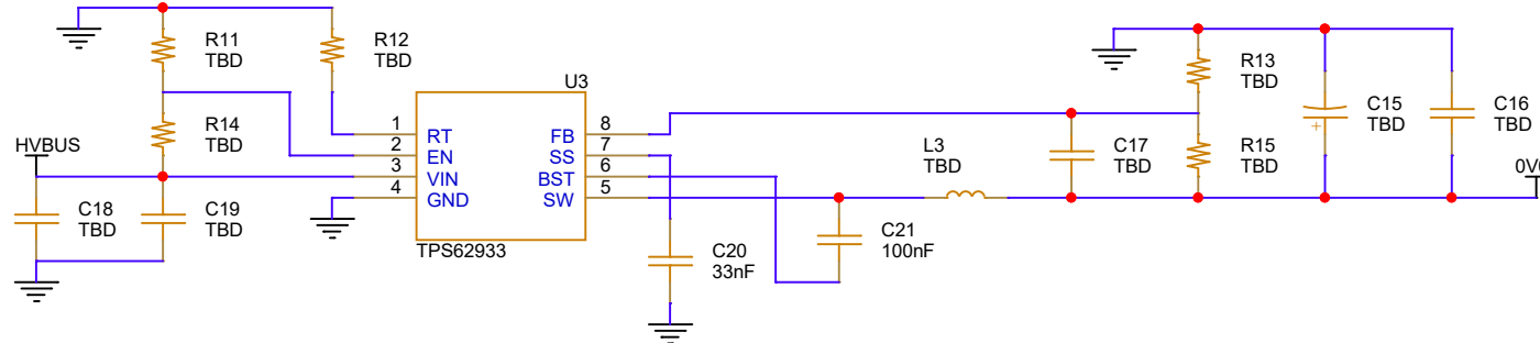
6-18V UNREG BUS TO ADDITIONAL RAIL (VOUT CAN BE ADJUSTED VIA THE FB VOLTAGE DIVIDER)
