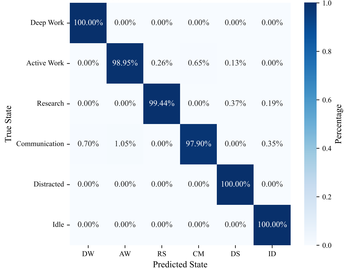
(b) Confusion Matrix (Normalized)
