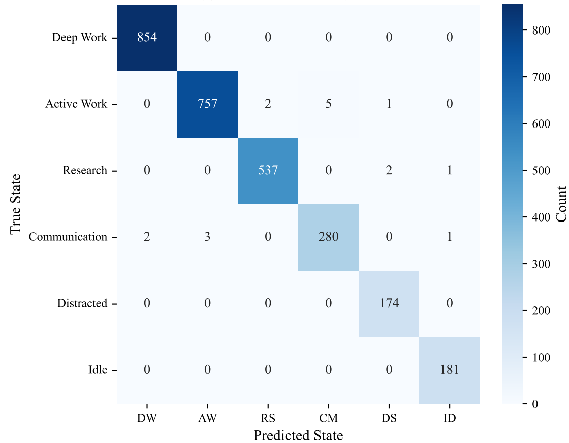
(a) Confusion Matrix (Counts)
