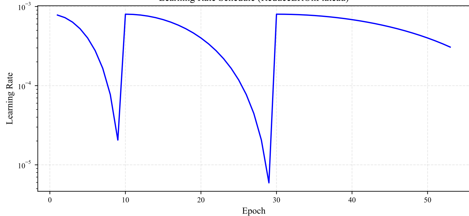
Learning Rate Schedule (ReduceLROnPlateau)
