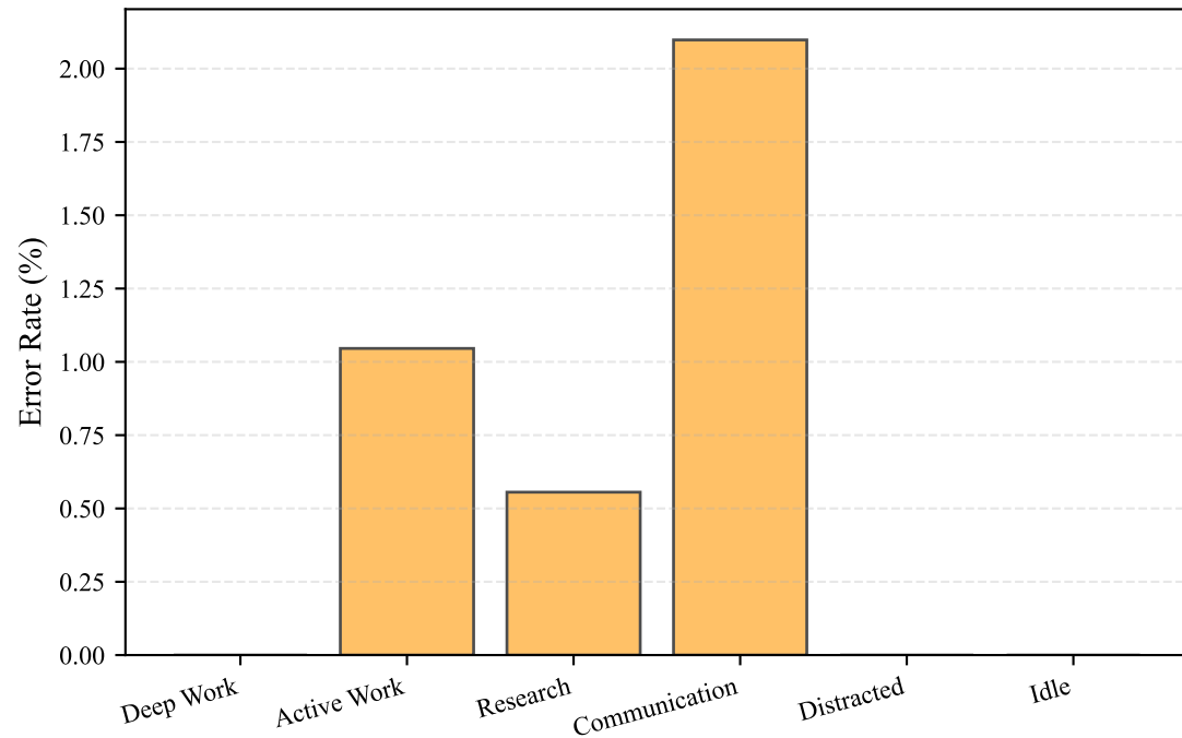
(b) Error Rate by State
