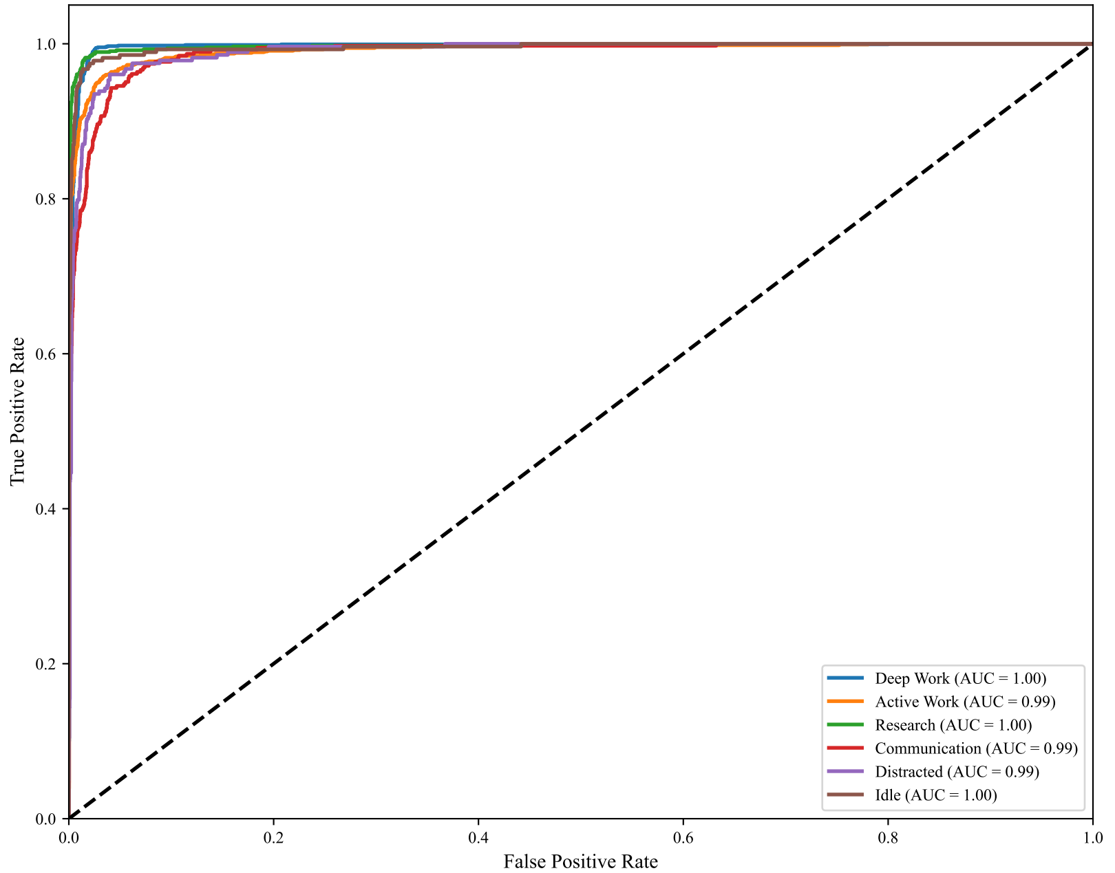
ROC Curves by Class
