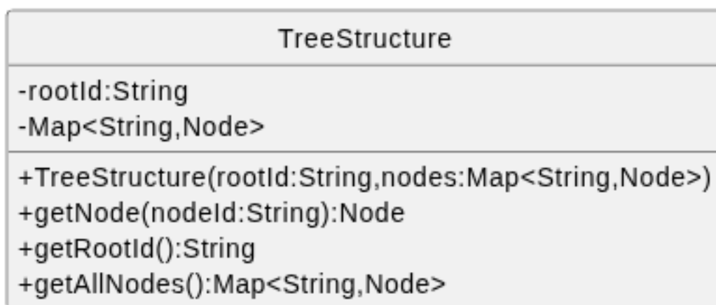
Figura 192: TreeStructure
