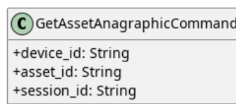
Figura 88: GetAssetAnagraphicCommand
