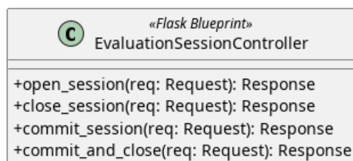
Figura 133: EvaluationSessionController
