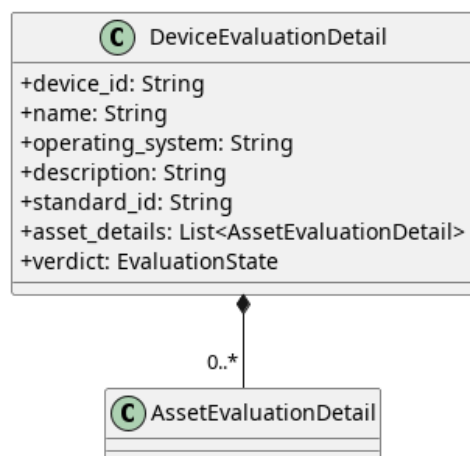
Figura 26: DeviceEvaluationDetail
