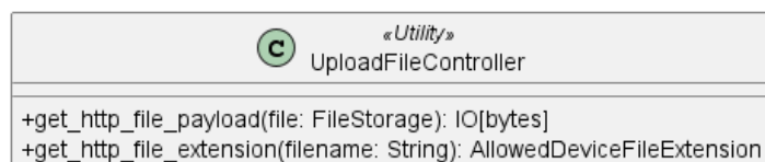
Figura 104: UploadFileController
