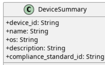
Figura 31: DeviceSummary
