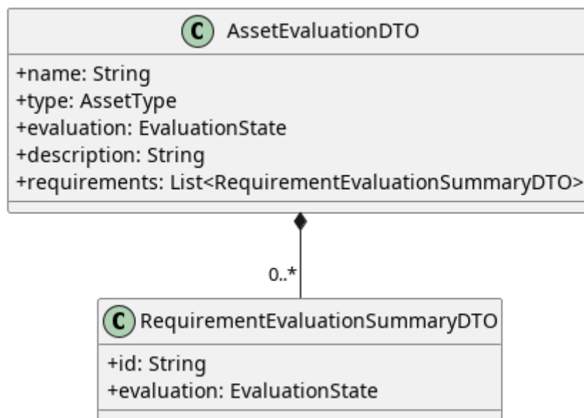
Figura 97: AssetEvaluationDTO
