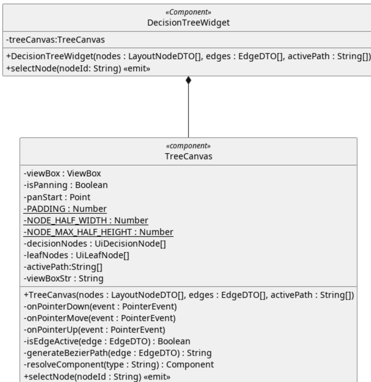
Figura 214: DecisionTreeWidget
