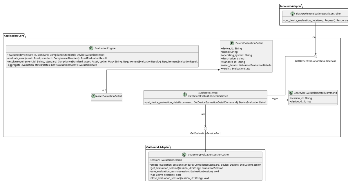
Figura 65: GetDeviceEvaluationDetail
