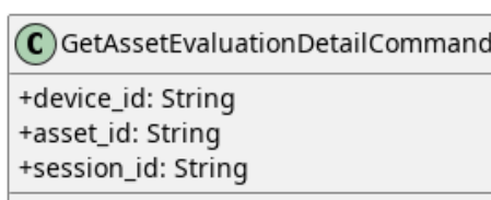
Figura 94: GetAssetEvaluationDetailCommand
