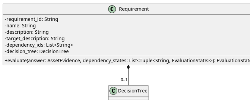
Figura 13: Requirement
