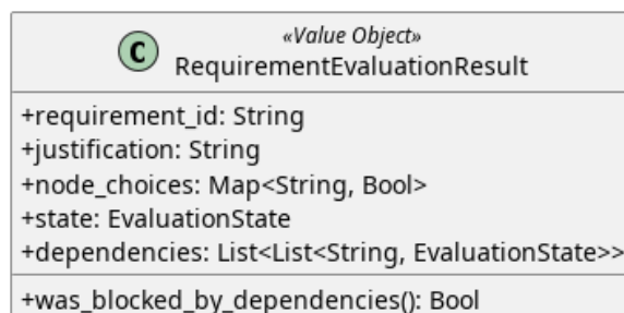
Figura 21: RequirementEvaluationResult
