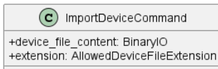
Figura 108: ImportDeviceCommand
