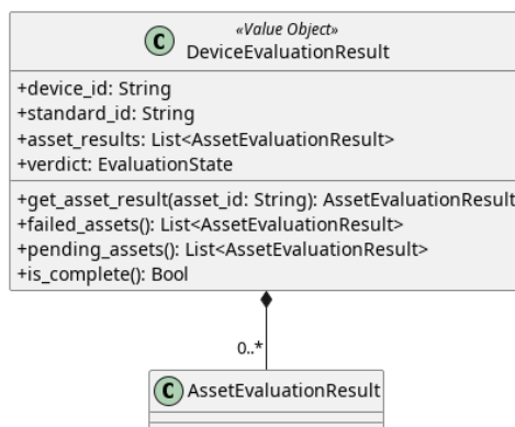
Figura 23: DeviceEvaluationResult
