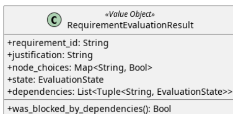
Figura 20: RequirementEvaluationResult
