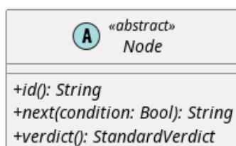
Figura 14: Node
