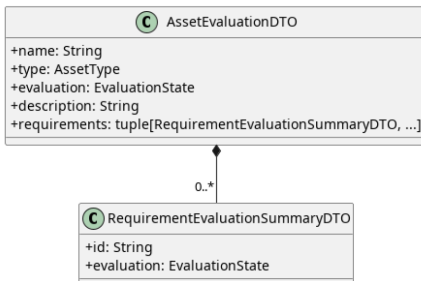
Figura 96: AssetEvaluationDTO
