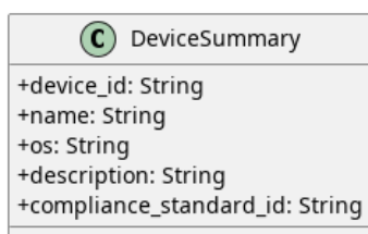
Figura 30: DeviceSummary
