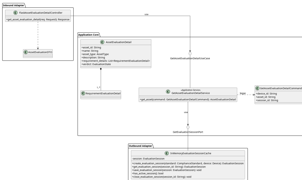
Figura 91: GetAssetEvaluationDetail
