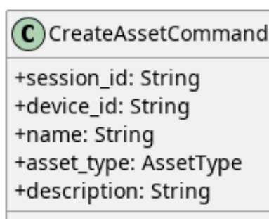
Figura 73: CreateAssetCommand
