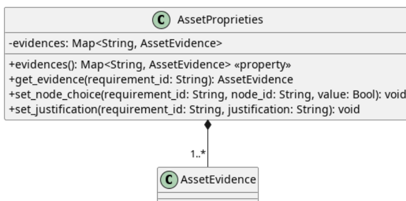
Figura 8: AssetProprieties
