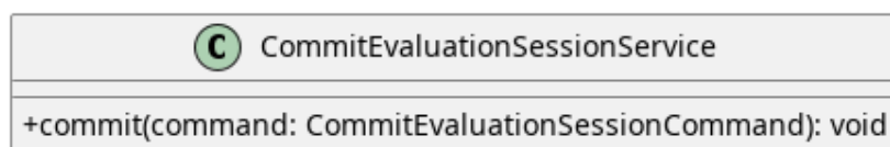
Figura 135: CommitEvaluationSessionService
