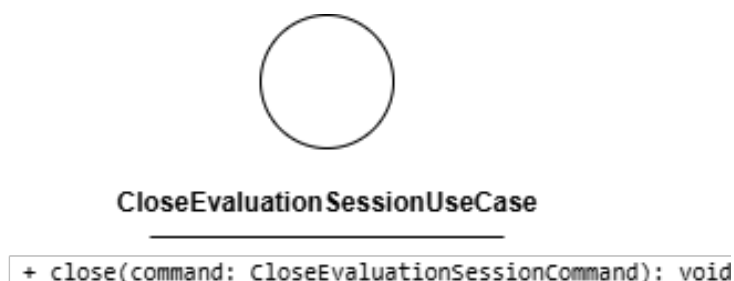
Figura 138: CloseEvaluationSessionUseCase
