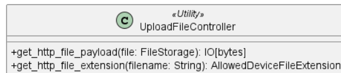
Figura 104: UploadFileController
