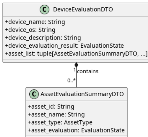
Figura 69: DeviceEvaluationDTO
