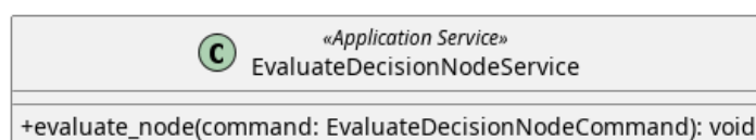
Figura 146: EvaluateDecisionNodeService
