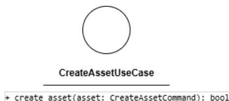
Figura 72: CreateAssetUseCase
