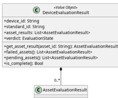
Figura 22: DeviceEvaluationResult
