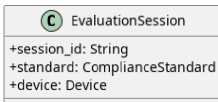
Figura 27: EvaluationSession
