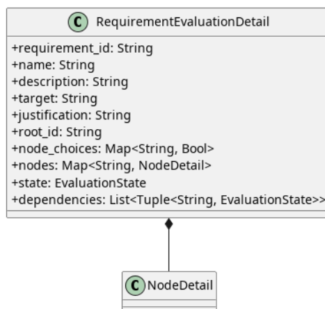
Figura 24: RequirementEvaluationDetail
