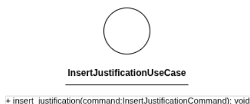
Figura 149: InsertJustificationUseCase
