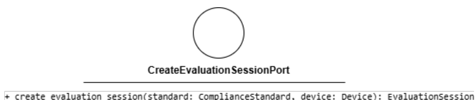
Figura 132: CreateEvaluationSessionPort
