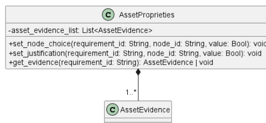
Figura 41: AssetProprieties
