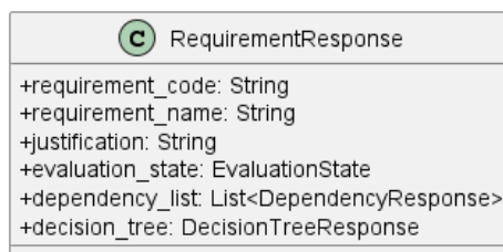
Figura 127: RequirementResponse
