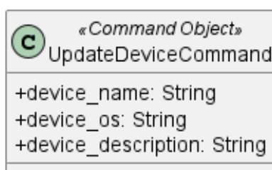
Figura 19: UpdateDeviceCommand
