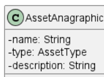
Figura 40: AssetAnagraphic
