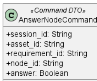
Figura 120: AnswerNodeCommand
