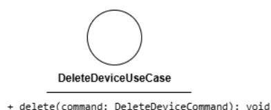
Figura 13: DeleteDeviceUseCase
