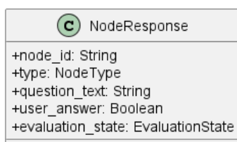
Figura 129: NodeResponse
