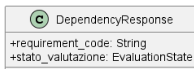
Figura 130: DependencyResponse
