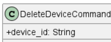
Figura 14: DeleteDeviceCommand
