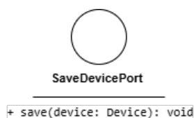
Figura 21: SaveDevicePort
