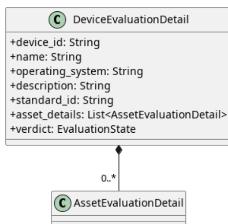
Figura 26: DeviceEvaluationDetail
