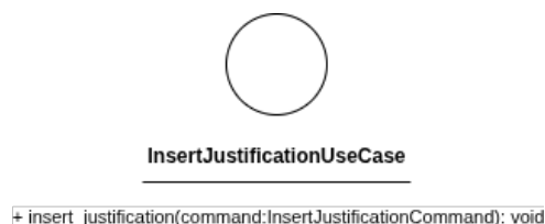
Figura 156: InsertJustificationUseCase
