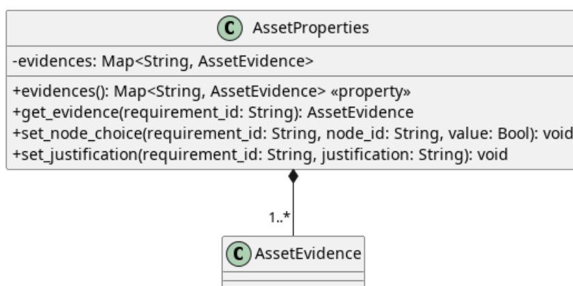
Figura 8: AssetProperties
