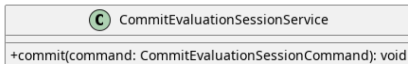
Figura 142: CommitEvaluationSessionService
