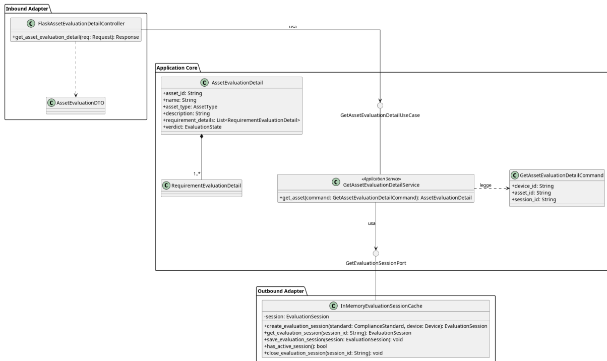
Figura 91: GetAssetEvaluationDetail
