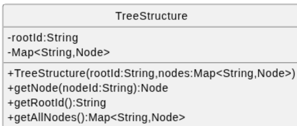
Figura 192: TreeStructure
