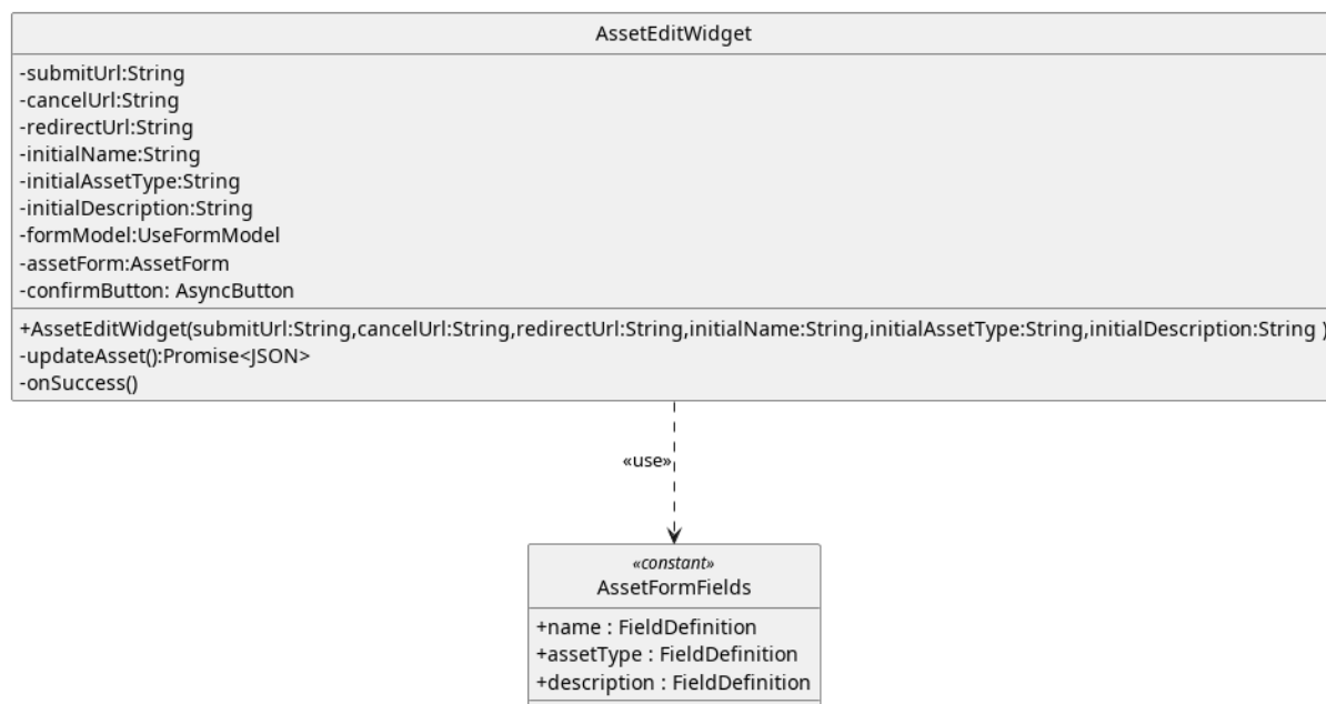
Figura 176: Widget - AssetEditWidget
