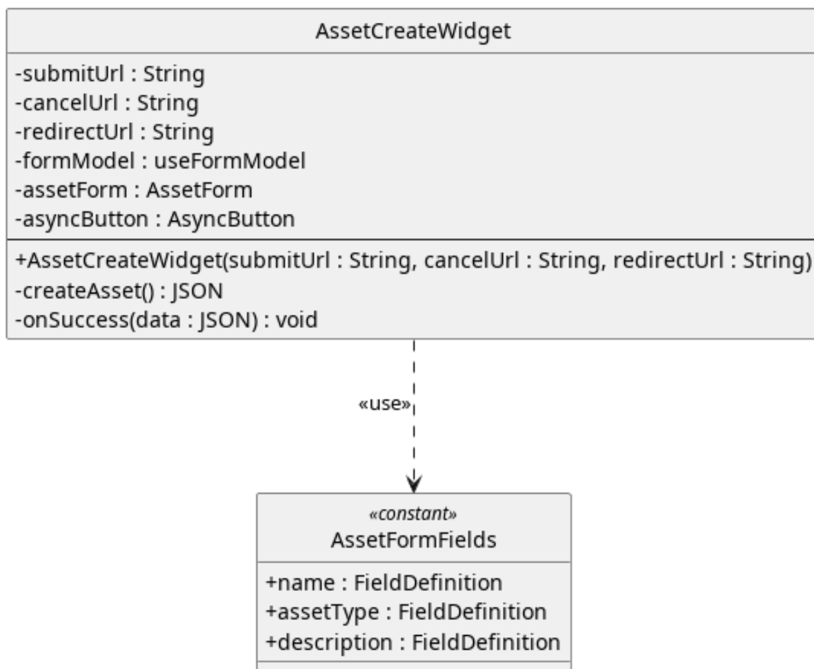
Figura 171: Widget - AssetCreateWidget
