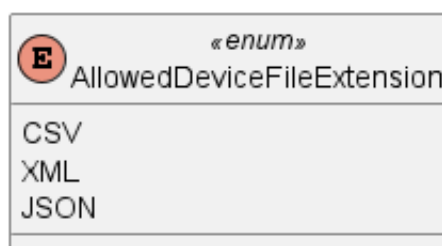
Figura 108: AllowedDeviceFileExtension
