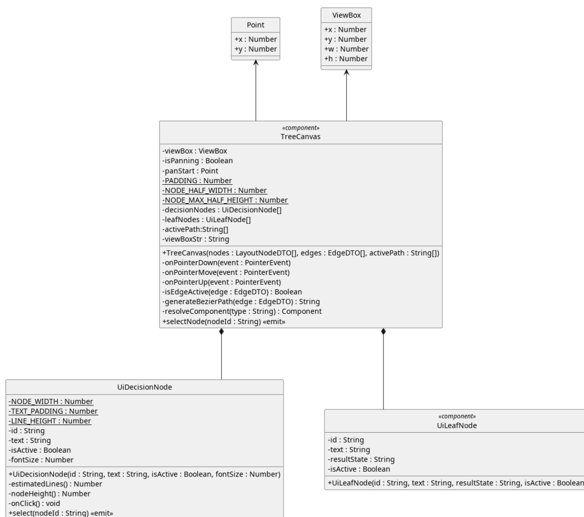
Figura 214: TreeCanvas
