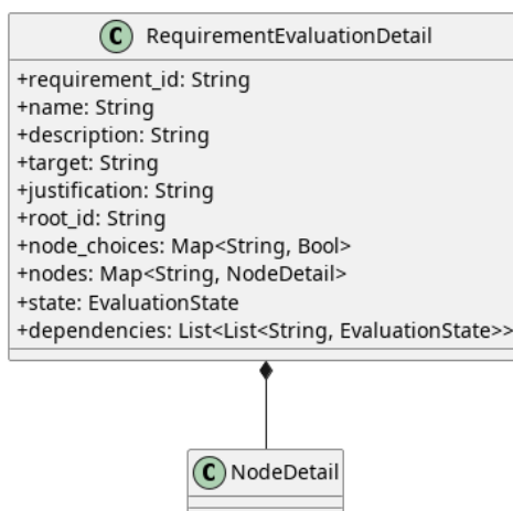
Figura 24: RequirementEvaluationDetail
