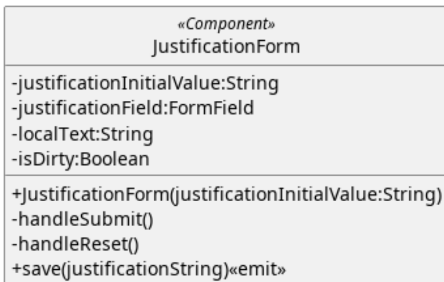
Figura 216: JustificationForm
