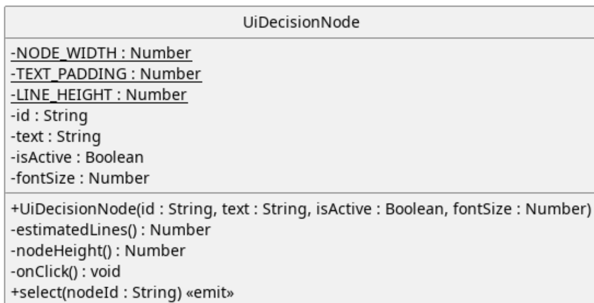
Figura 219: UiDecisionNode
