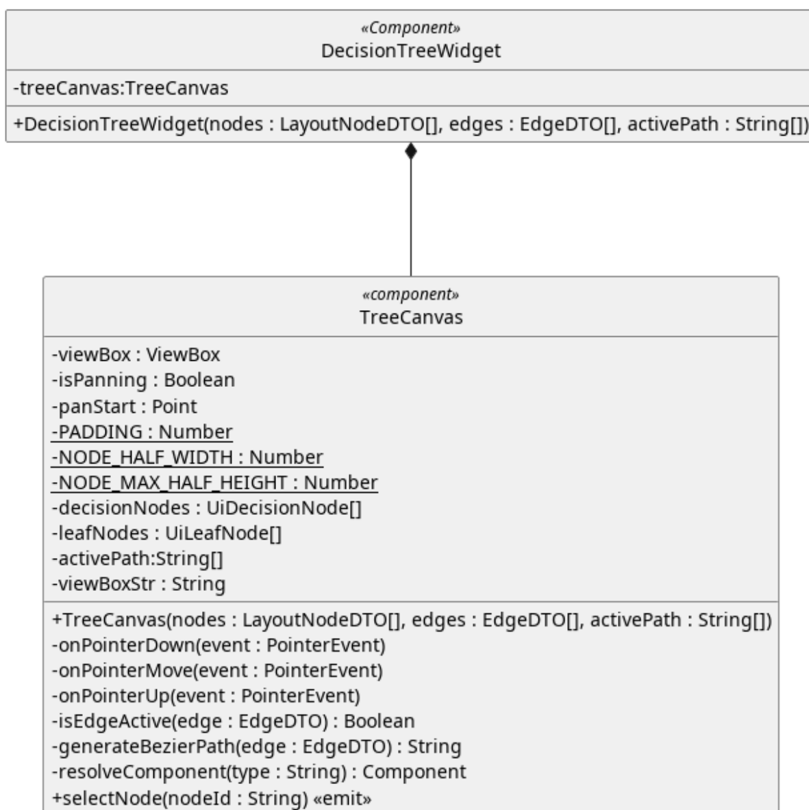
Figura 213: DecisionTreeWidget
