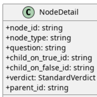
Figura 23: NodeDetail
