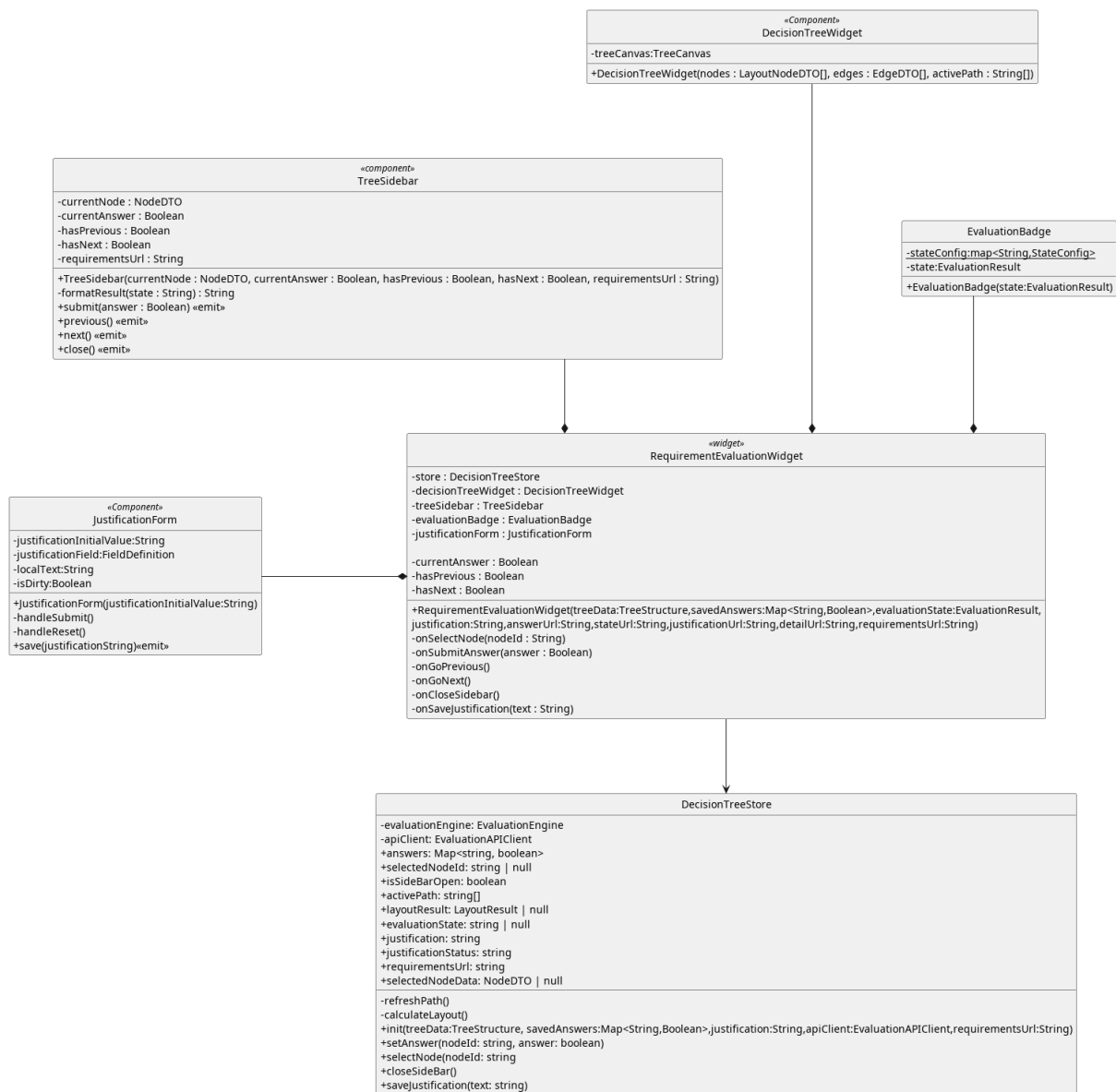
Figura 210: RequirementEvaluationWidget
