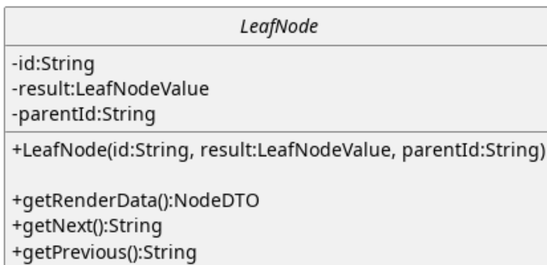
Figura 195: LeafNode
