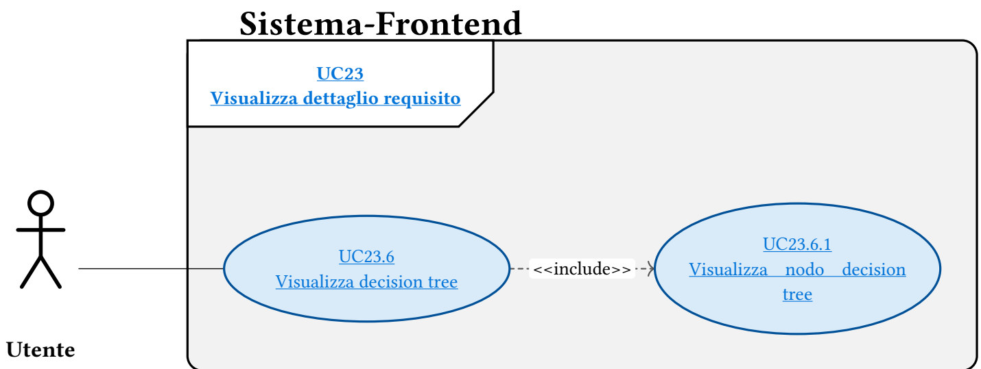
Figura 36: UC23.6 - Visualizza decision tree
