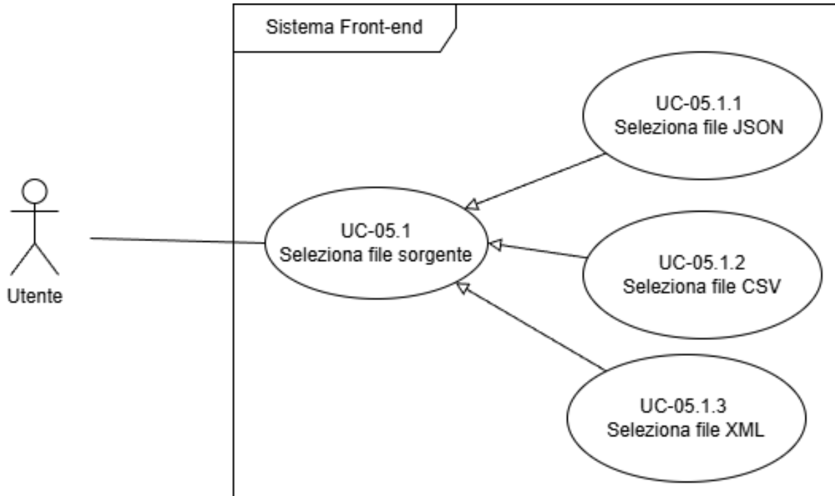
Figure 6: UC05.1
