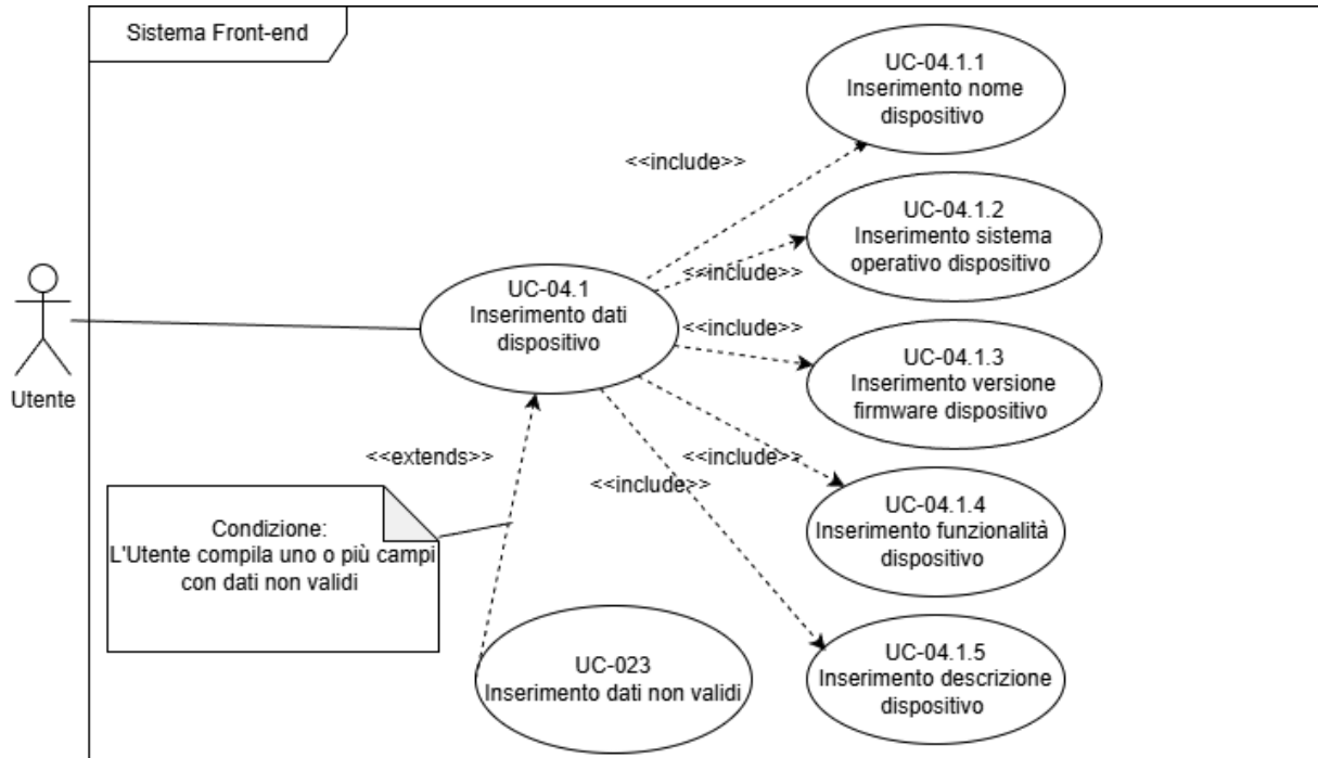
Figure 4: UC04.1
