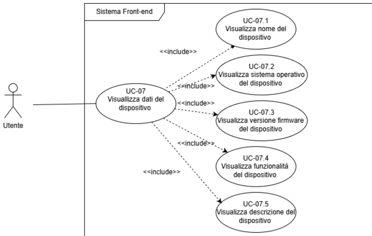
Figure 7: UC07
