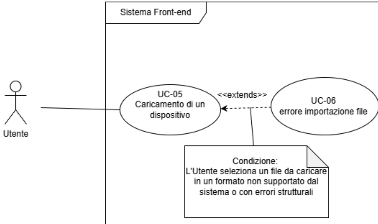
Figure 5: UC05
