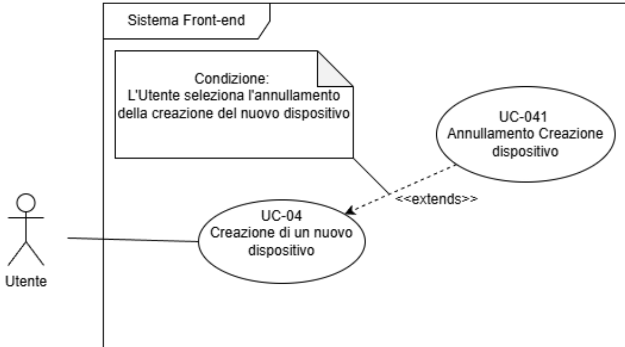
Figure 3: UC04
