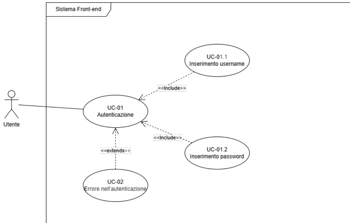
Figure 1: UC01
