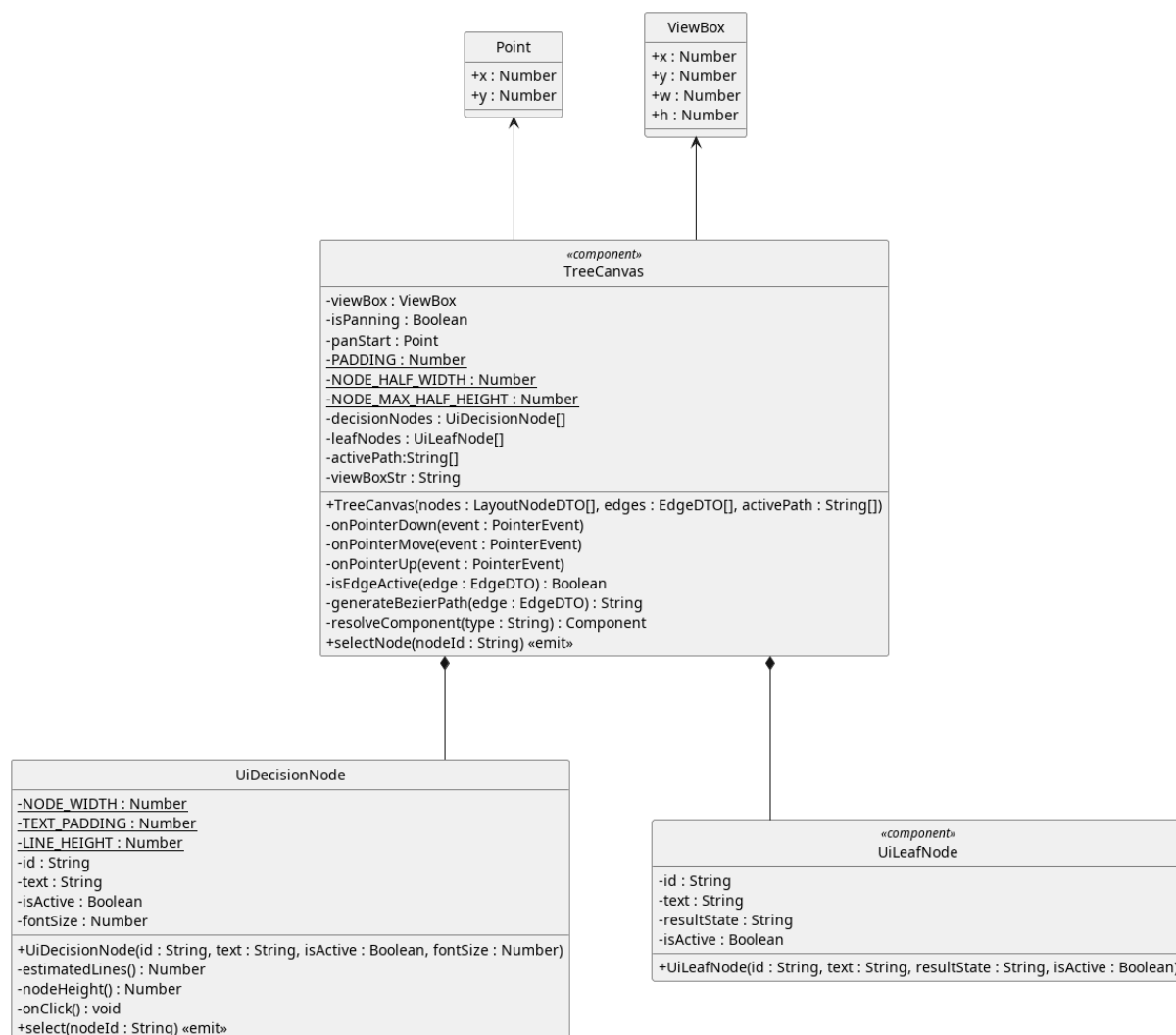
Figura 215: TreeCanvas
