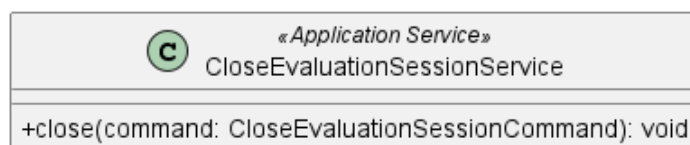
Figura 147: CloseEvaluationSessionService
