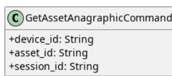
Figura 89: GetAssetAnagraphicCommand
