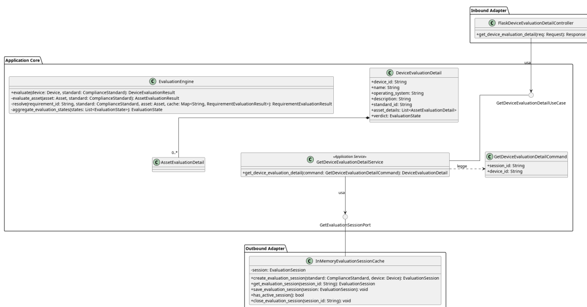
Figura 65: GetDeviceEvaluationDetail
