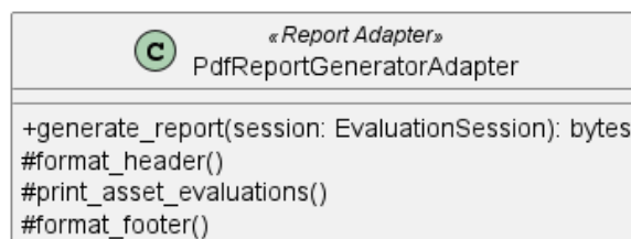
Figura 154: PdfReportGeneratorAdapter
