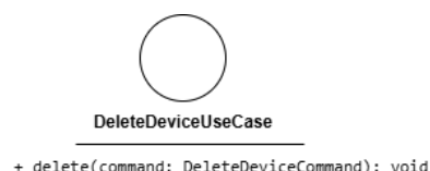
Figura 13: DeleteDeviceUseCase
