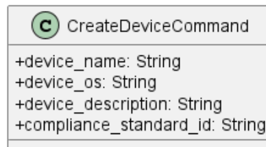
Figura 7: CreateDeviceCommand
