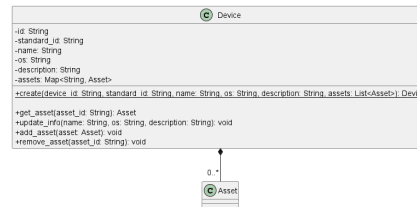
Figura 9: Device
