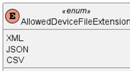
Figura 140: AllowedDeviceFileExtension
