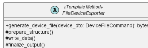
Figura 144: FileDeviceExporter
