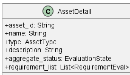
Figura 58: AssetDetail
