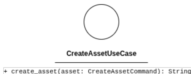
Figura 73: CreateAssetUseCase
