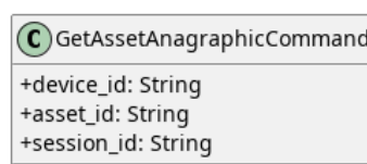
Figura 88: GetAssetAnagraphicCommand
