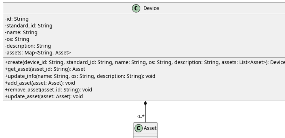
Figura 5: Device
