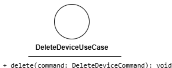
Figura 39: DeleteDeviceUseCase
