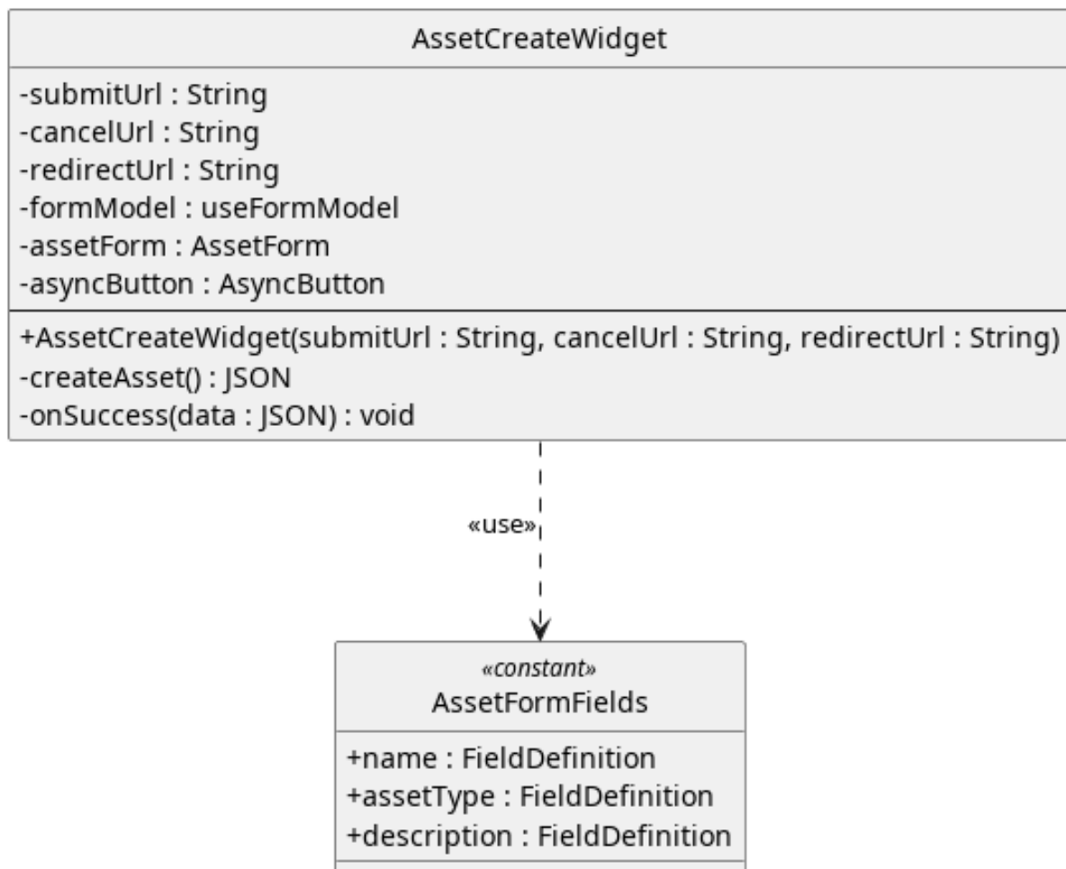
Figura 172: Widget - AssetCreateWidget
