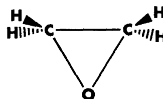
ethylene oxide
