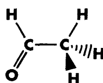
acetaldehyde
