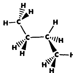
anticlinal isomer
