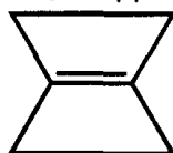
bicyclo[2.2.0]hex-1(4)-ene ( \text{C}_6\text{H}_8 )
