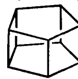
pentaprismane ( \text{C}_{10}\text{H}_{10} )
