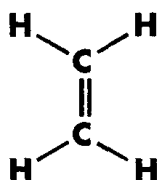
ethylene
