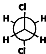
trans
