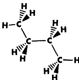
anti isomer
