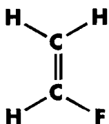
fluoroethylene
