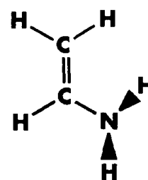
minimum
