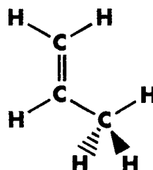
propene
