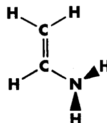
vinyl amine
