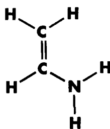
transition state
