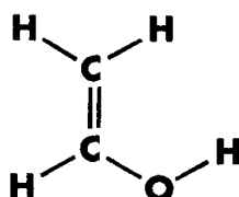
vinyl alcohol
