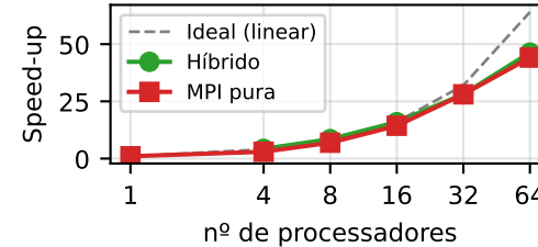
(a) Speed-up (forte)
