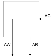
Figure D6-3 Required non-blocking transaction channel ordering
