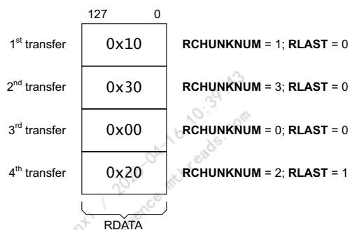
Figure E1-8 Example of a wrapping burst
