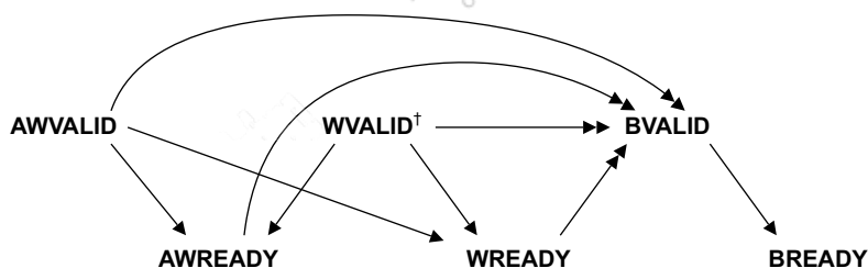
Figure A3-7 AXI4 and AXI5 write transaction handshake dependencies
