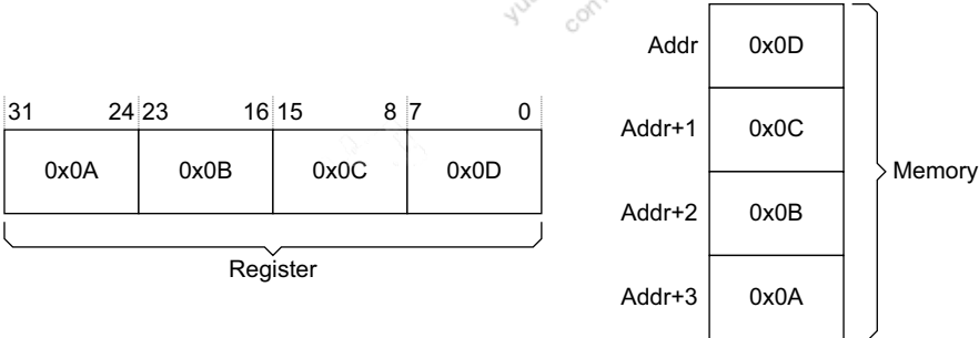
Figure A3-11 Example little-endian byte-invariant data structure
