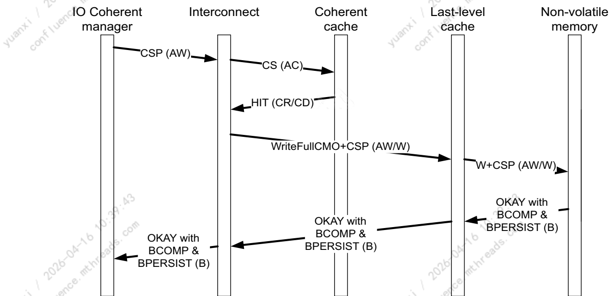
Figure D7-2 Example write with CMO
