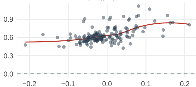
Newman vs FNIH
