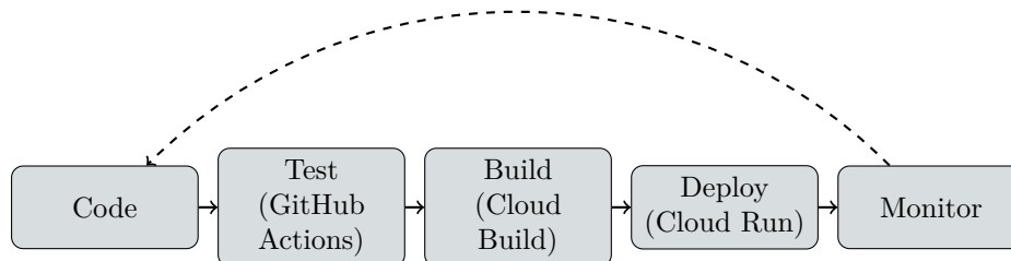
Figura 9: Pipeline CI/CD do FocusQuest
