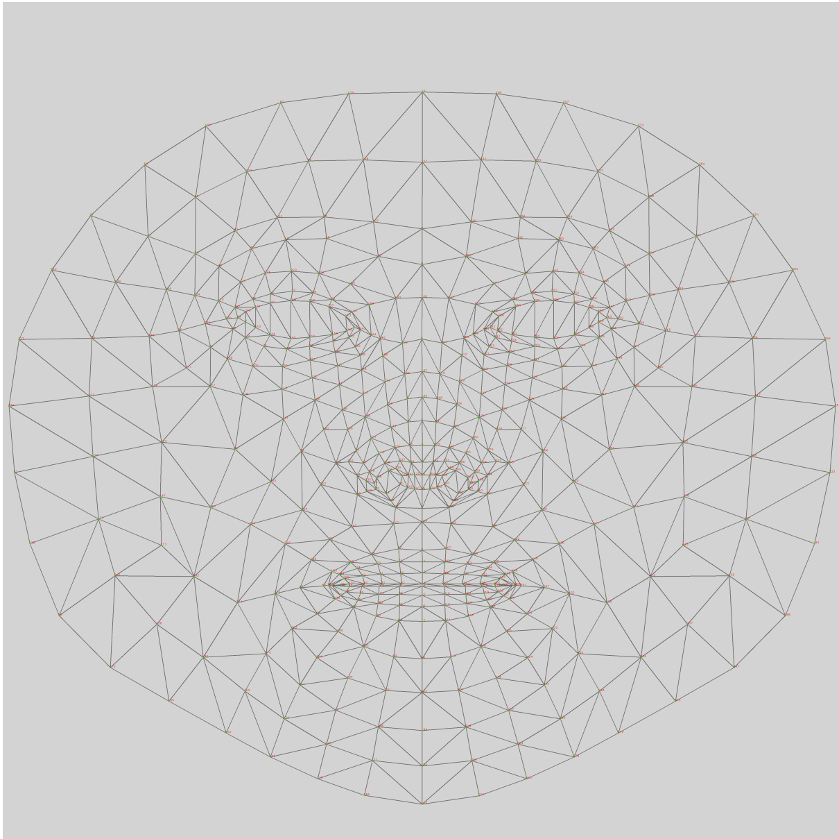
Figura 1: TensorFlow FaceMesh
