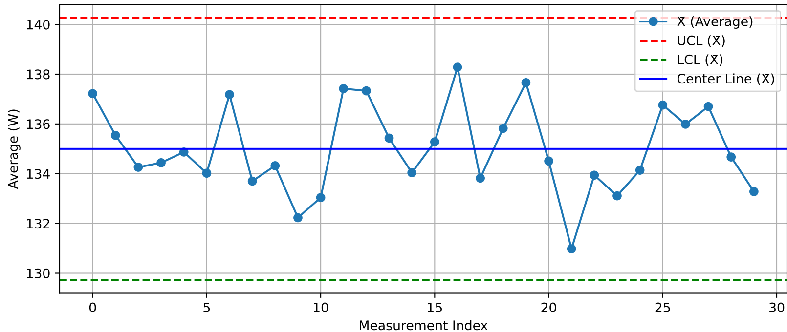
DUT - \bar{X} Chart (T32_Test1_Xint@Test.xlsx)
