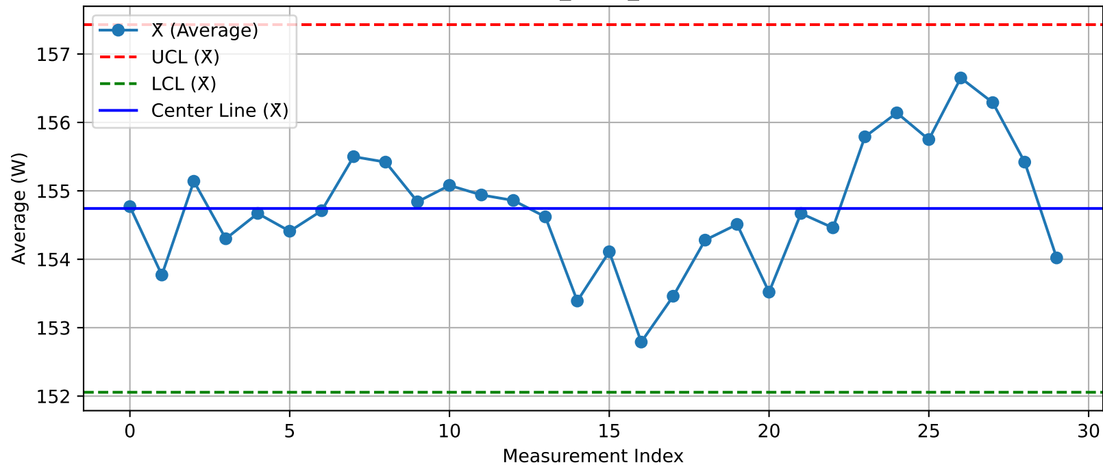
DUT - \bar{X} Chart (T49_Test2_Nuitka@Test.xlsx)
