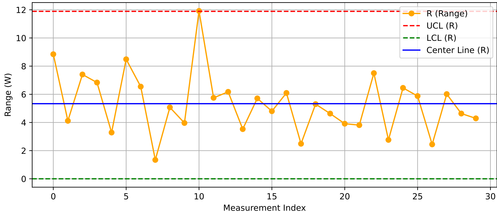
DUT - R Chart (T7_Test1@Test.xlsx)
