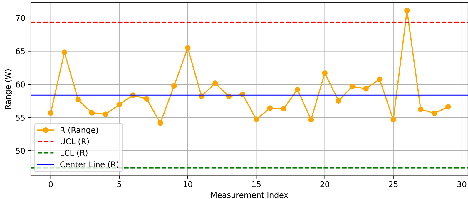
DUT - R Chart (T49_Test1@Test.xlsx)
