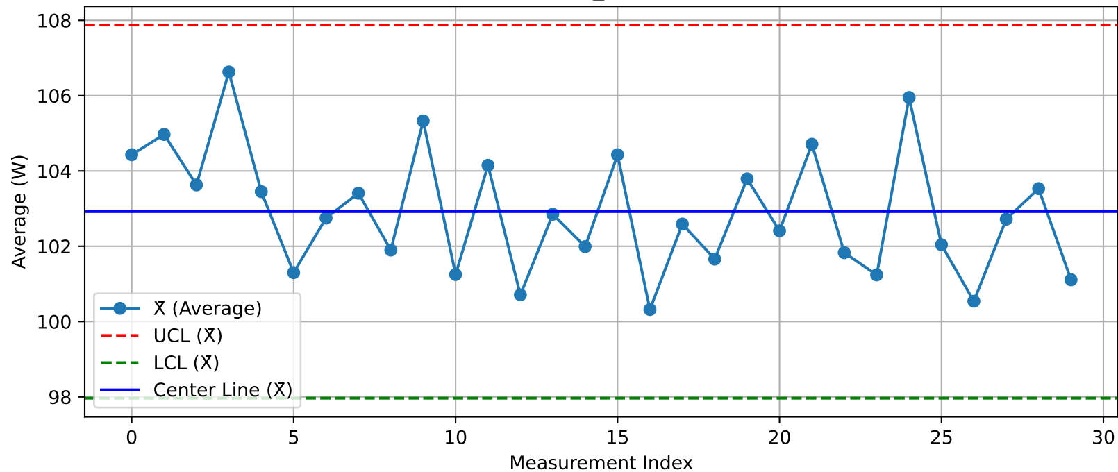
DUT - \bar{X} Chart (T10_Test200@Test.xlsx)
