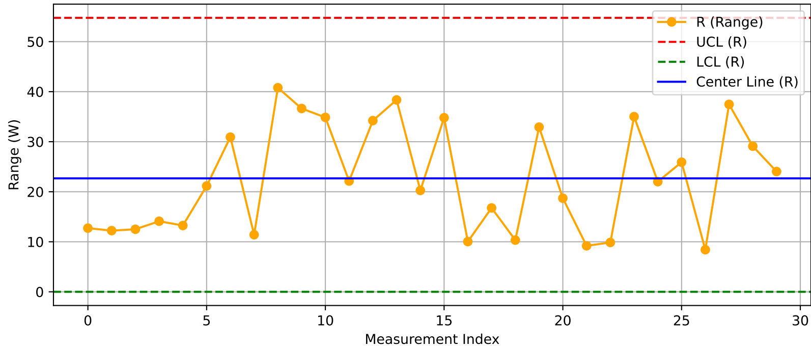
DUT - R Chart (T7_Test2@Test.xlsx)
