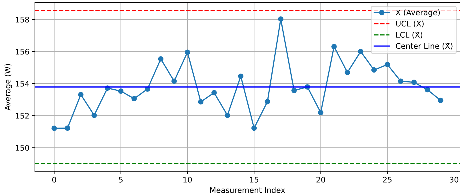
DUT - \bar{X} Chart (T29_Test1@Test.xlsx)
