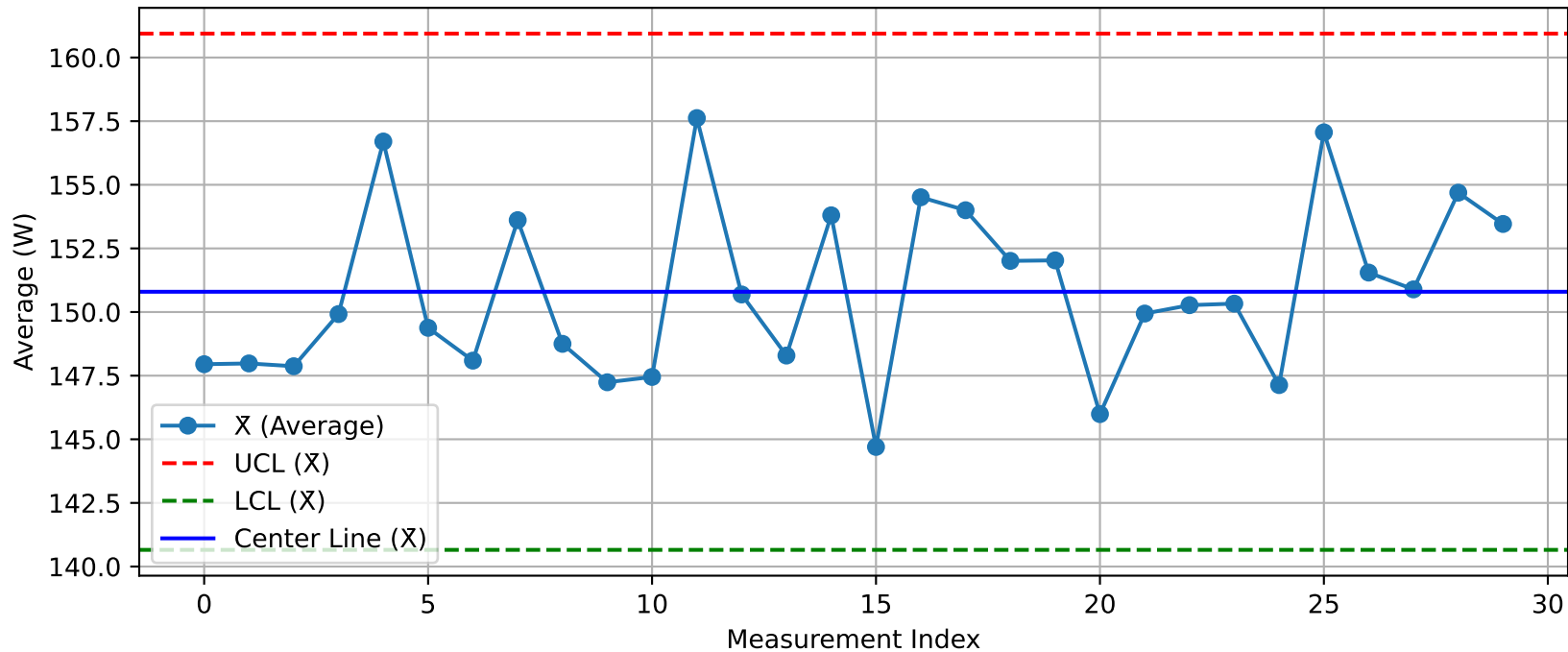
DUT - \bar{X} Chart (T44_Test2_Nuitka@Test.xlsx)
