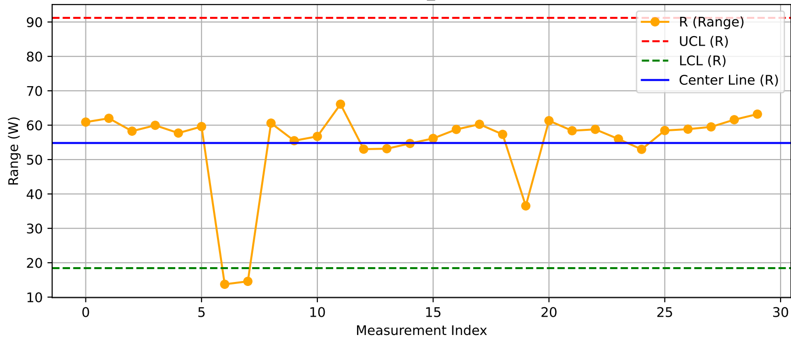
DUT - R Chart (T40_Test1@Test.xlsx)
