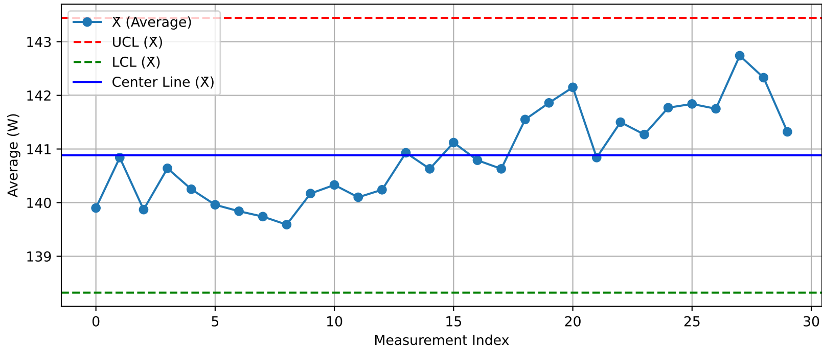
DUT - \bar{X} Chart (T4_Test2@Test.xlsx)
