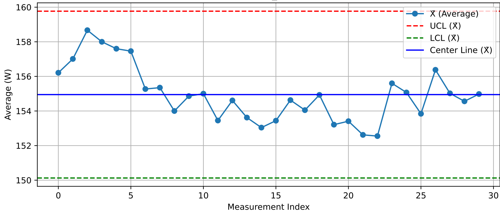
DUT - \bar{X} Chart (T17_Test2@Test.xlsx)
