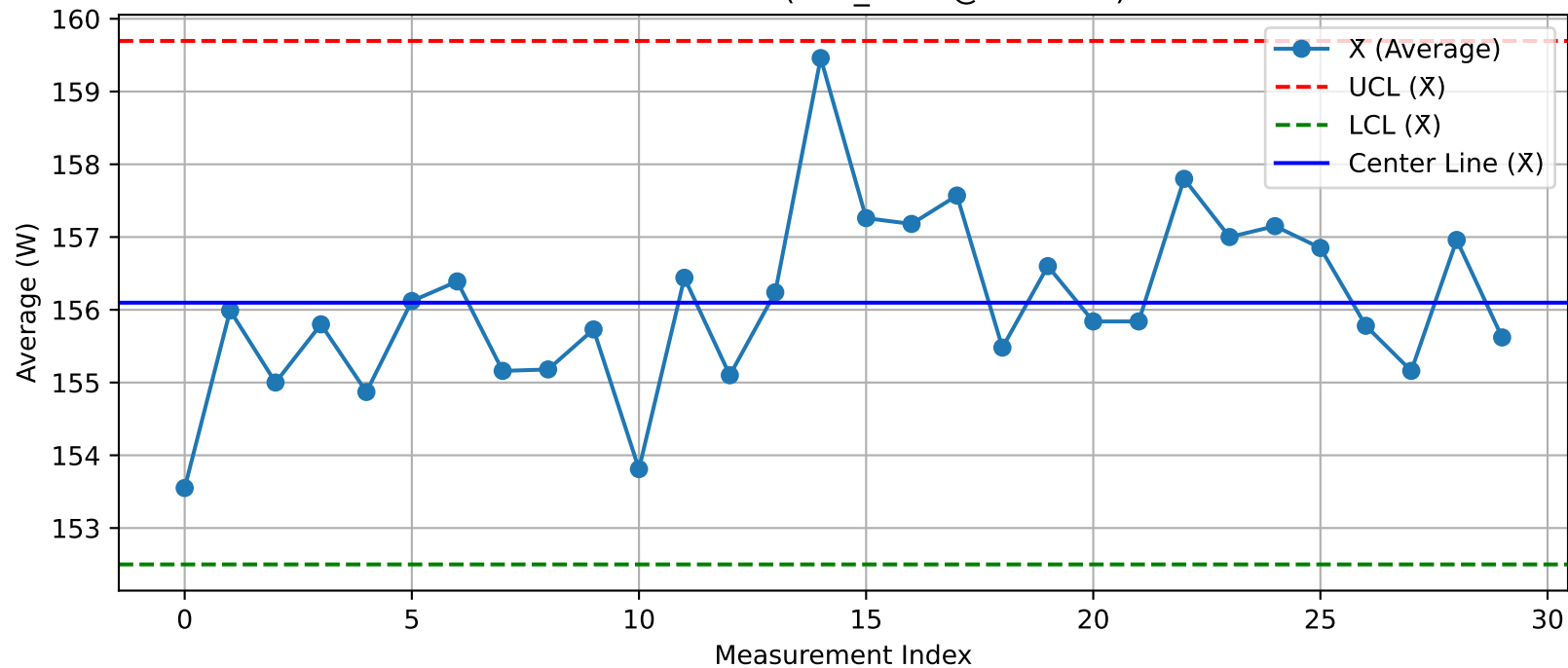
DUT - \bar{X} Chart (T20_Test1@Test.xlsx)
