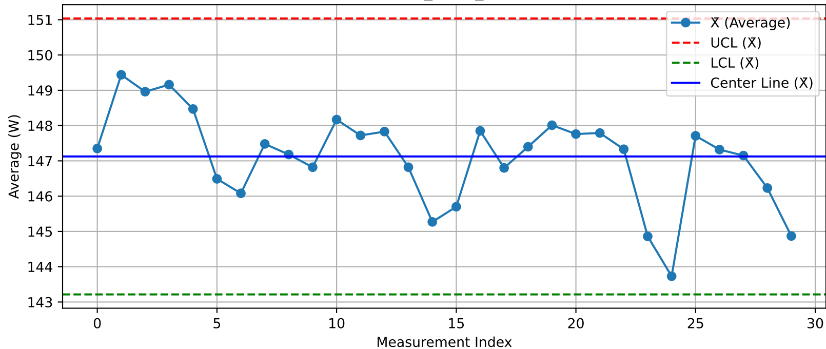
DUT - \bar{X} Chart (T5_Test2_Xint@Test.xlsx)
