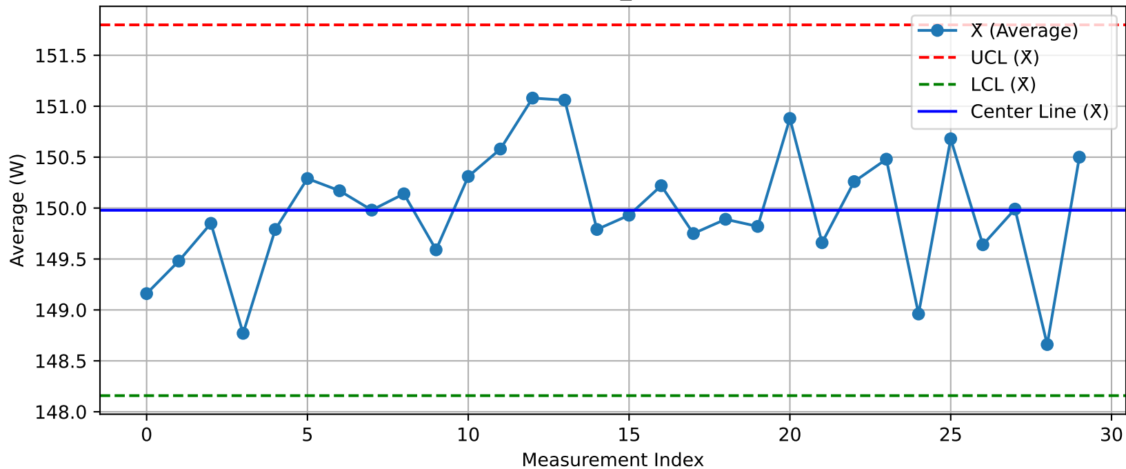
DUT - \bar{X} Chart (T49_Test1@Test.xlsx)
