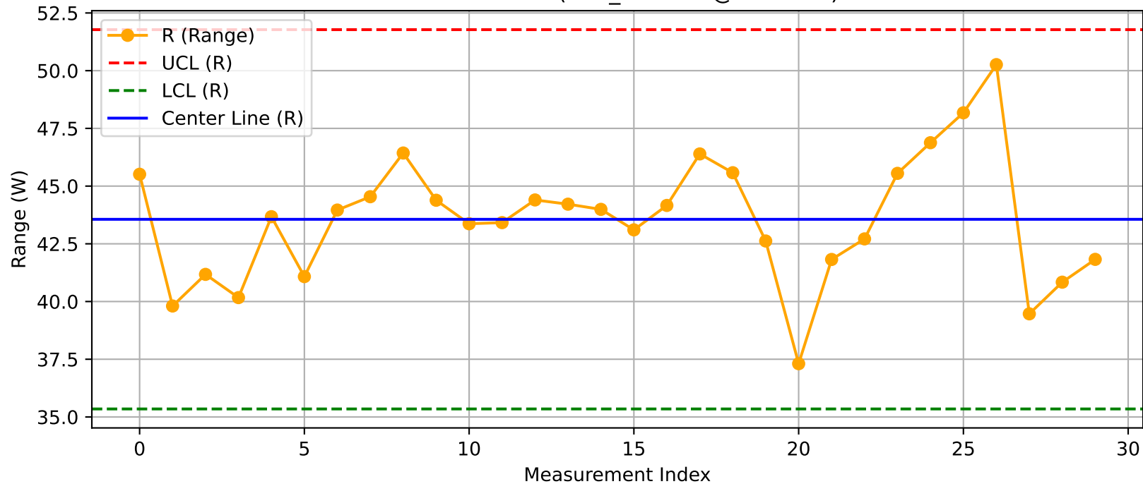
DUT - R Chart (T36_Test100@Test.xlsx)
