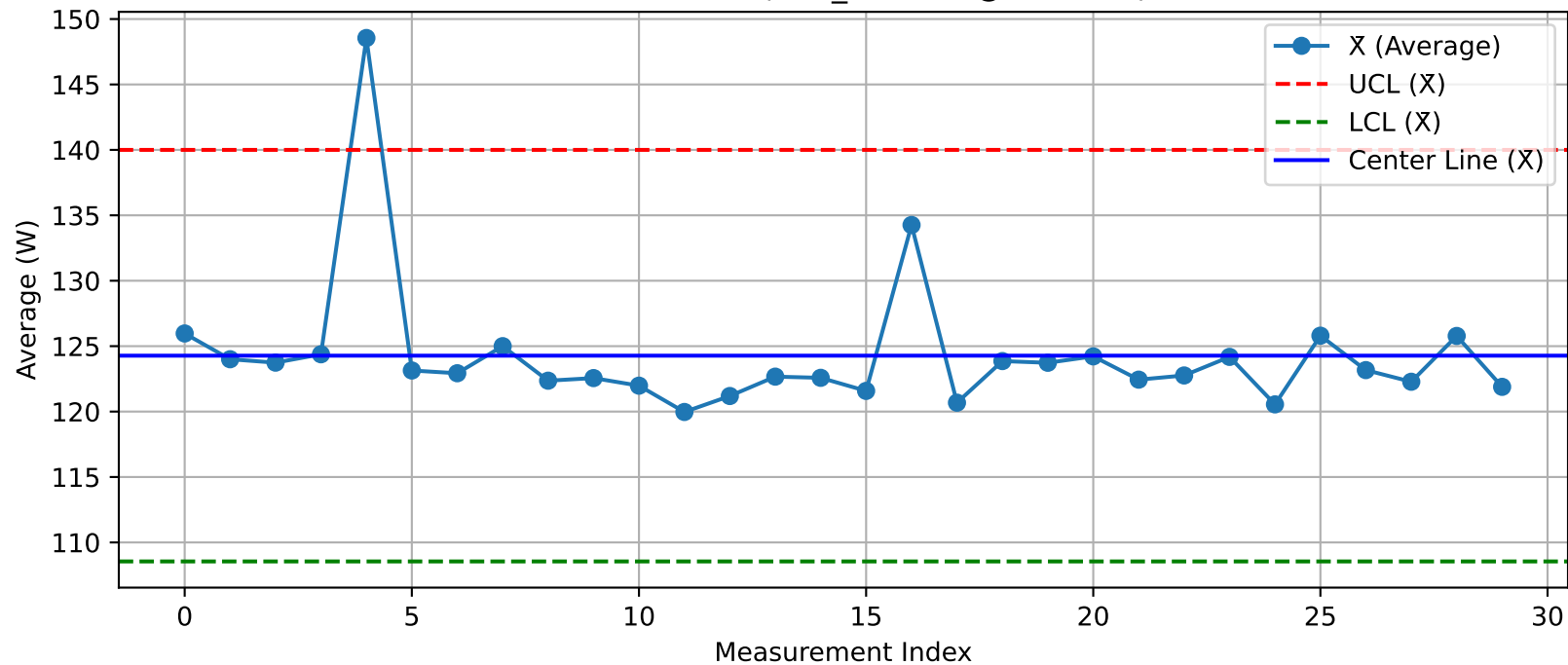
DUT - \bar{X} Chart (T19_Test203@Test.xlsx)
