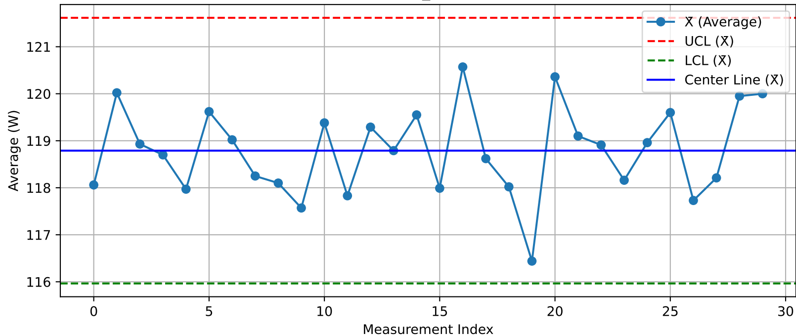
DUT - \bar{X} Chart (T07_Test103@Test.xlsx)
