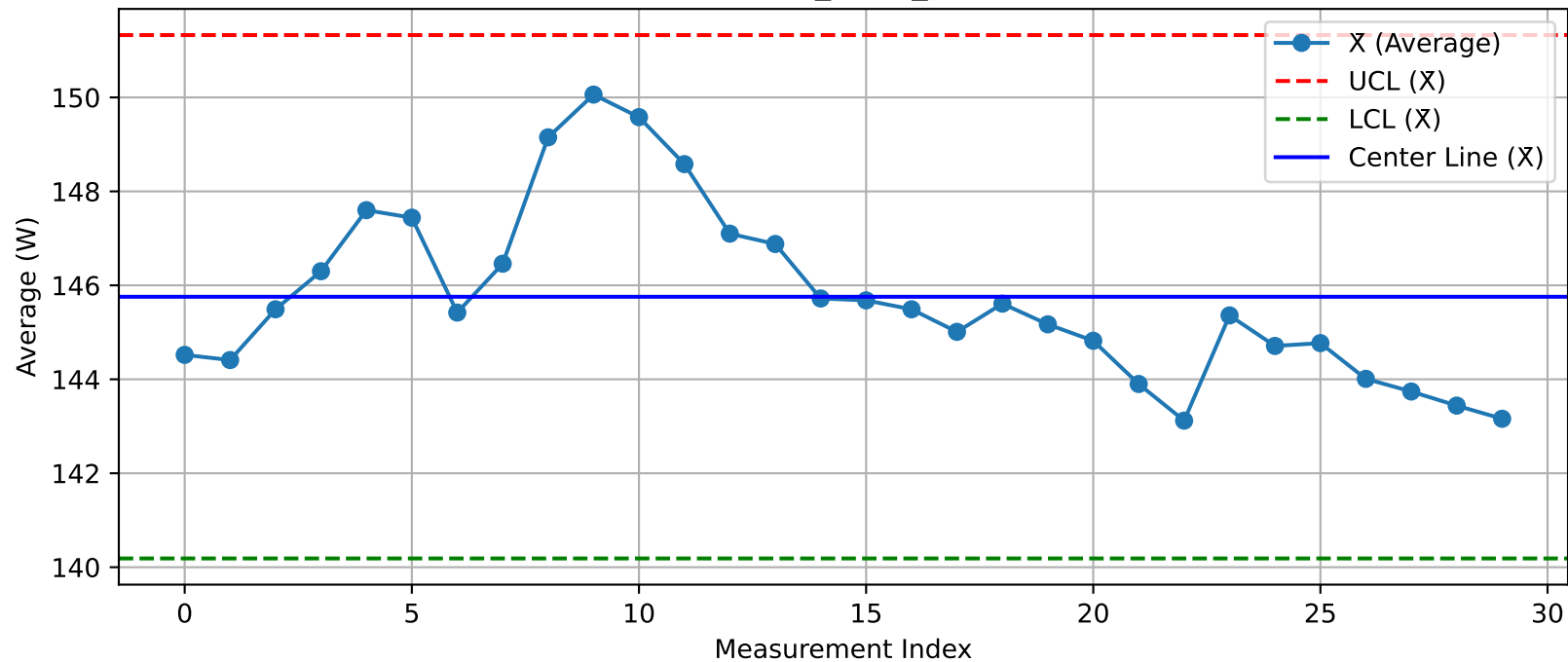
DUT - \bar{X} Chart (T51_Test1_Xint@Test.xlsx)
