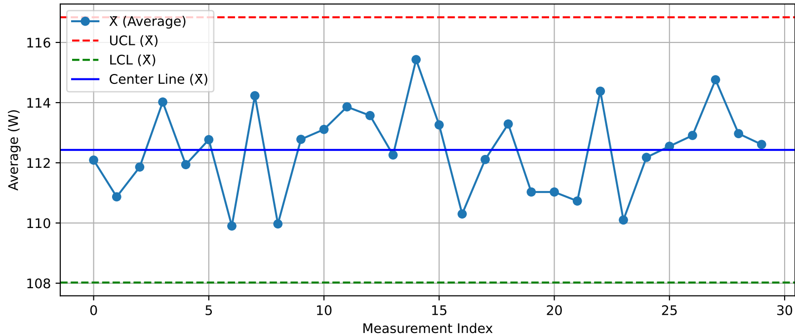
DUT - \bar{X} Chart (T04_Test2O3@Test.xlsx)
