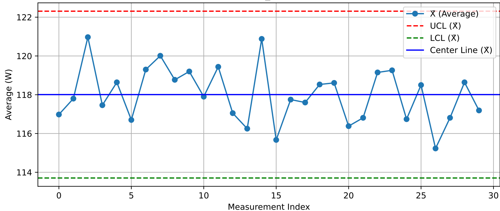
DUT - \bar{X} Chart (T07_Test100@Test.xlsx)
