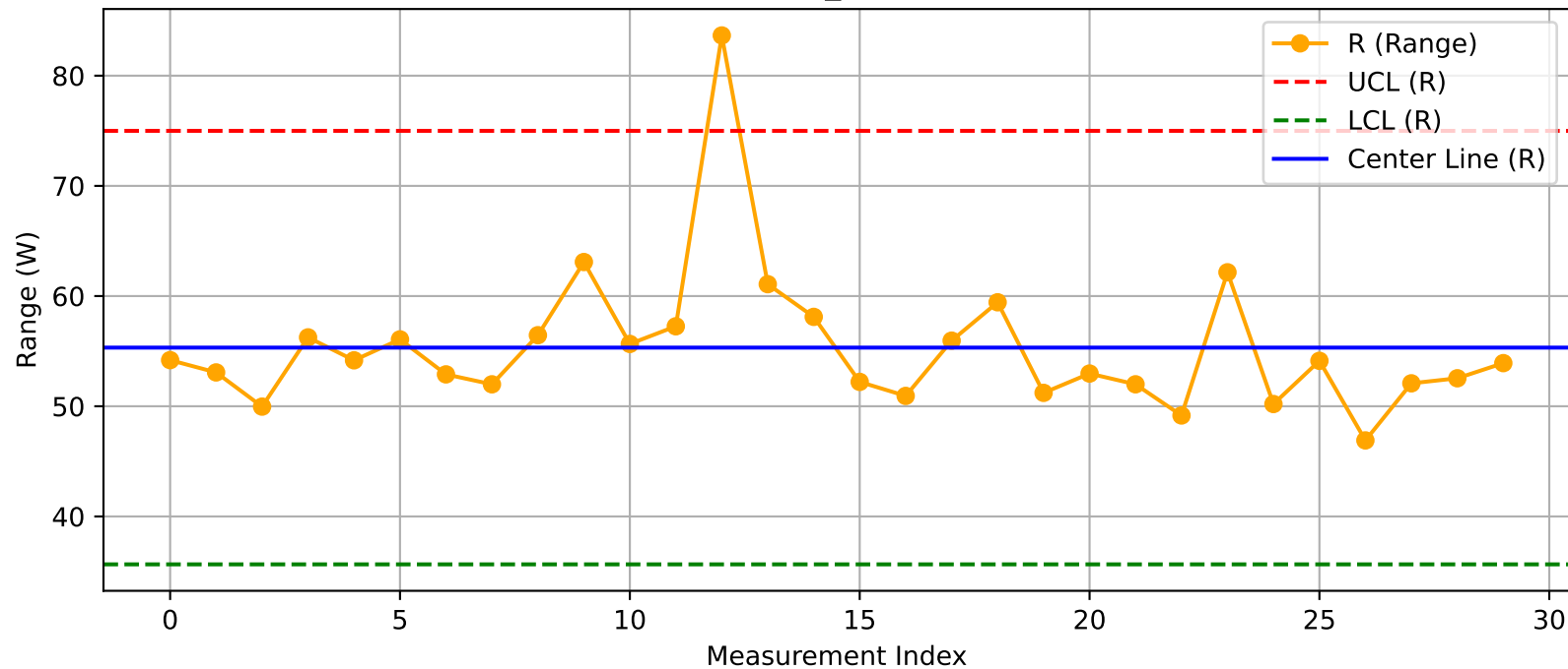
DUT - R Chart (T05_Test200@Test.xlsx)
