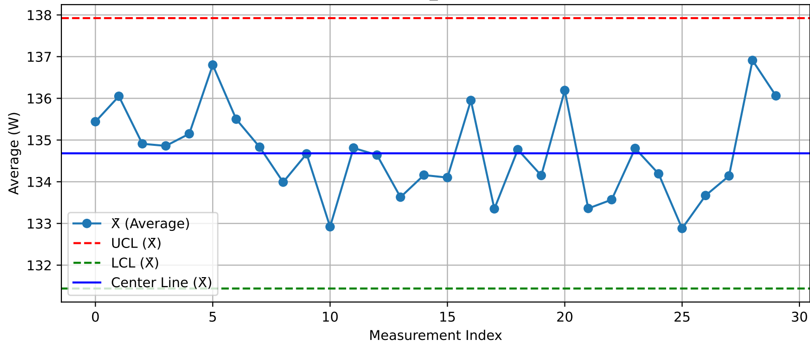
DUT - \bar{X} Chart (T08_Test2O3@Test.xlsx)
