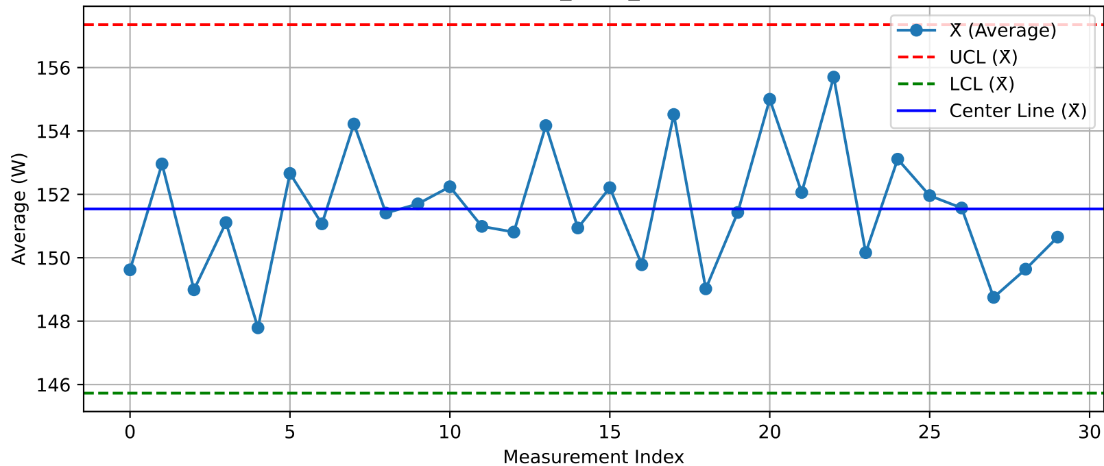
DUT - \bar{X} Chart (T32_Test2_Nuitka@Test.xlsx)
