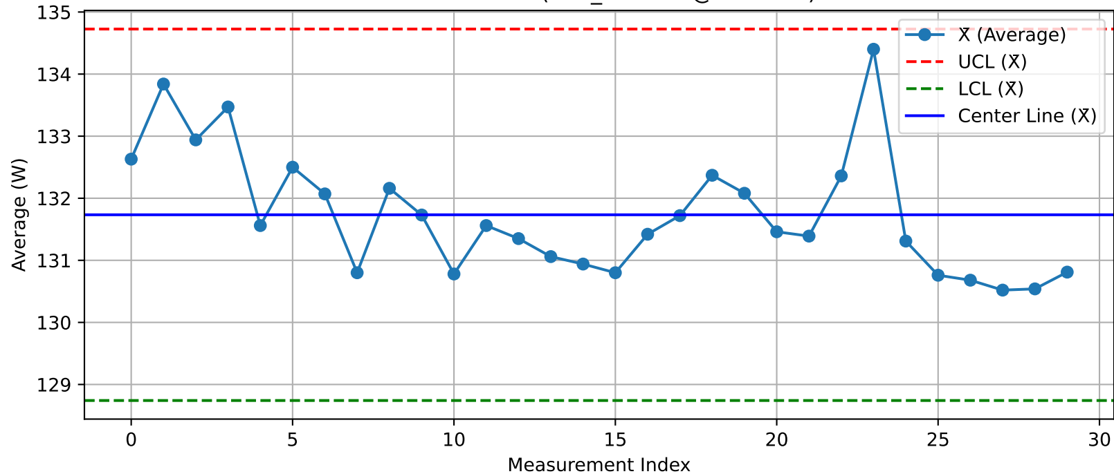
DUT - \bar{X} Chart (T25_Test203@Test.xlsx)
