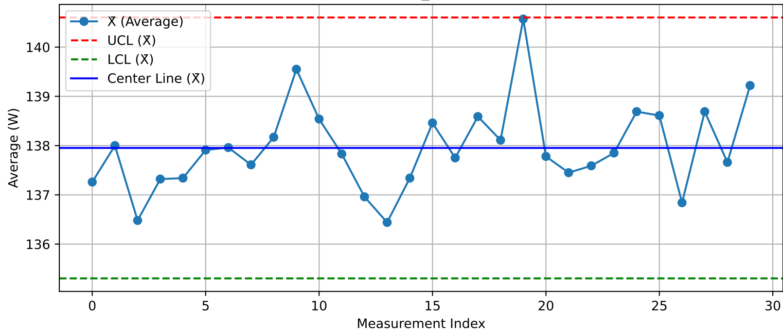
DUT - \bar{X} Chart (T8_Test2@Test.xlsx)
