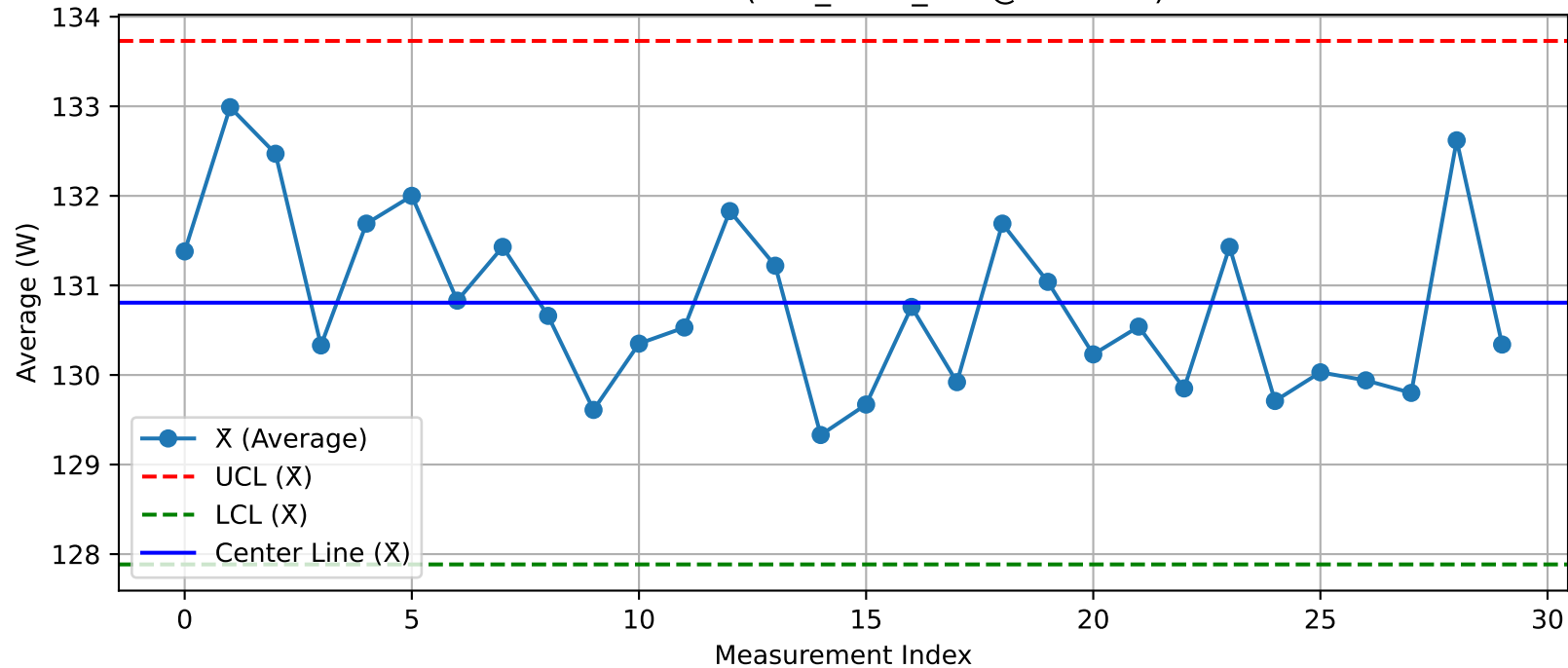
DUT - \bar{X} Chart (T17_Test2_Xint@Test.xlsx)
