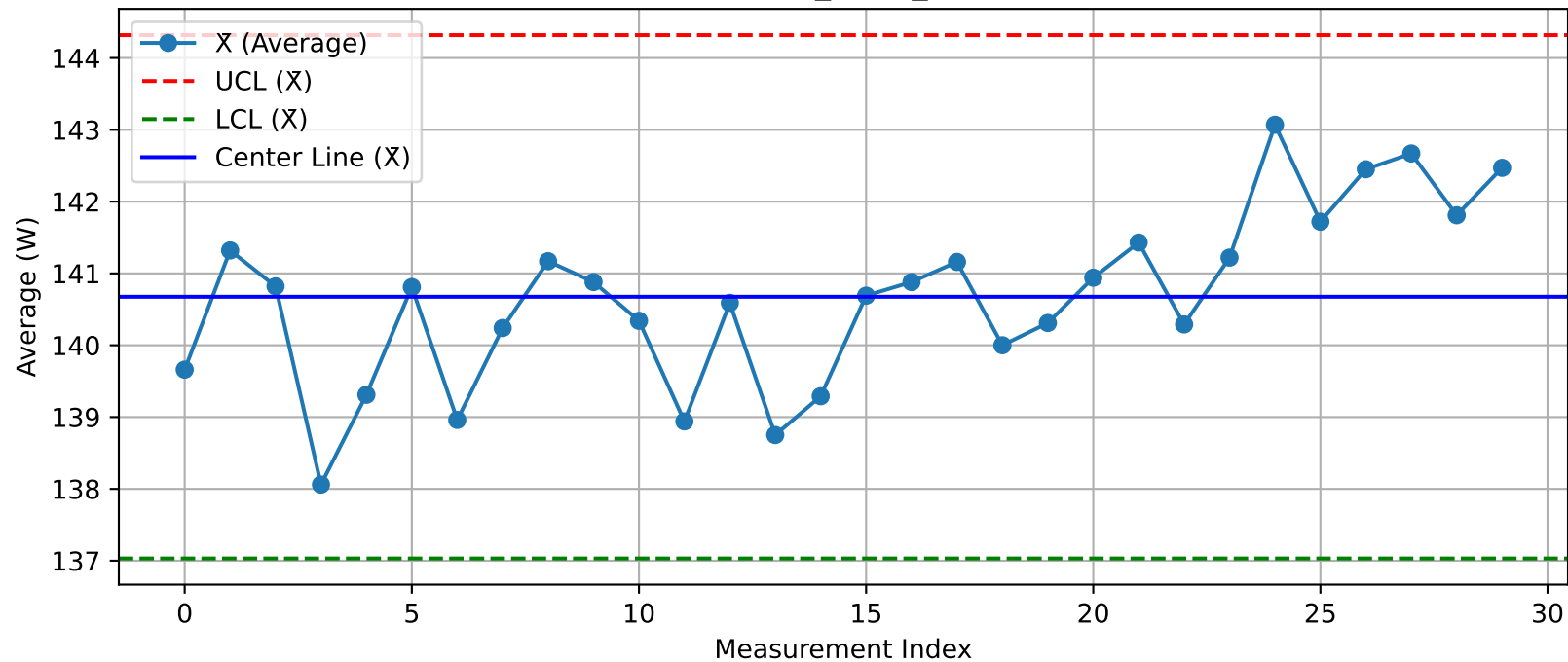
DUT - \bar{X} Chart (T31_Test1_Xint@Test.xlsx)
