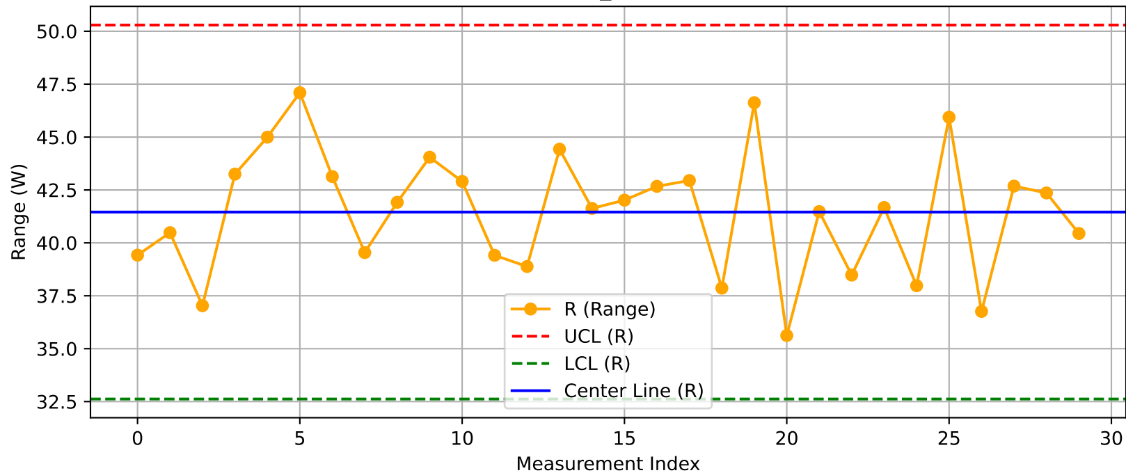
DUT - R Chart (T20_Test103@Test.xlsx)
