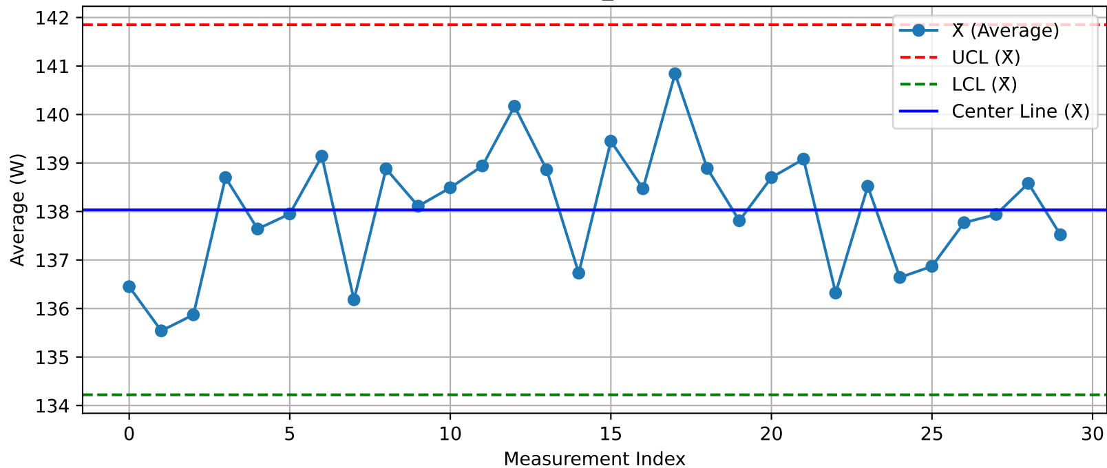
DUT - \bar{X} Chart (T12_Test1@Test.xlsx)
