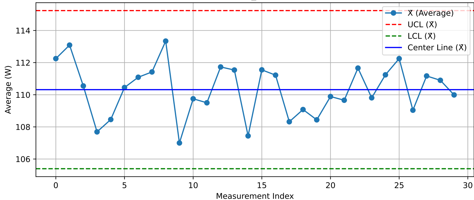
DUT - \bar{X} Chart (T16_Test203@Test.xlsx)
