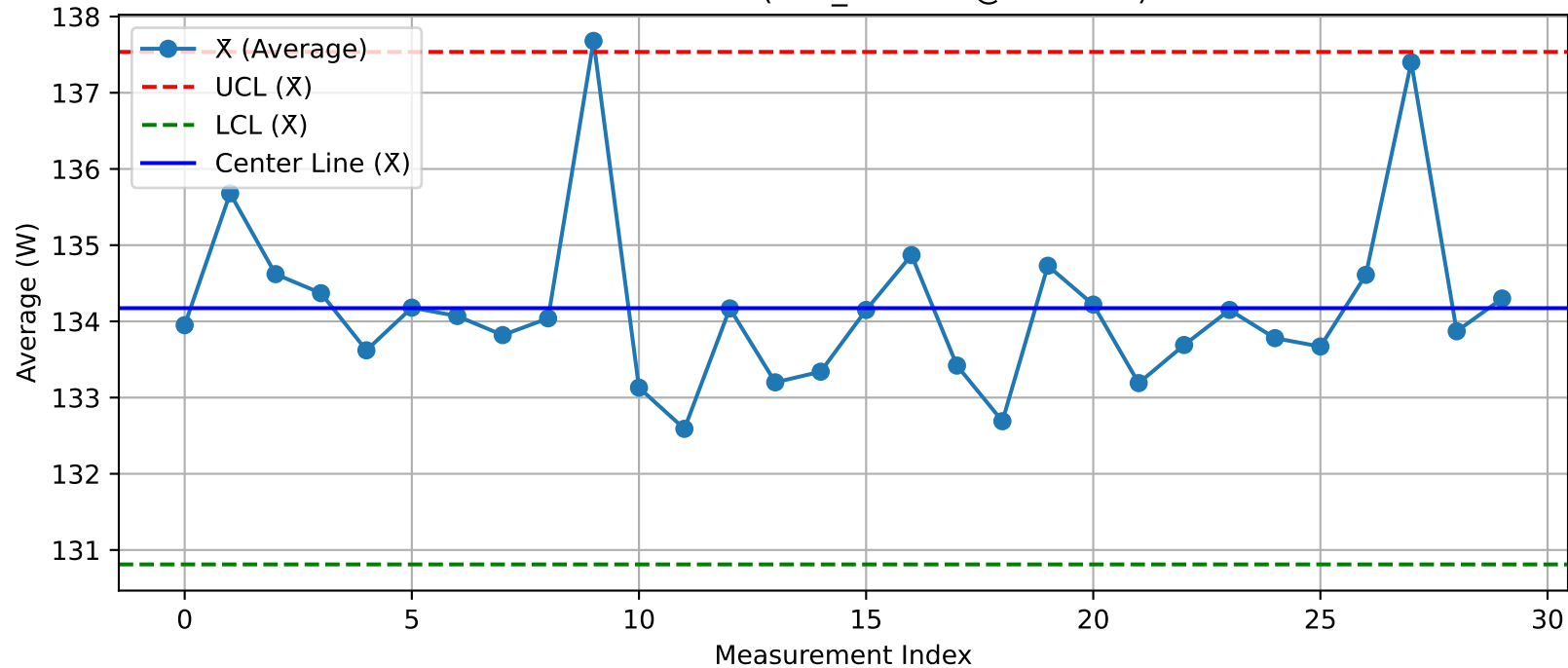
DUT - \bar{X} Chart (T13_Test203@Test.xlsx)
