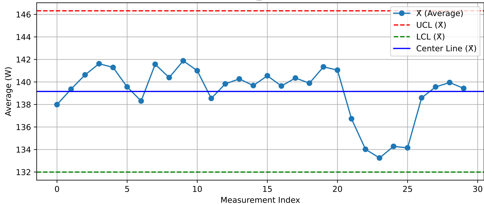
DUT - \bar{X} Chart (T28_Test100@Test.xlsx)
