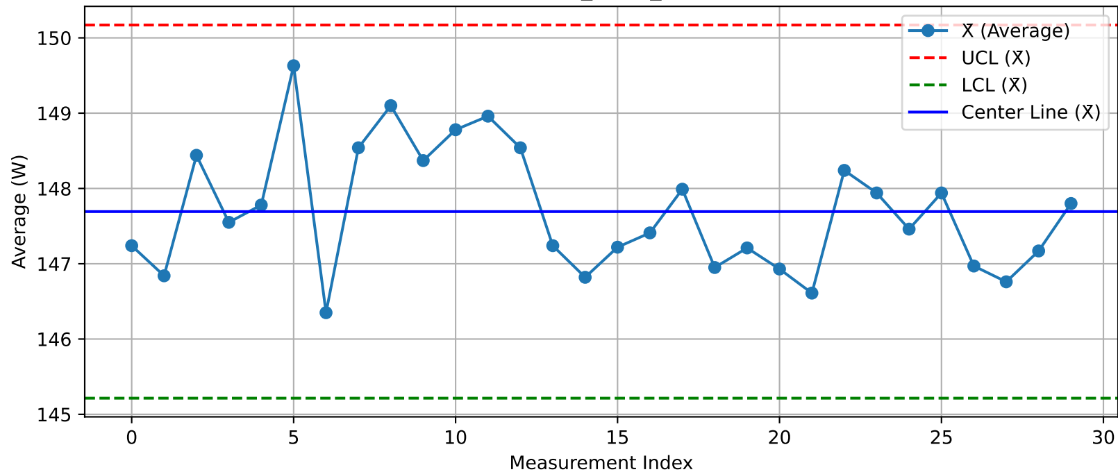
DUT - \bar{X} Chart (T50_Test2_Xint@Test.xlsx)
