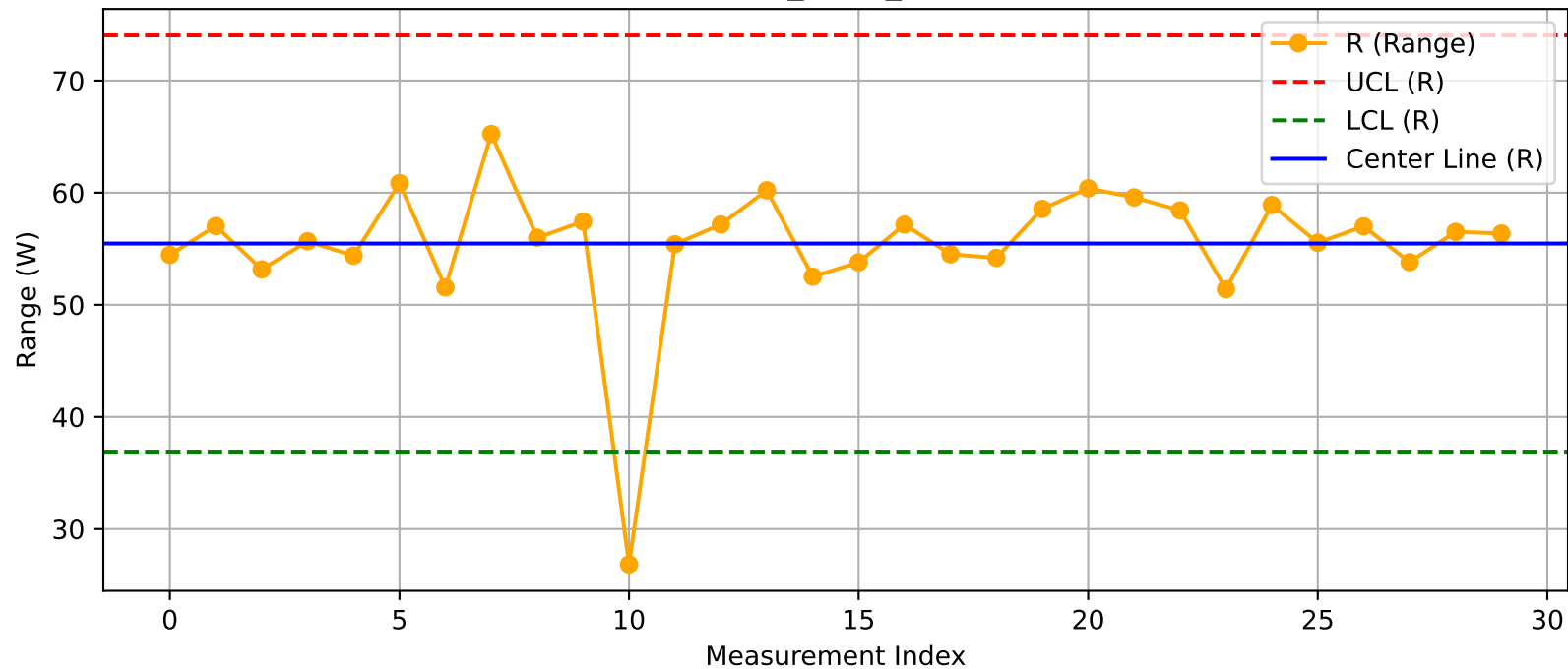
DUT - R Chart (T13_Test1_Nuitka@Test.xlsx)
