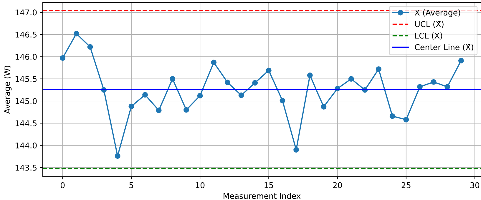
DUT - X Chart (T26_Test2_Xint@Test.xlsx)
