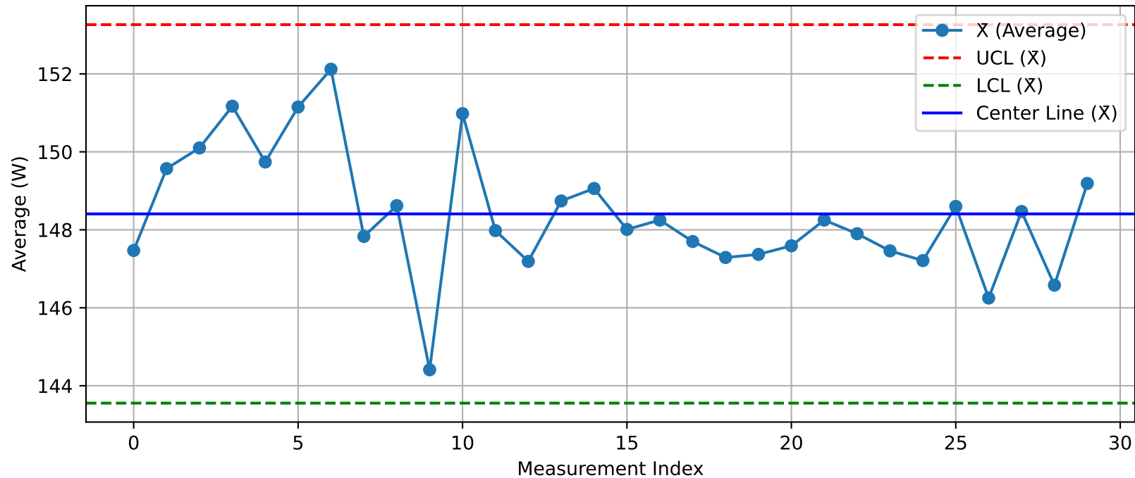
DUT - \bar{X} Chart (T50_Test2@Test.xlsx)
