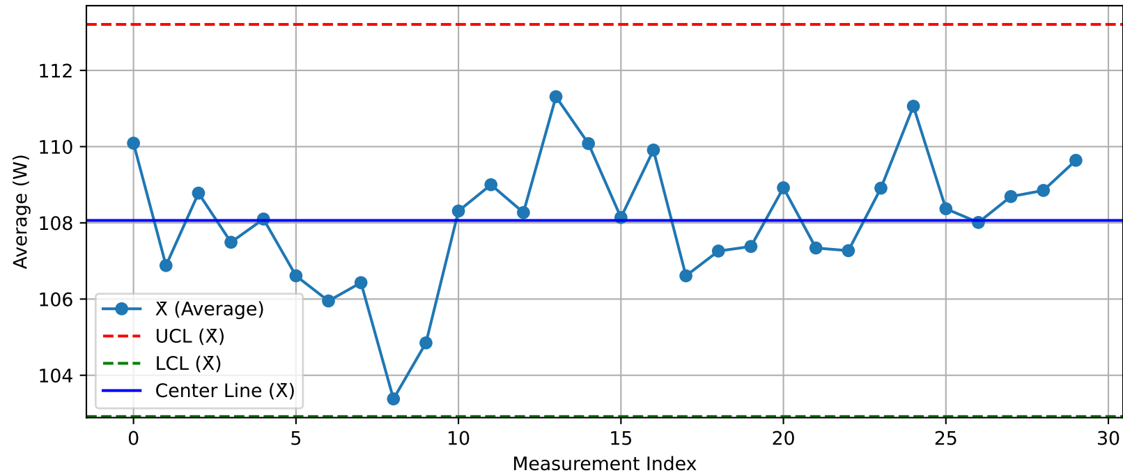
DUT - \bar{X} Chart (T33_Test203@Test.xlsx)
