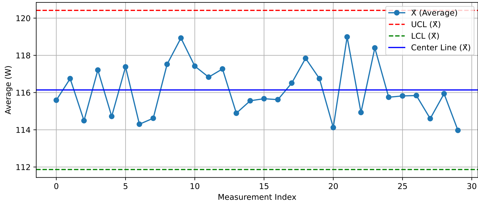
DUT - \bar{X} Chart (T07_Test2O3@Test.xlsx)
