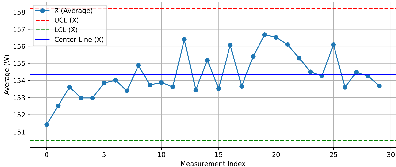
DUT - \bar{X} Chart (T31_Test100@Test.xlsx)
