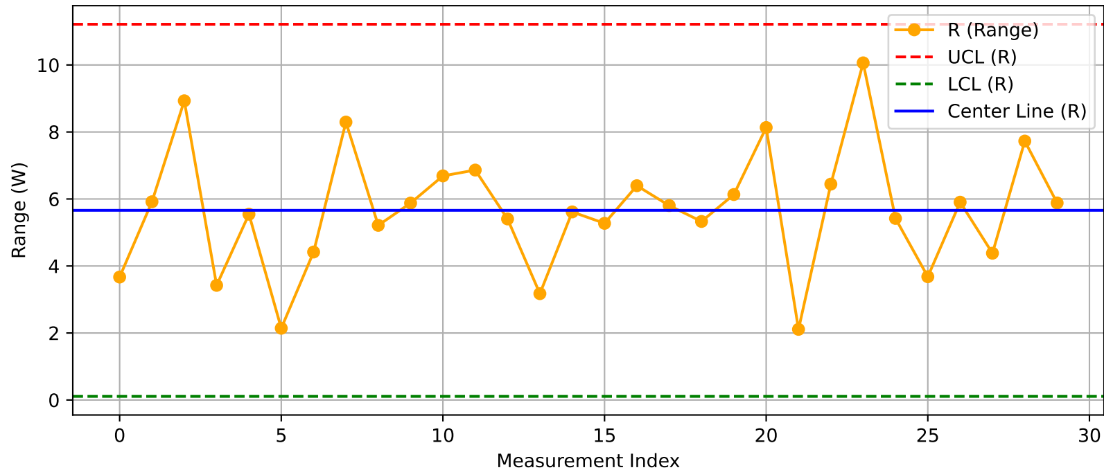
DUT - R Chart (T12_Test2@Test.xlsx)
