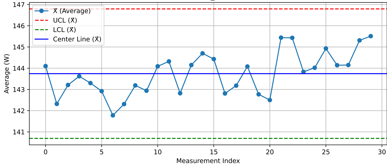
DUT - \bar{X} Chart (T26_Test2@Test.xlsx)
