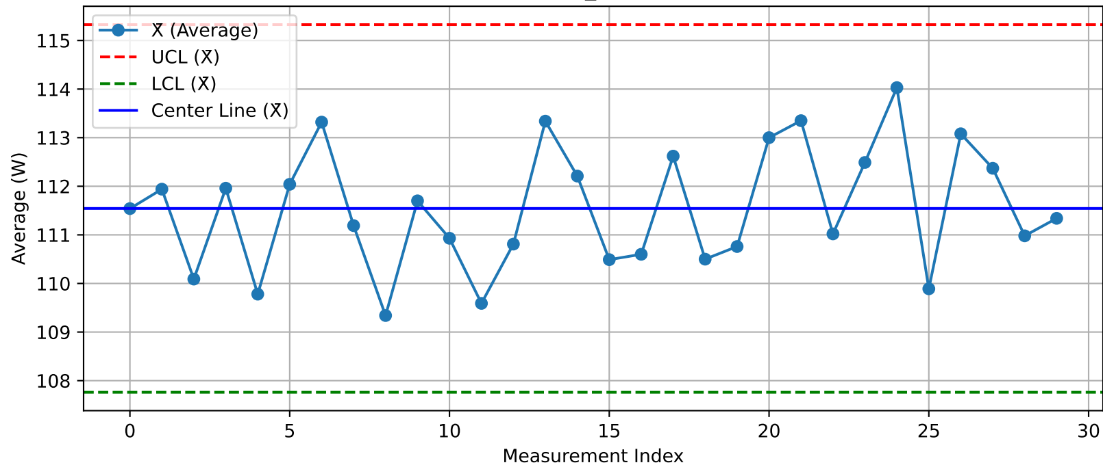
DUT - \bar{X} Chart (T33_Test100@Test.xlsx)
