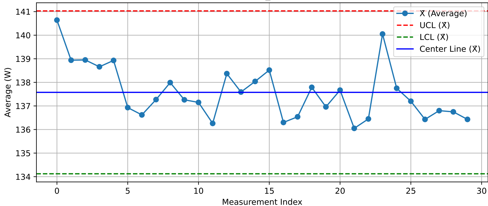
DUT - \bar{X} Chart (T10_Test2@Test.xlsx)
