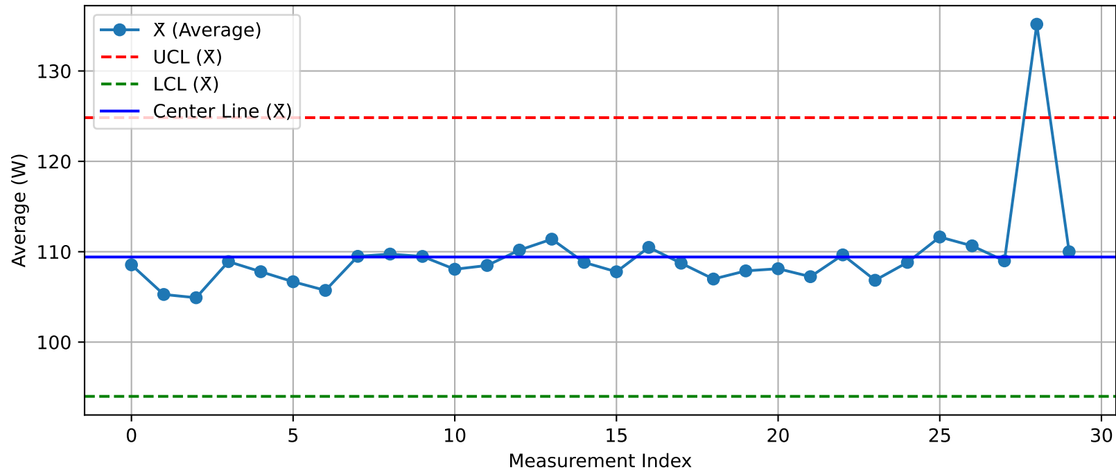
DUT - \bar{X} Chart (T09_Test100@Test.xlsx)
