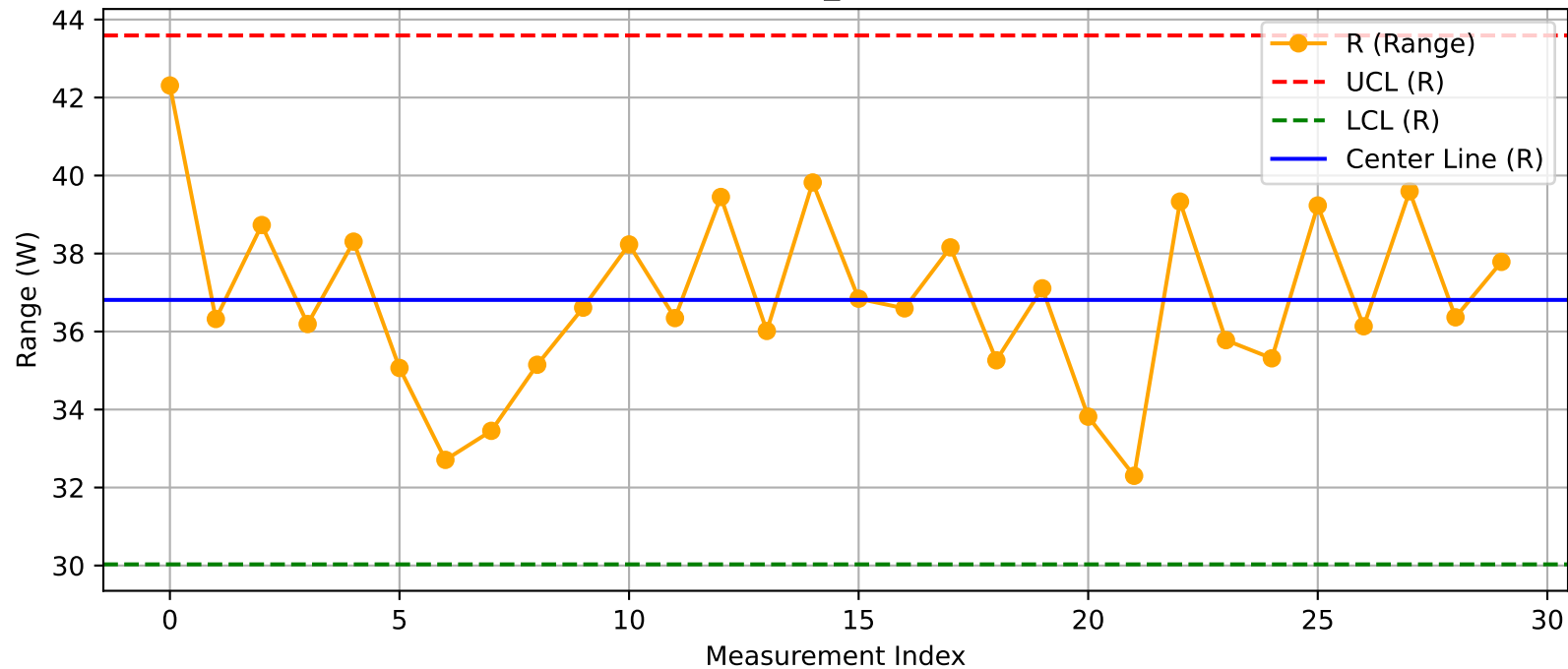
DUT - R Chart (T07_Test100@Test.xlsx)
