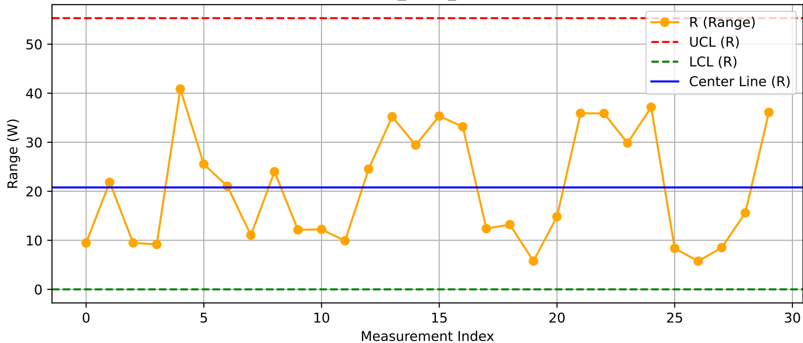
DUT - R Chart (T8_Test2_Nuitka@Test.xlsx)
