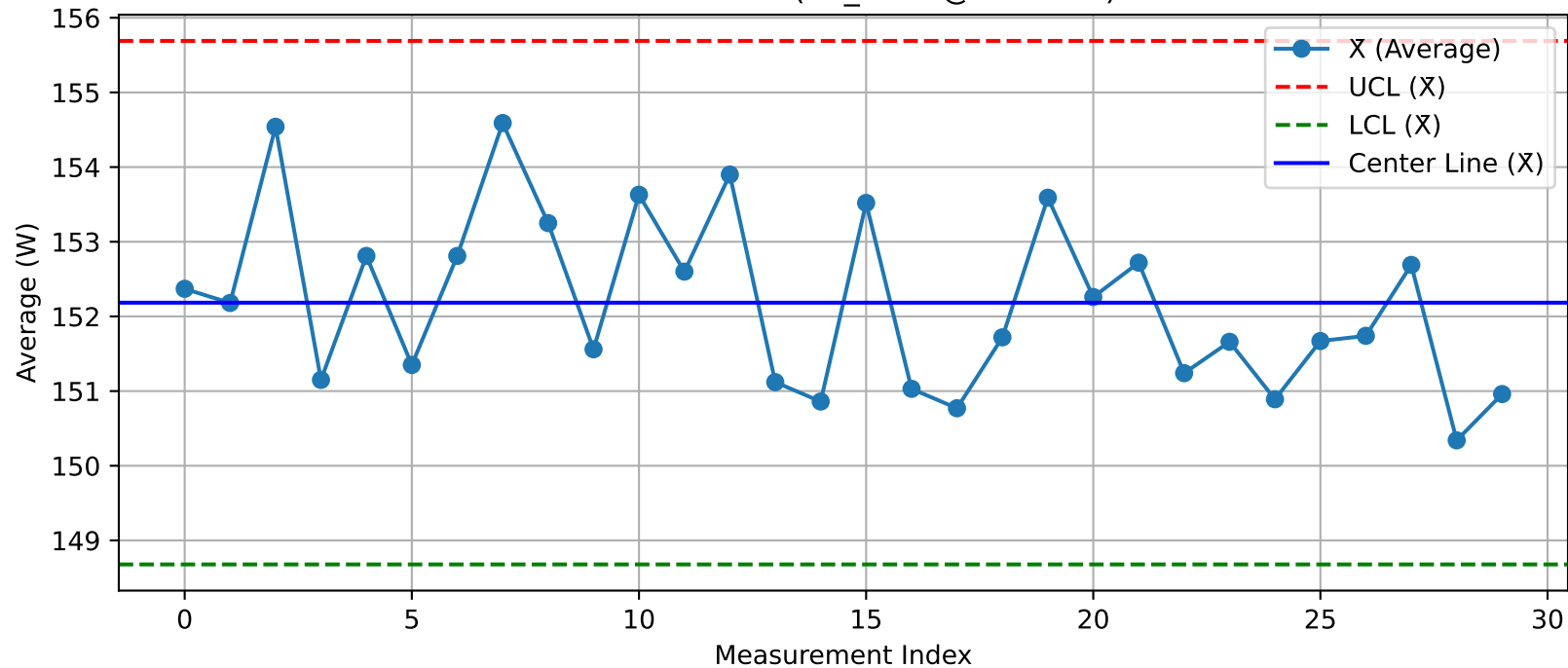
DUT - \bar{X} Chart (T8_Test2@Test.xlsx)
