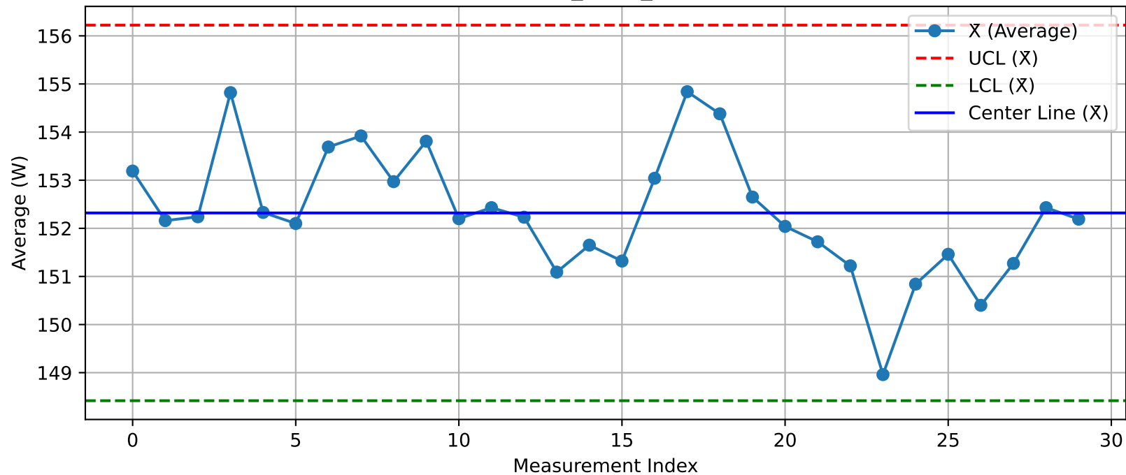
DUT - \bar{X} Chart (T49_Test1_Nuitka@Test.xlsx)
