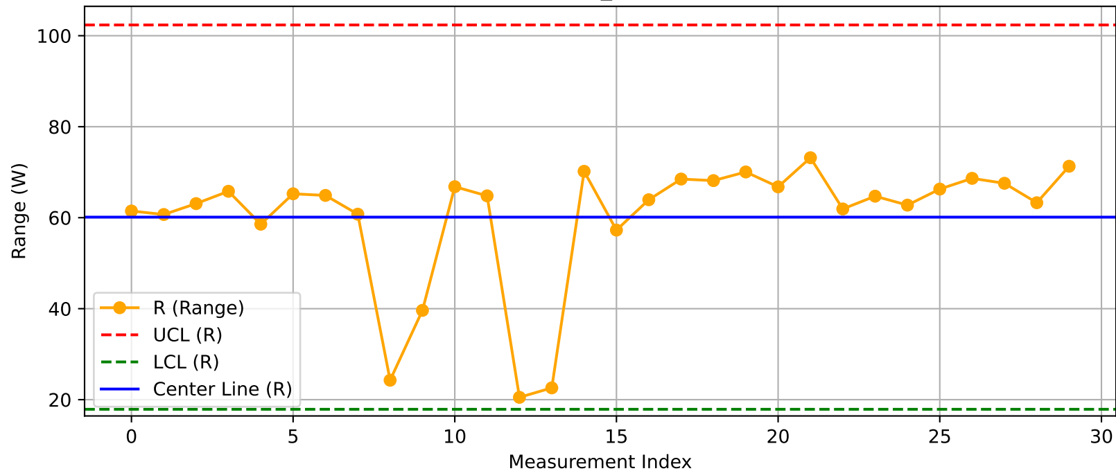
DUT - R Chart (T4_Test1@Test.xlsx)
