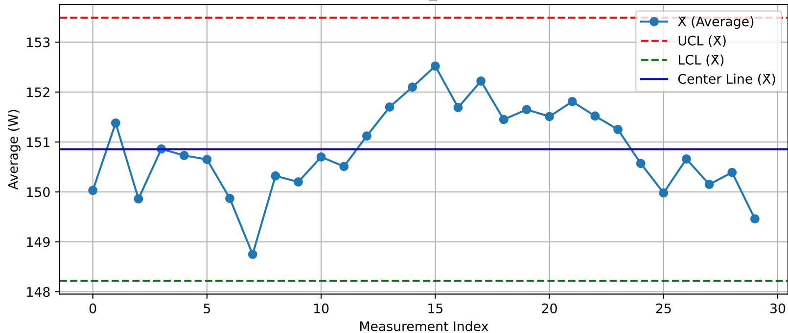
DUT - \bar{X} Chart (T25_Test1@Test.xlsx)
