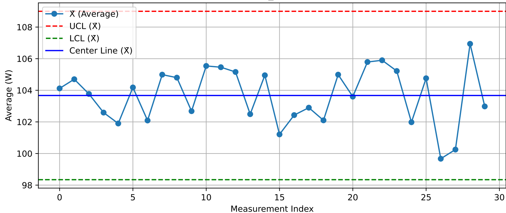
DUT - \bar{X} Chart (T49_Test103@Test.xlsx)
