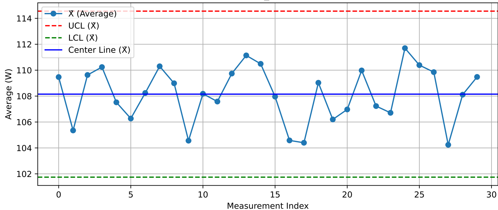
DUT - \bar{X} Chart (T09_Test103@Test.xlsx)
