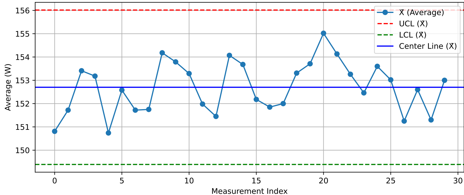
DUT - \bar{X} Chart (T50_Test1_Nuitka@Test.xlsx)
