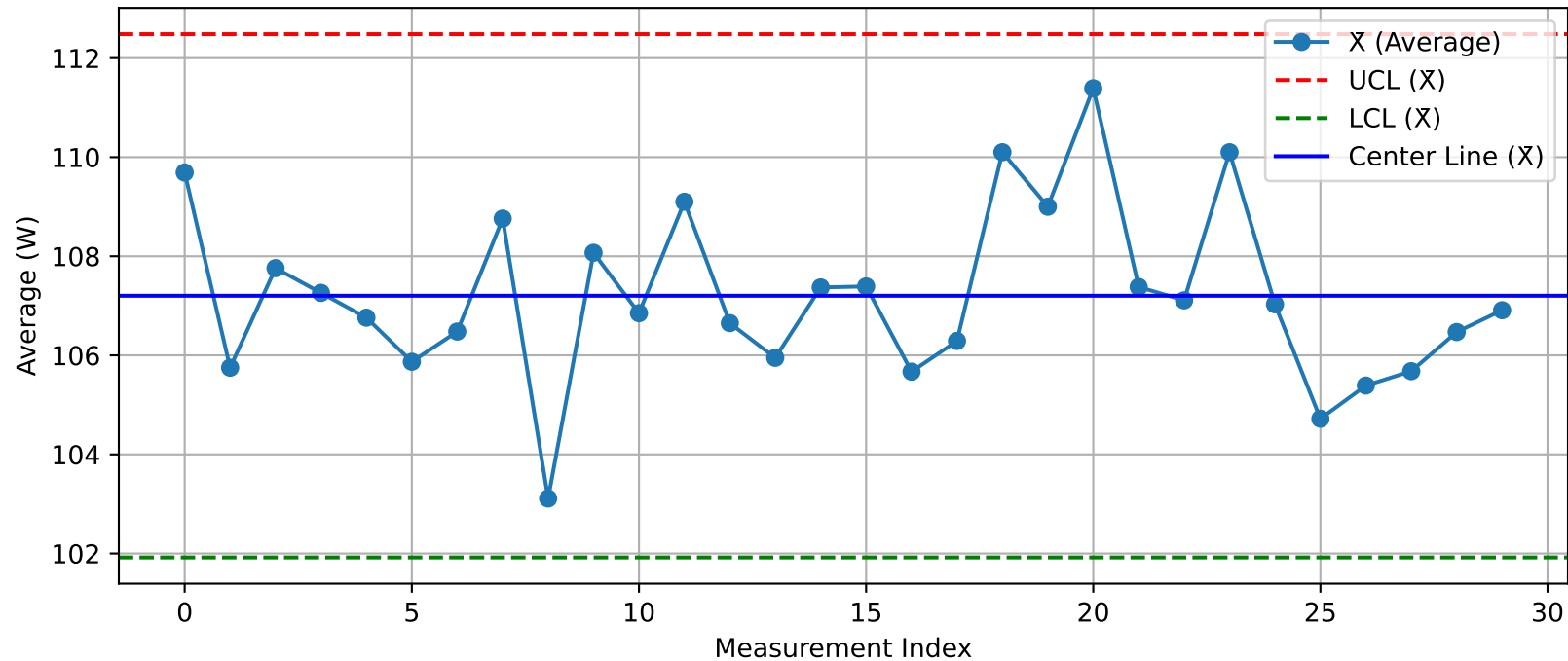
DUT - \bar{X} Chart (T09_Test2O3@Test.xlsx)
