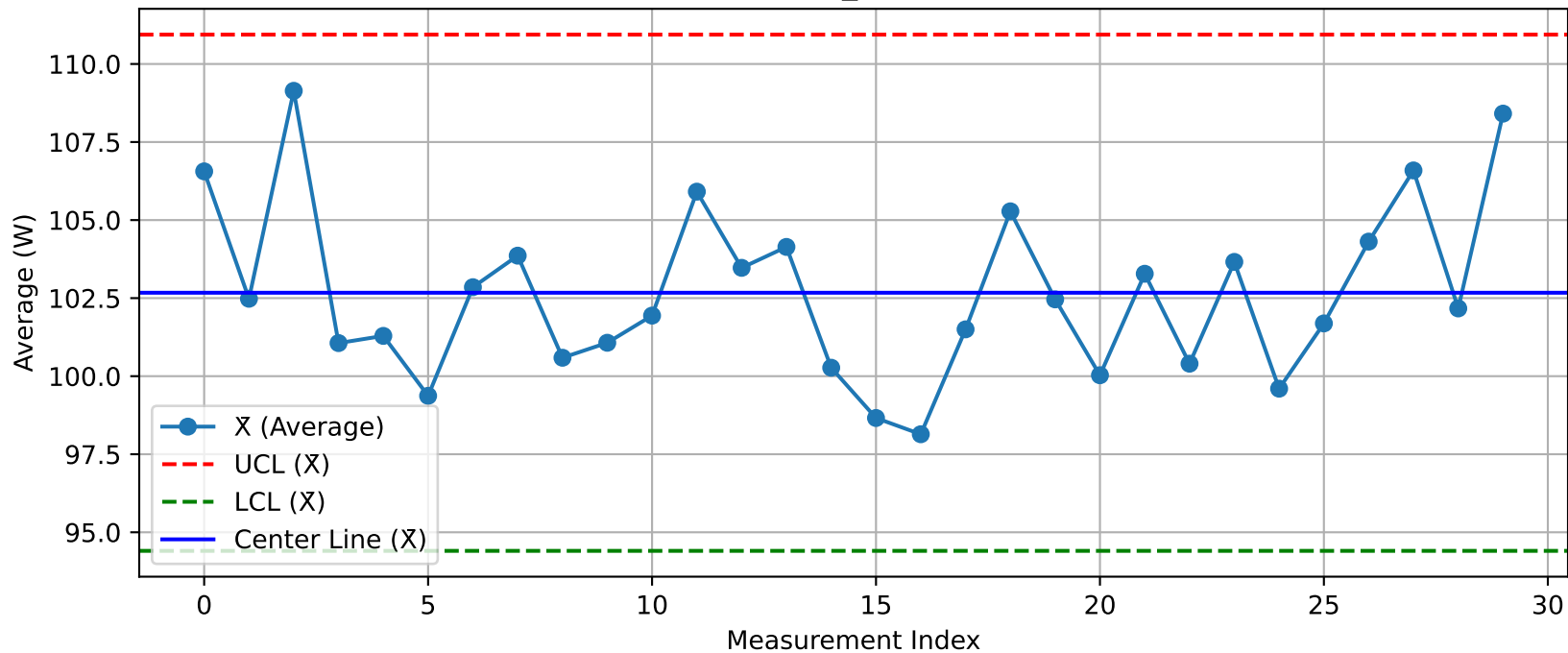
DUT - \bar{X} Chart (T44_Test103@Test.xlsx)
