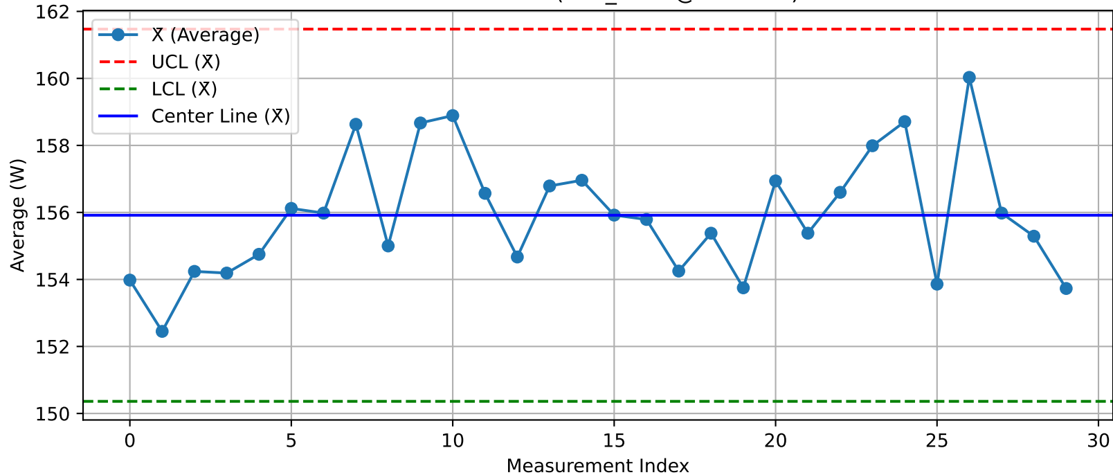
DUT - \bar{X} Chart (T44_Test2@Test.xlsx)
