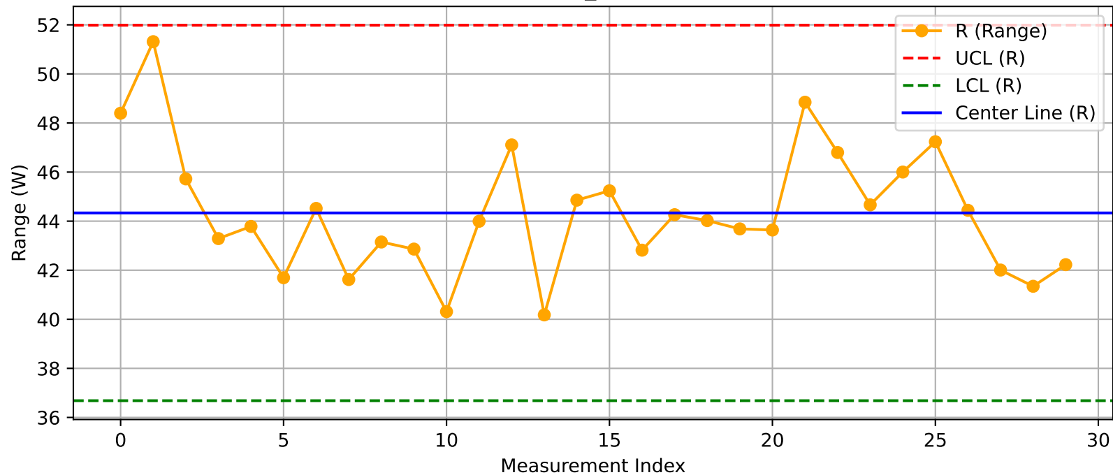
DUT - R Chart (T19_Test103@Test.xlsx)
