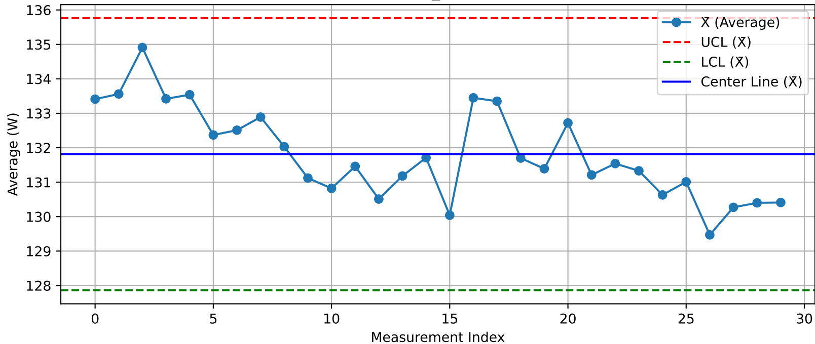
DUT - \bar{X} Chart (T25_Test103@Test.xlsx)
