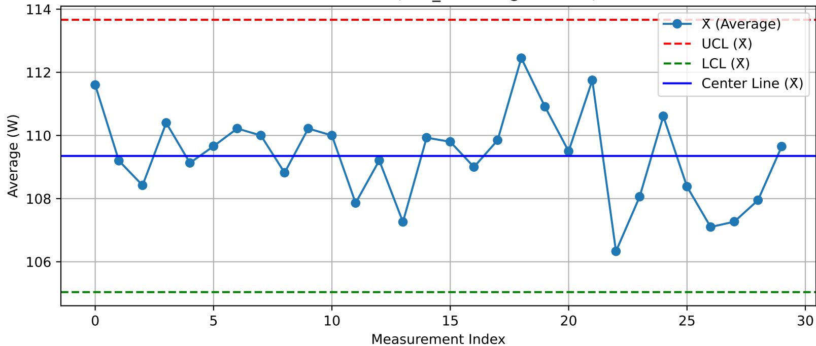
DUT - \bar{X} Chart (T12_Test200@Test.xlsx)
