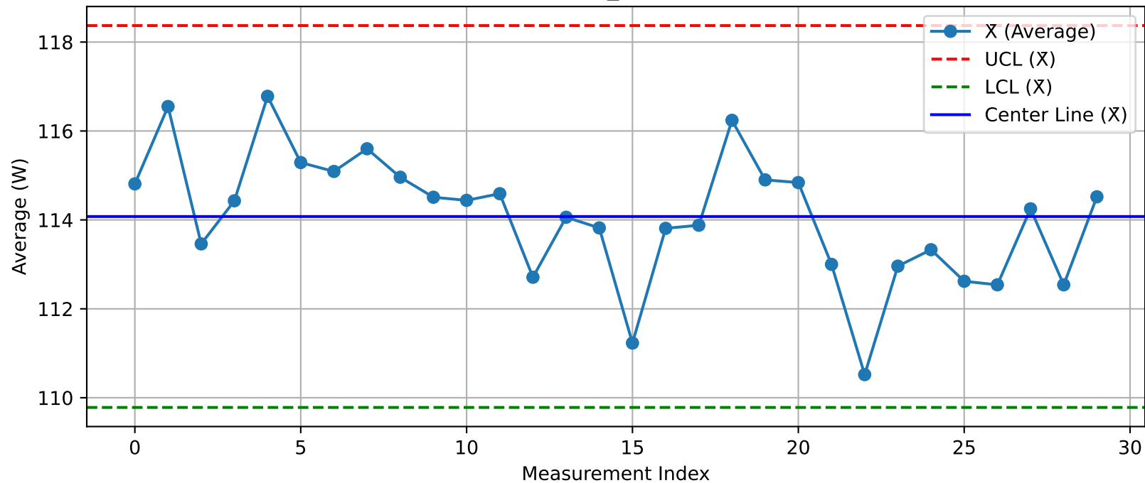
DUT - \bar{X} Chart (T11_Test103@Test.xlsx)
