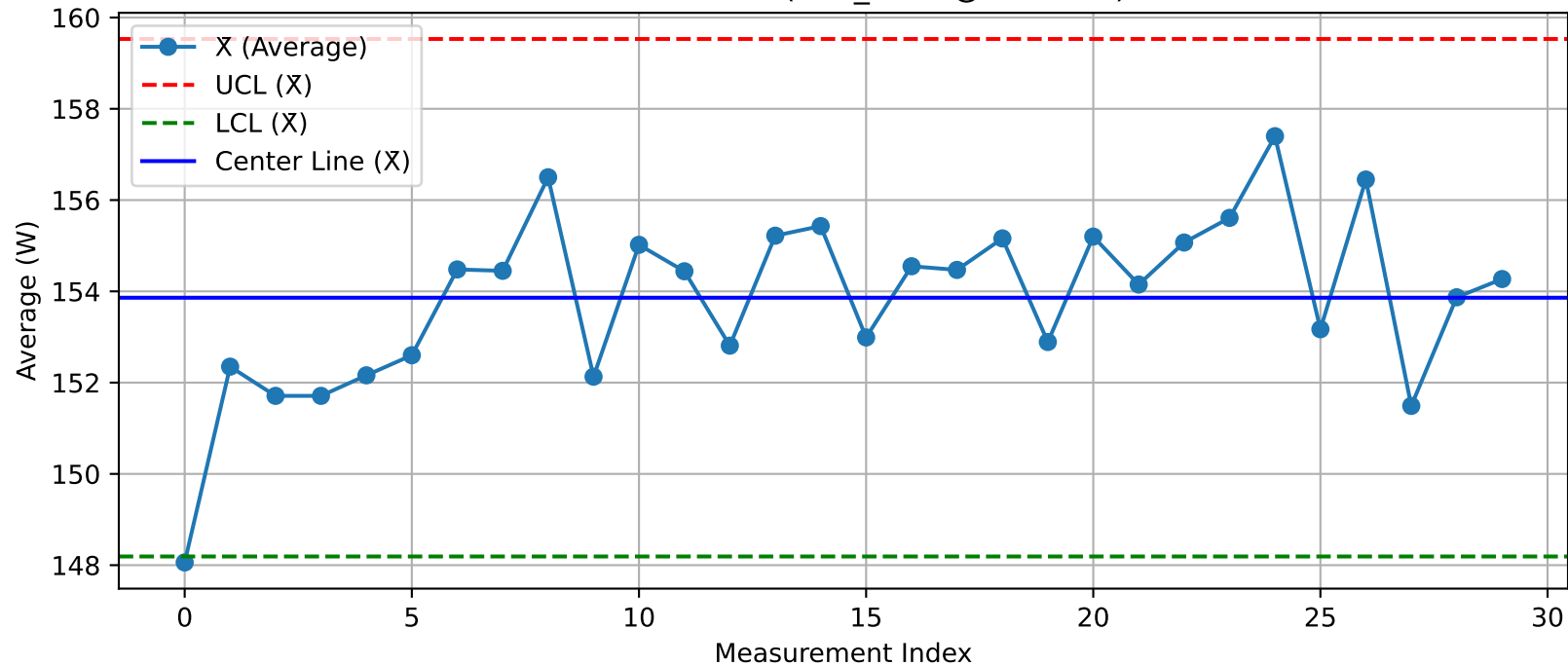
DUT - \bar{X} Chart (T44_Test1@Test.xlsx)
