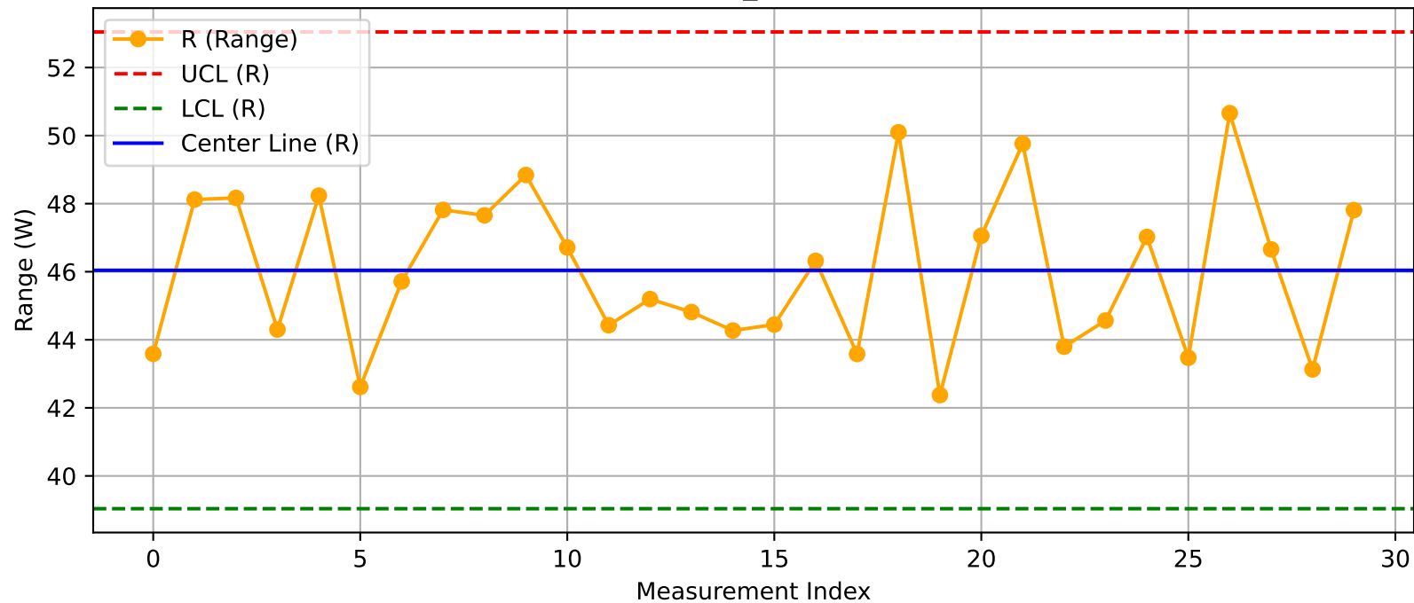
DUT - R Chart (T26_Test200@Test.xlsx)
