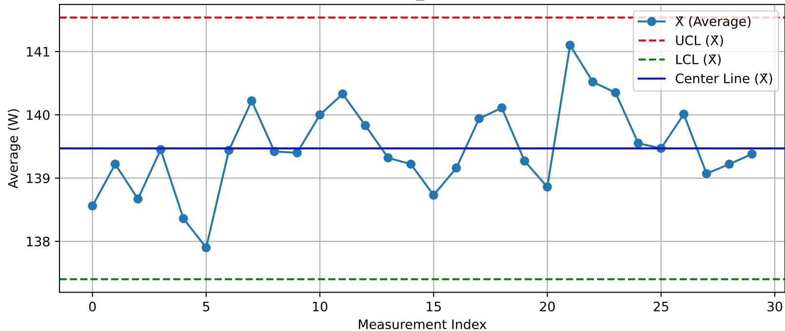
DUT - \bar{X} Chart (T26_Test200@Test.xlsx)
