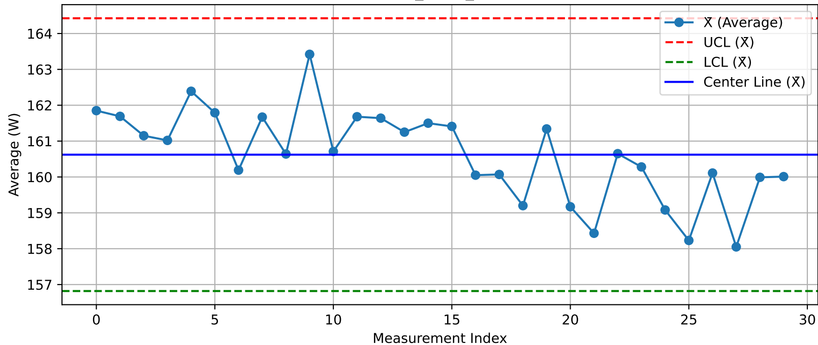
DUT - \bar{X} Chart (T51_Test1_Nuitka@Test.xlsx)
