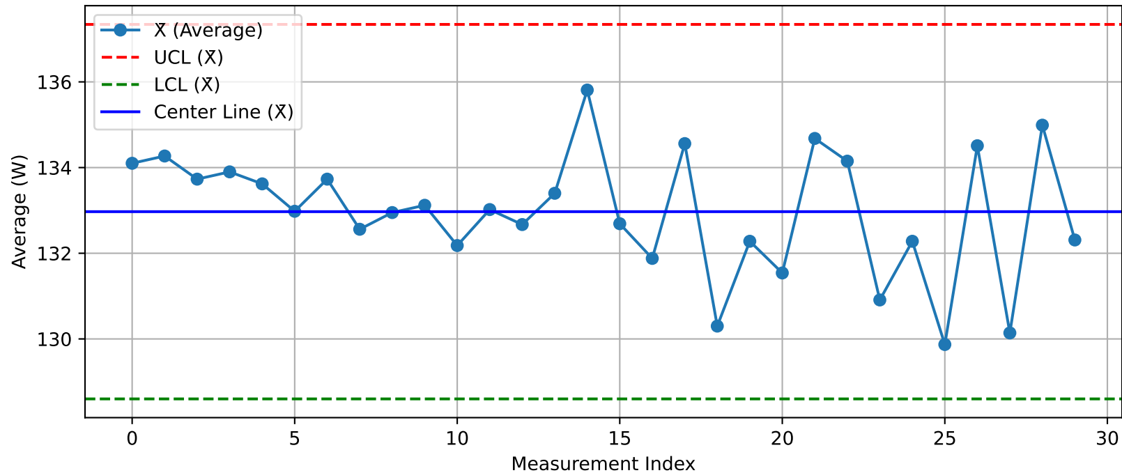
DUT - \bar{X} Chart (T8_Test2_Xint@Test.xlsx)
