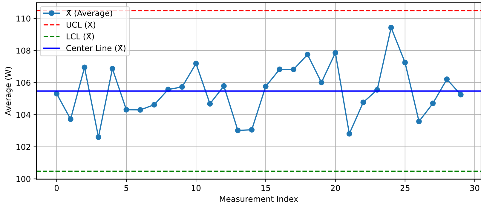
DUT - \bar{X} Chart (T12_Test203@Test.xlsx)
