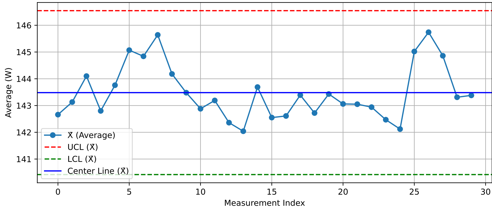
DUT - \bar{X} Chart (T36_Test1_Xint@Test.xlsx)
