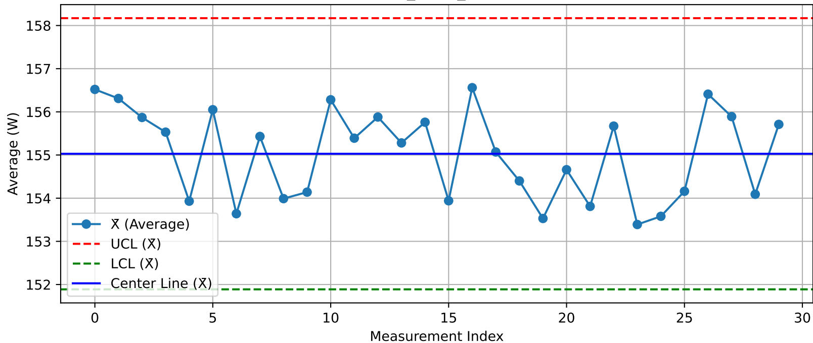
DUT - \bar{X} Chart (T4_Test1_Nuitka@Test.xlsx)
