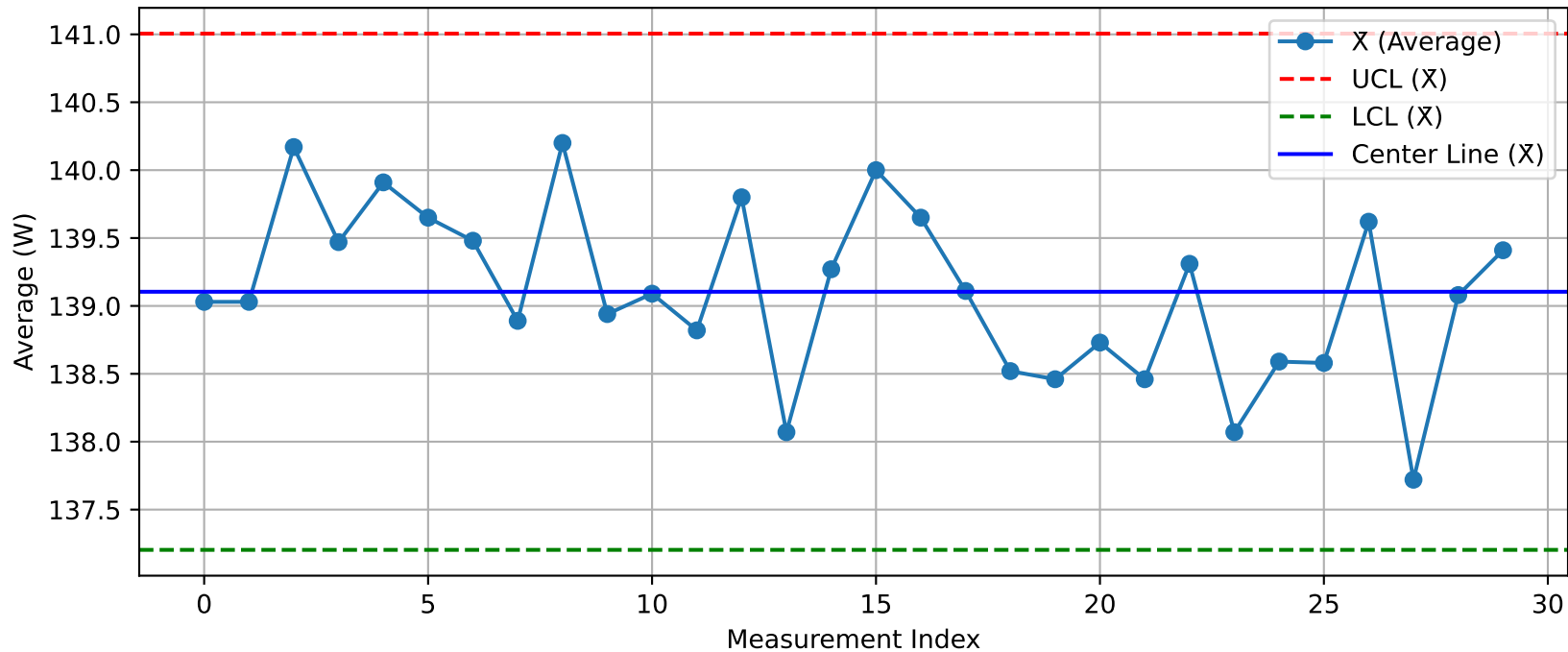
DUT - \bar{X} Chart (T5_Test2@Test.xlsx)
