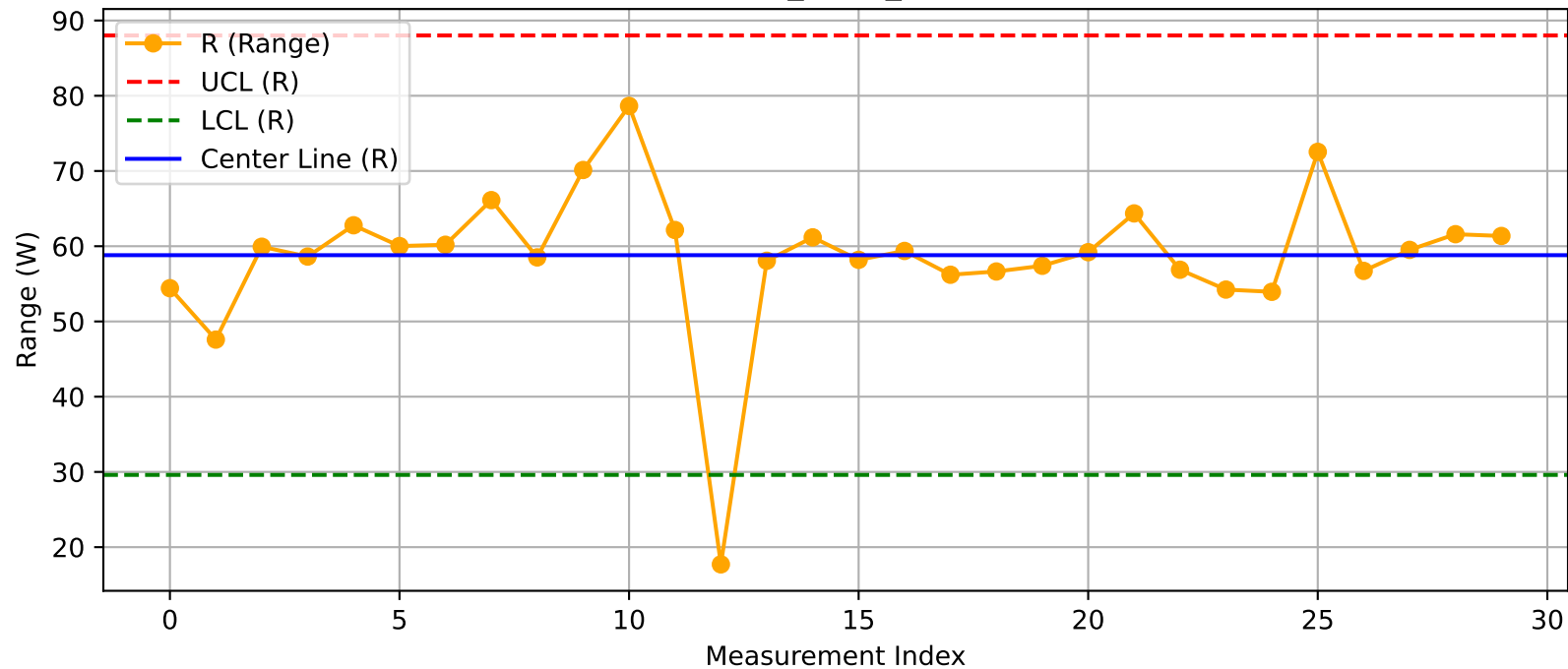
DUT - R Chart (T40_Test2_Nuitka@Test.xlsx)
