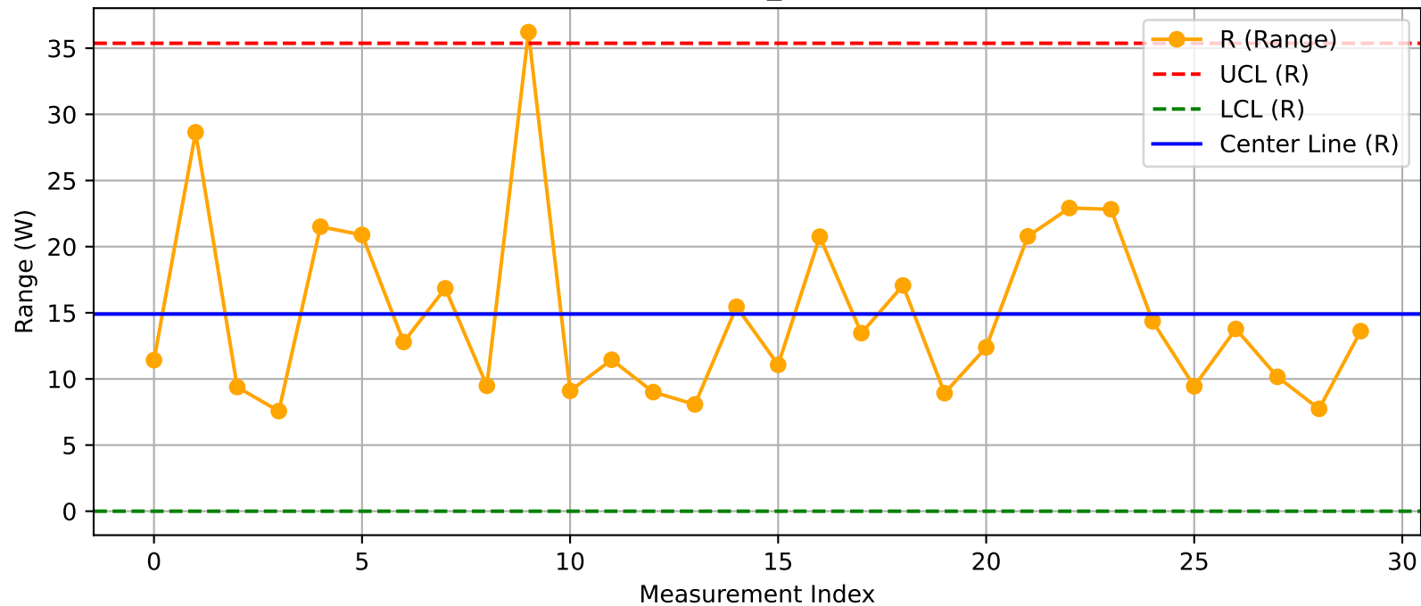
DUT - R Chart (T50_Test2@Test.xlsx)
