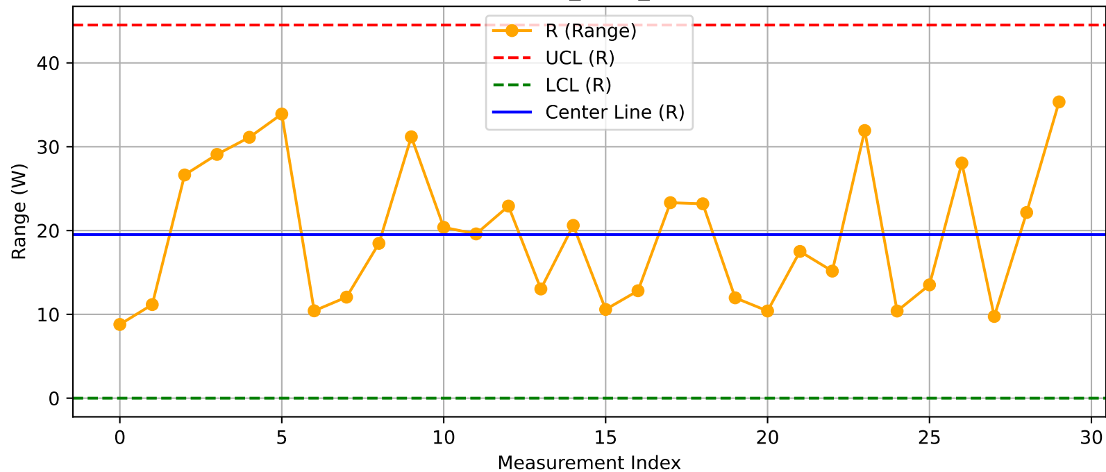
DUT - R Chart (T13_Test1_Xint@Test.xlsx)
