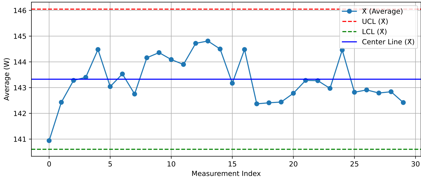
DUT - \bar{X} Chart (T8_Test1@Test.xlsx)
