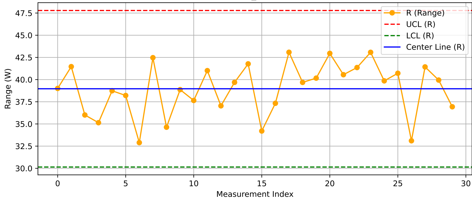
DUT - R Chart (T12_Test100@Test.xlsx)
