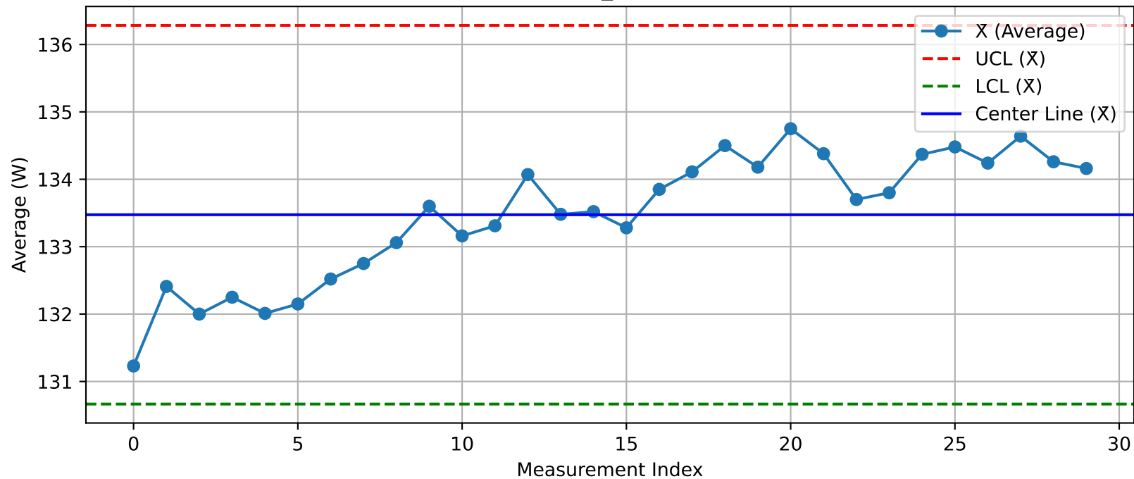
DUT - \bar{X} Chart (T08_Test1O3@Test.xlsx)
