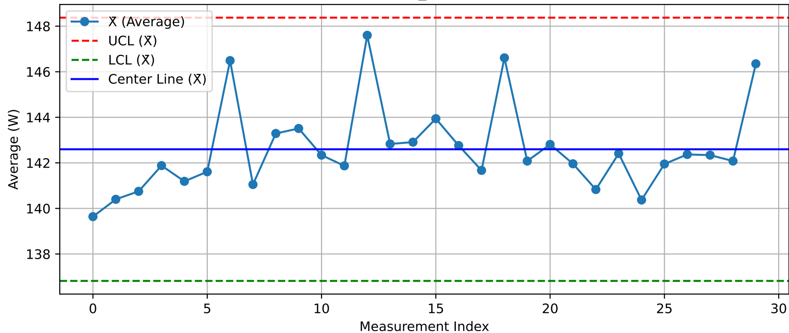
DUT - \bar{X} Chart (T19_Test100@Test.xlsx)
