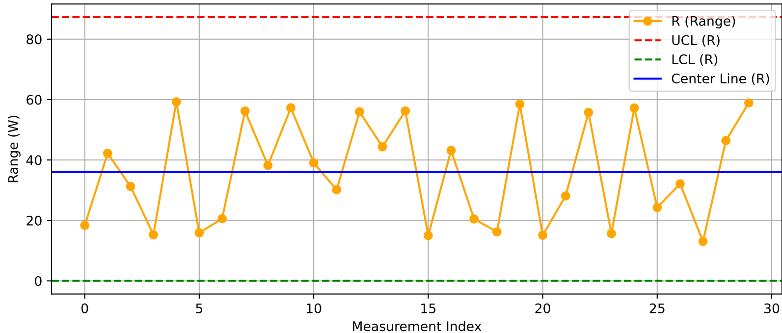
DUT - R Chart (T36_Test2@Test.xlsx)
