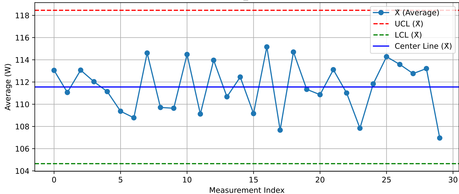
DUT - \bar{X} Chart (T17_Test200@Test.xlsx)
