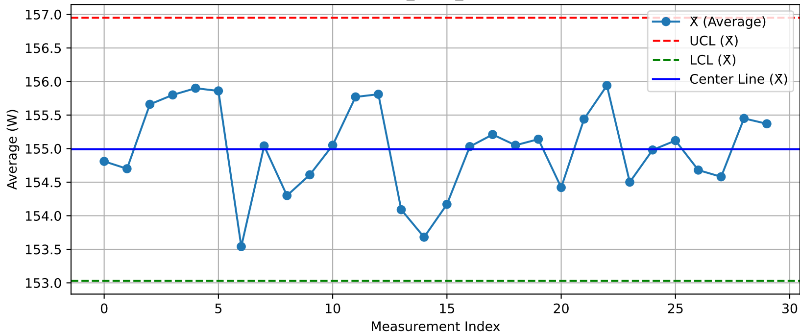
DUT - \bar{X} Chart (T7_Test1_Nuitka@Test.xlsx)
