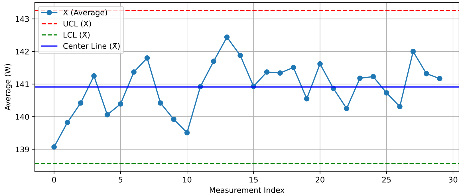
DUT - \bar{X} Chart (T26_Test100@Test.xlsx)
