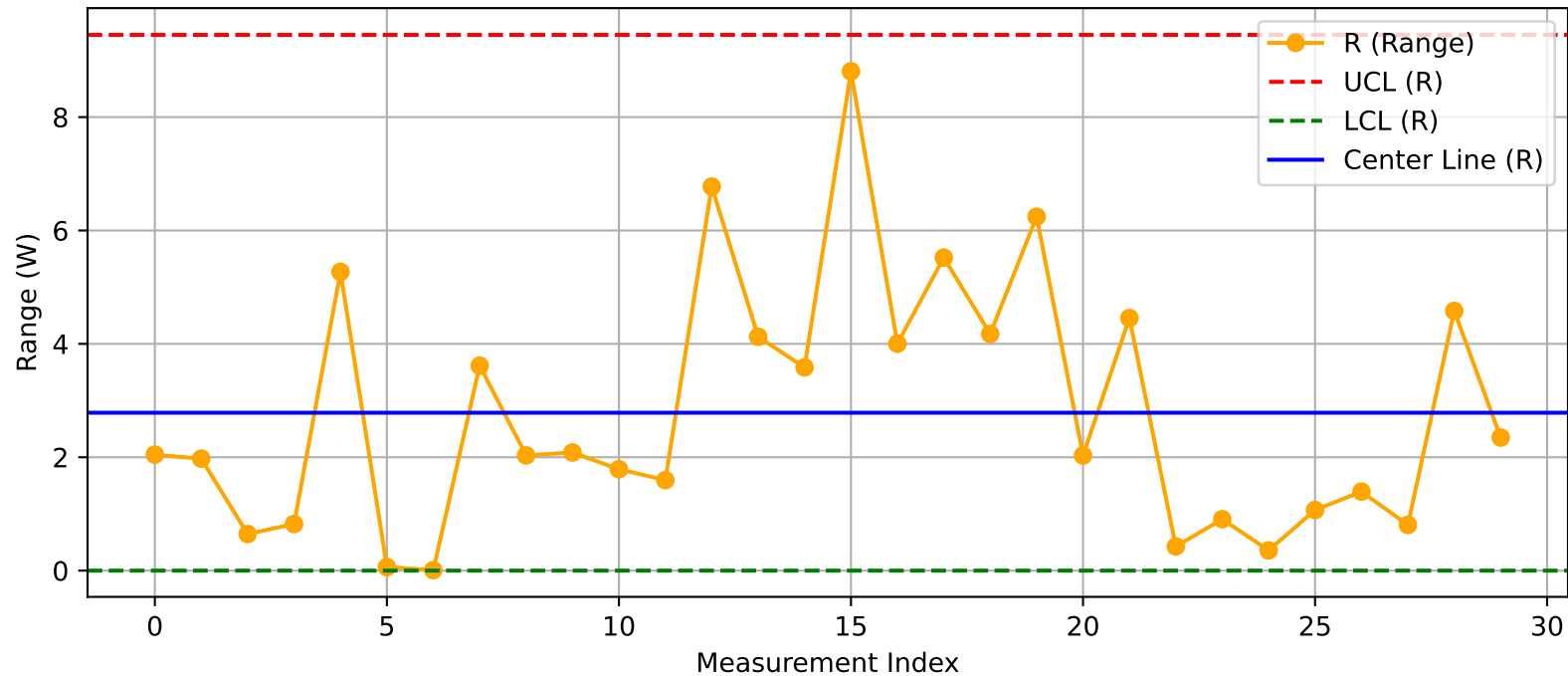
DUT - R Chart (T49_Test103@Test.xlsx)
