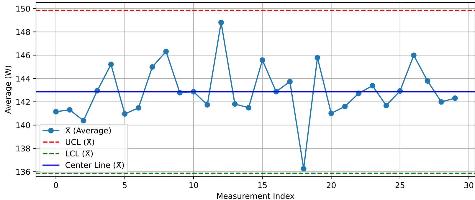
DUT - \bar{X} Chart (T25_Test2@Test.xlsx)
