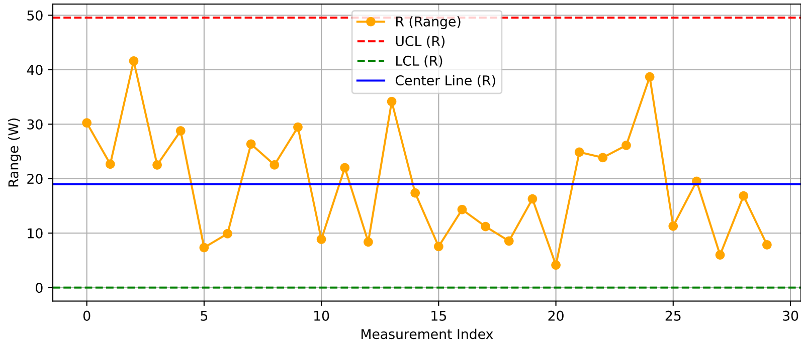
DUT - R Chart (T17_Test1_Nuitka@Test.xlsx)
