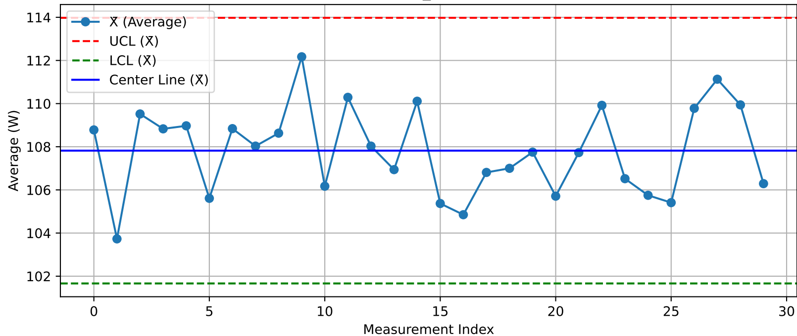
DUT - \bar{X} Chart (T17_Test203@Test.xlsx)
