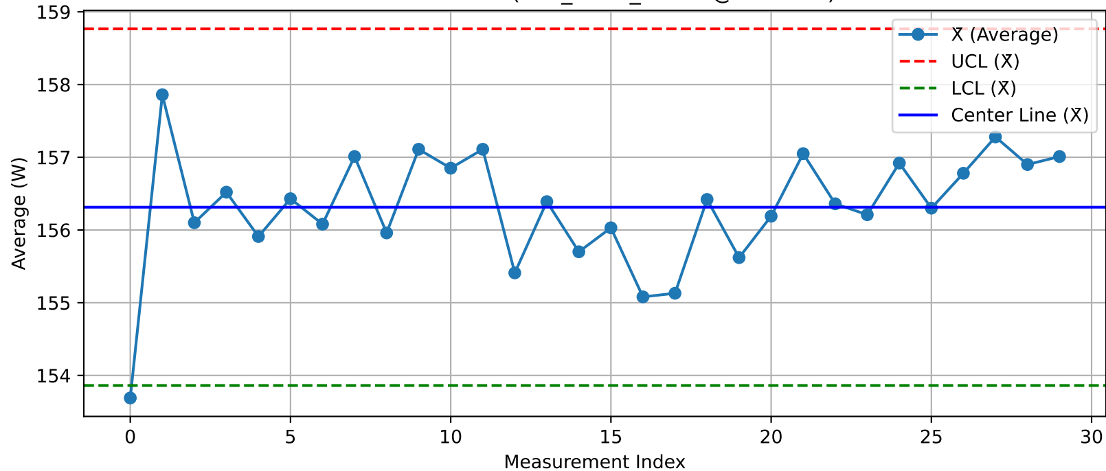
DUT - \bar{X} Chart (T11_Test2_Nuitka@Test.xlsx)
