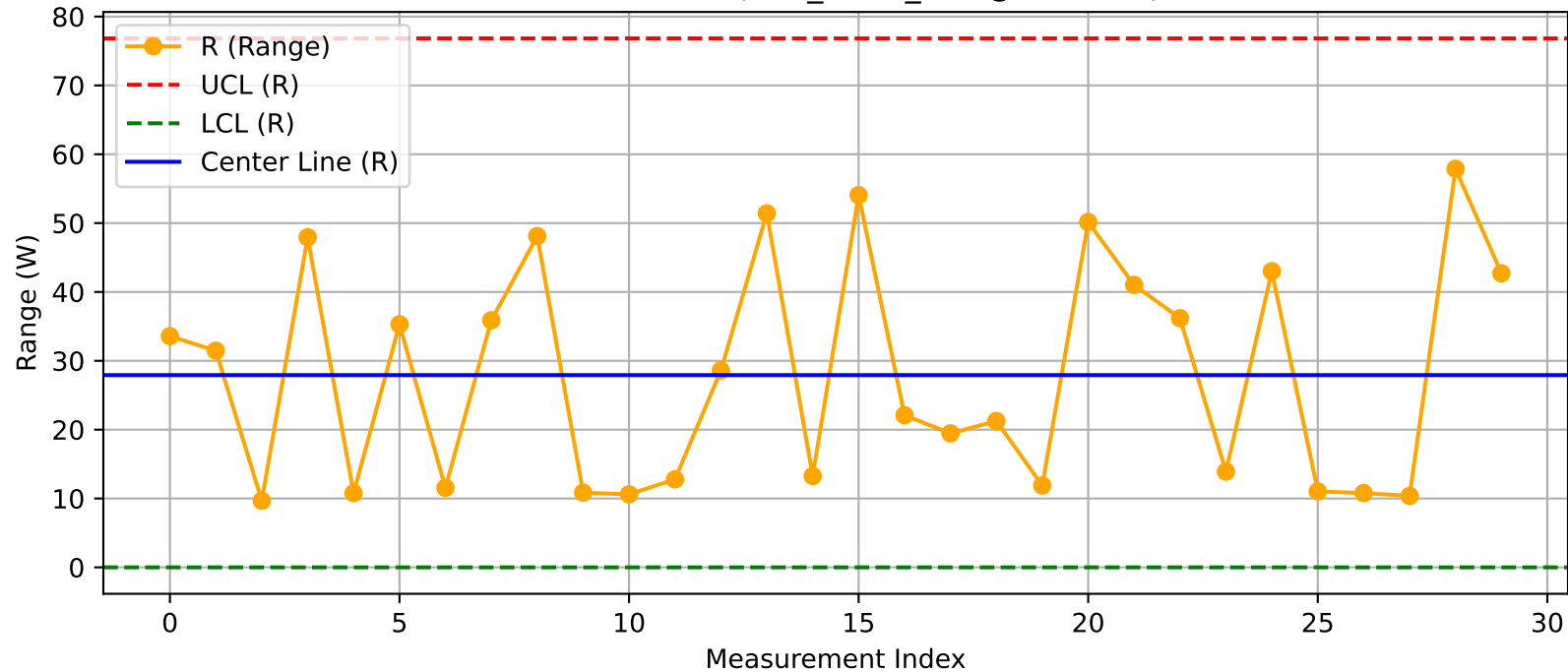
DUT - R Chart (T28_Test1_Xint@Test.xlsx)
