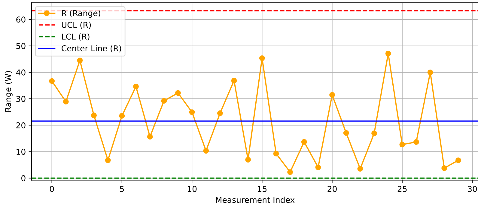
DUT - R Chart (T44_Test2_Nuitka@Test.xlsx)
