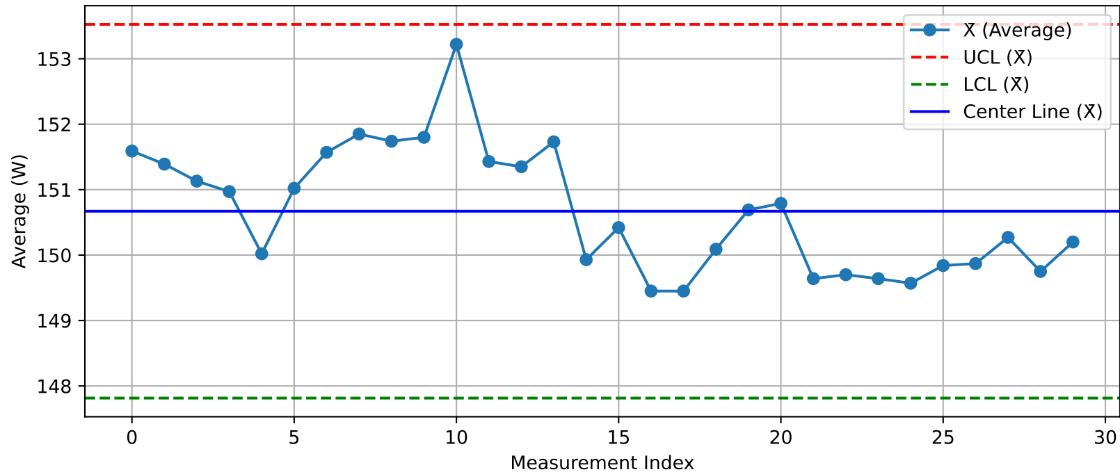
DUT - \bar{X} Chart (T13_Test1_Nuitka@Test.xlsx)
