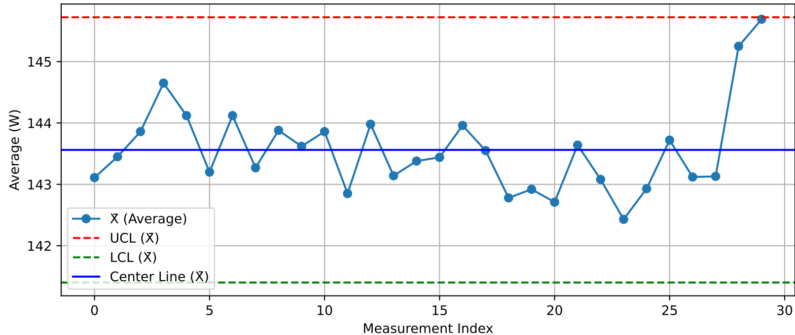
DUT - \bar{X} Chart (T51_Test2O3@Test.xlsx)
