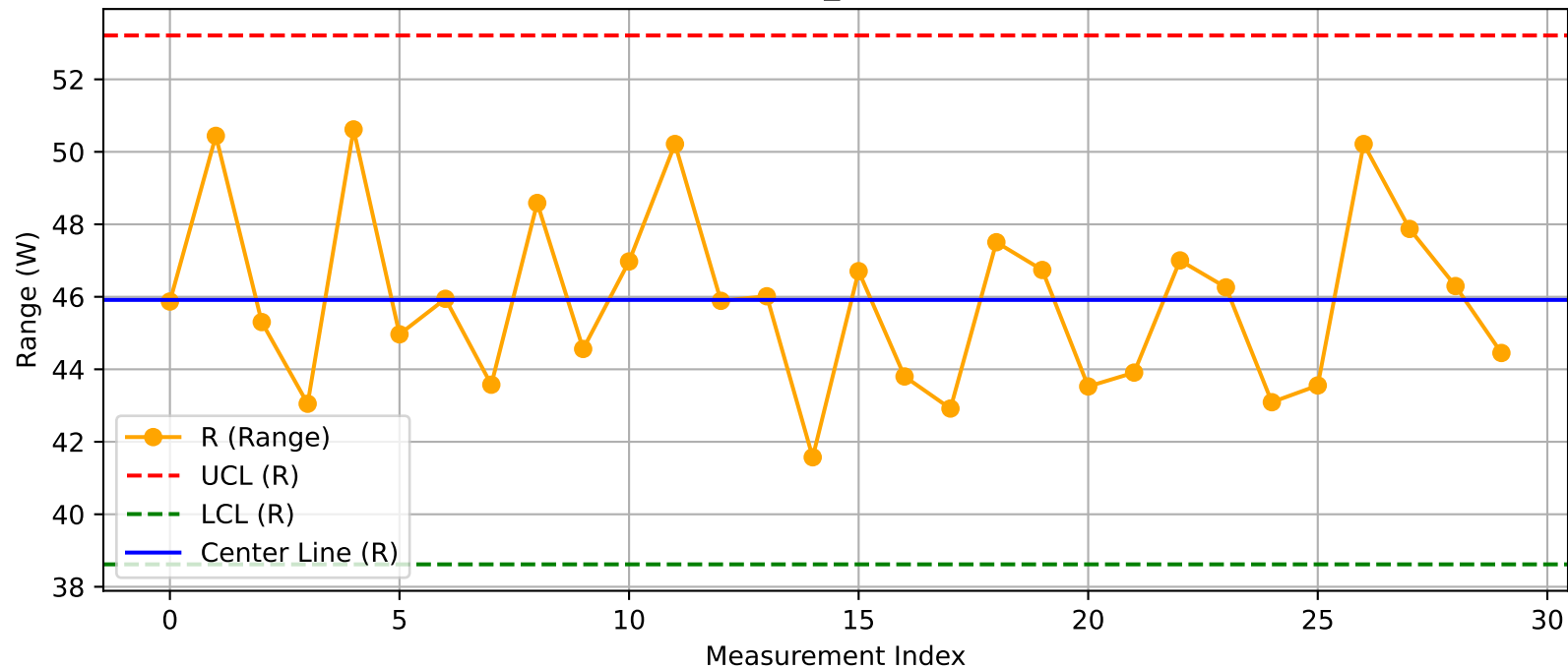
DUT - R Chart (T25_Test100@Test.xlsx)
