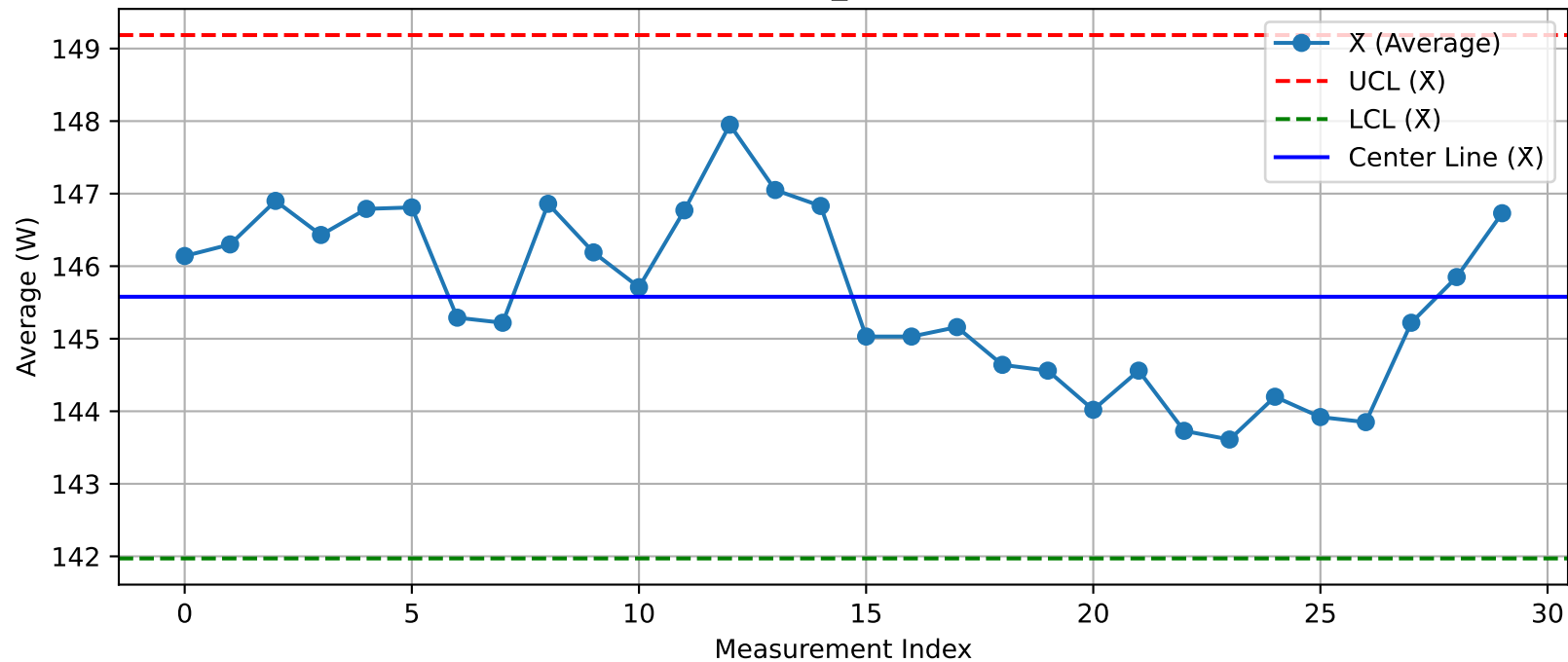
DUT - \bar{X} Chart (T05_Test200@Test.xlsx)
