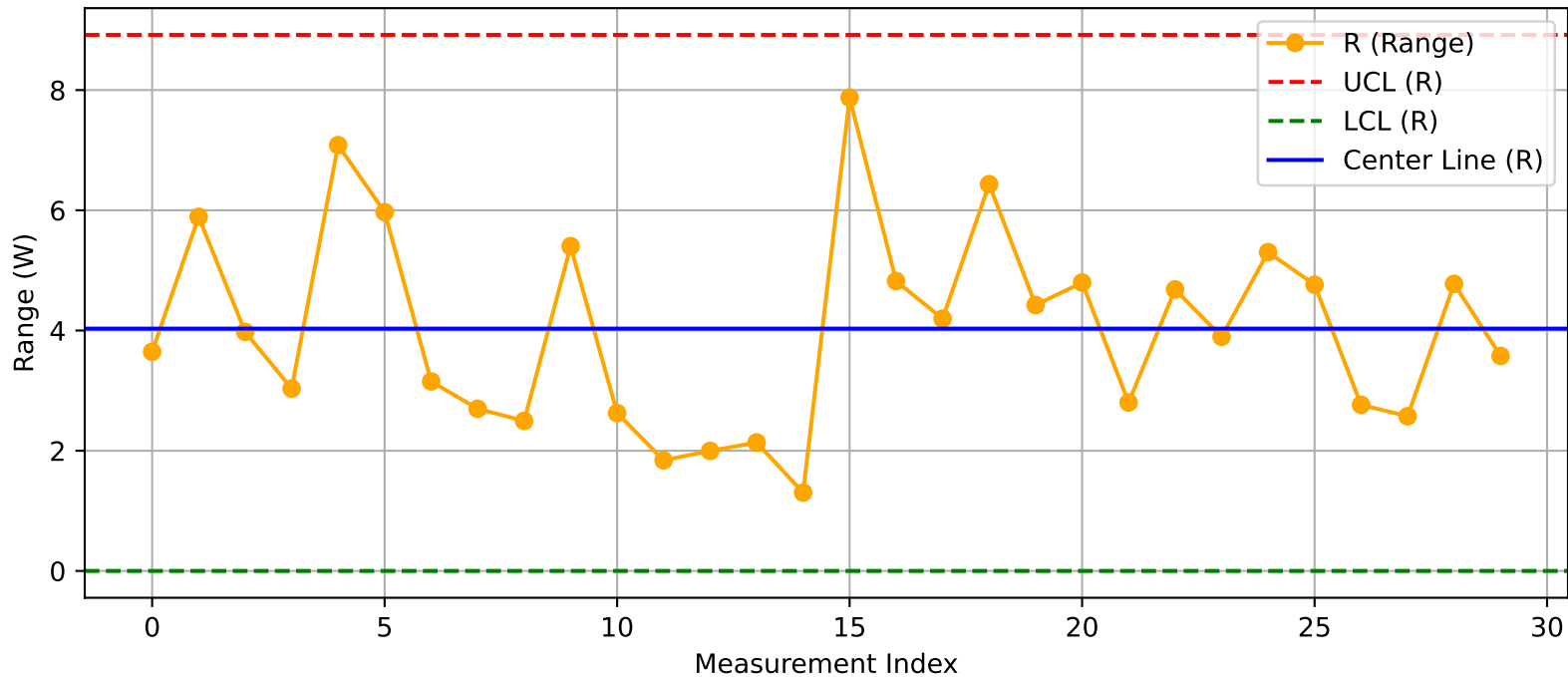
DUT - R Chart (T19_Test2@Test.xlsx)
