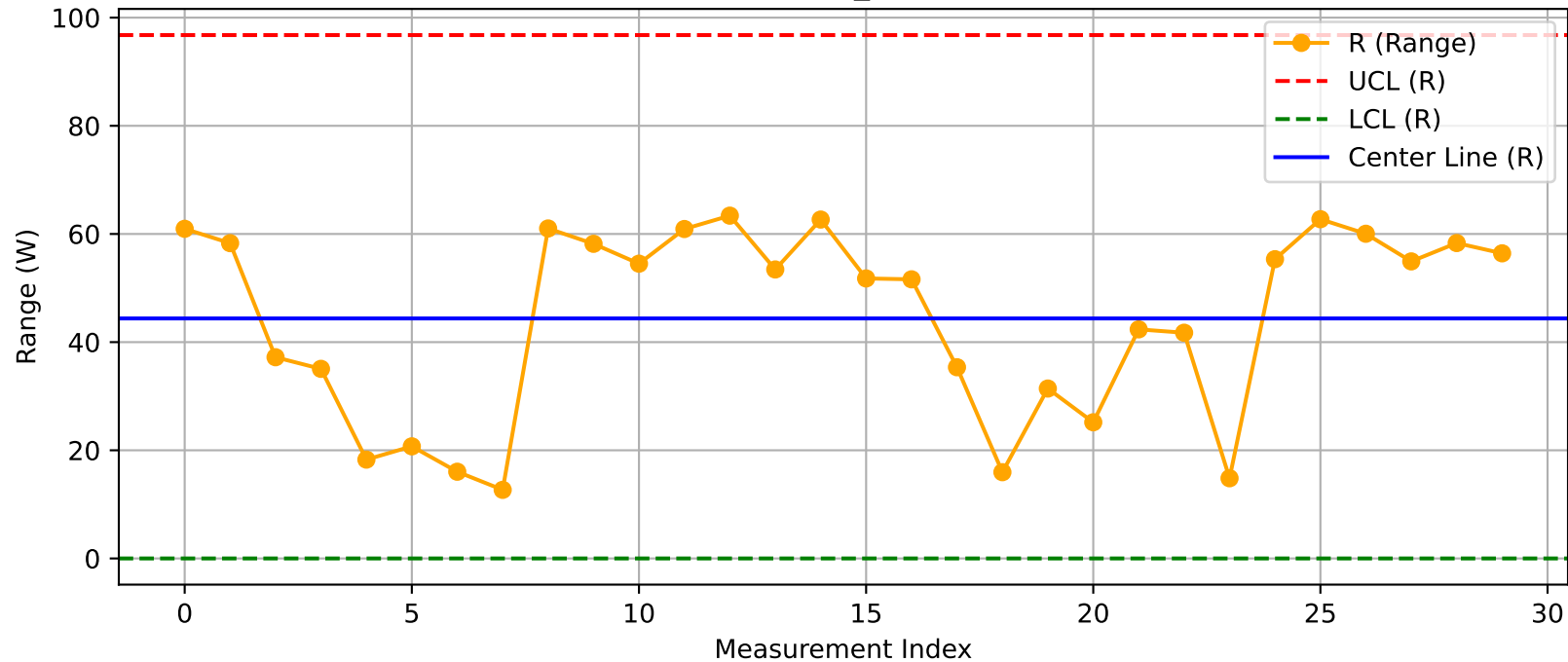
DUT - R Chart (T40_Test2@Test.xlsx)
