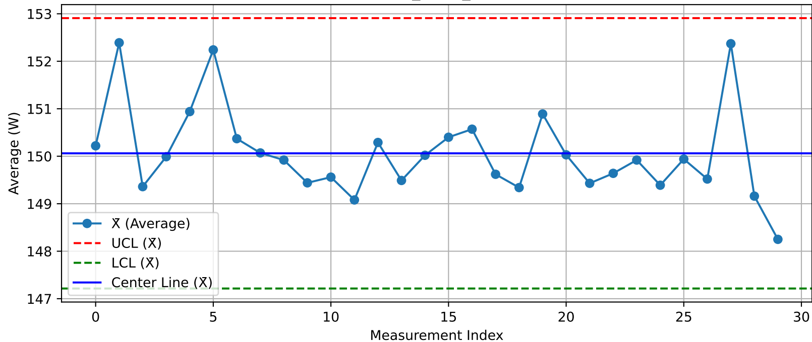
DUT - \bar{X} Chart (T19_Test2_Nuitka@Test.xlsx)
