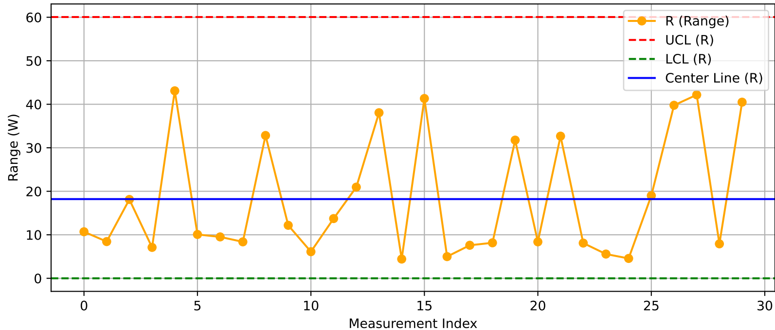
DUT - R Chart (T29_Test2_Nuitka@Test.xlsx)
