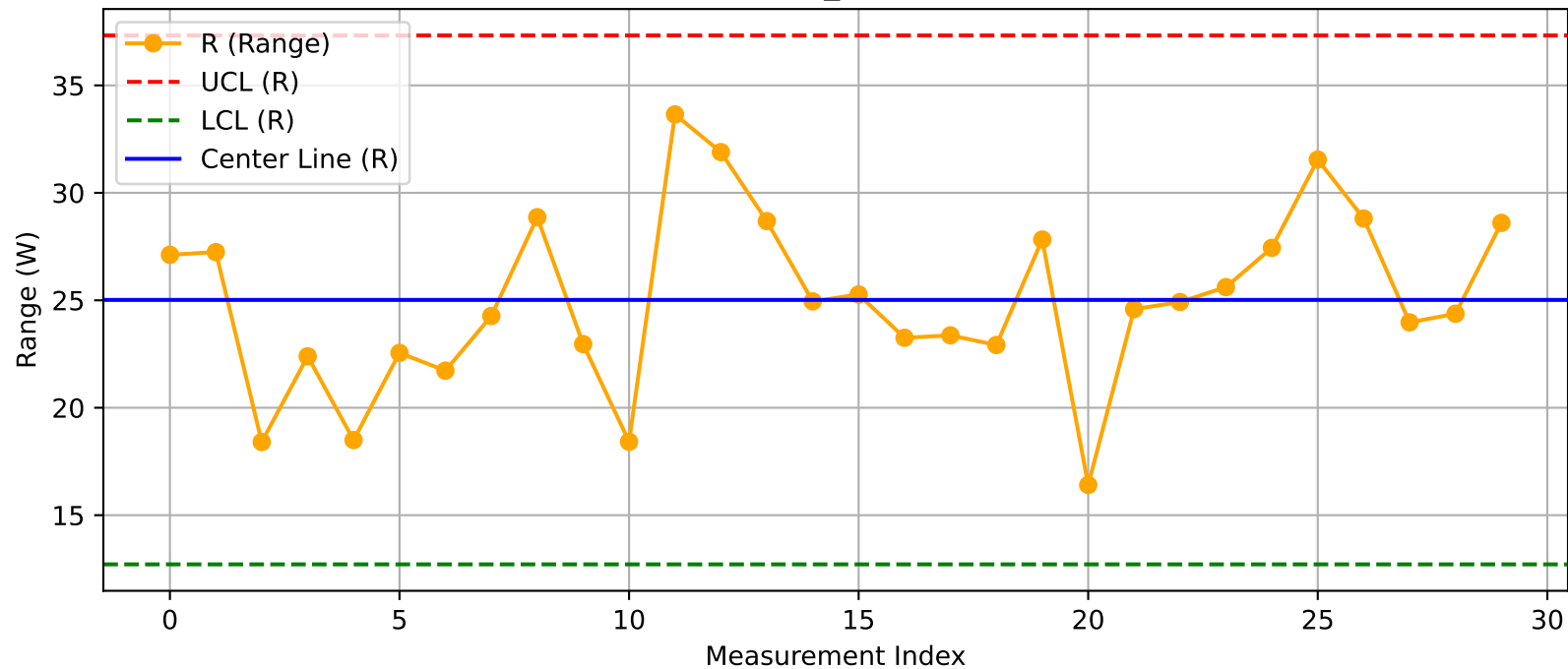
DUT - R Chart (T17_Test100@Test.xlsx)
