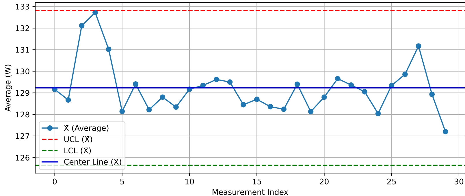
DUT - \bar{X} Chart (T04_Test1O3@Test.xlsx)
