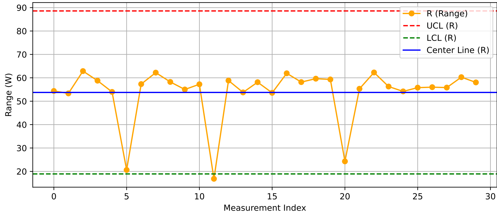
DUT - R Chart (T50_Test1_Xint@Test.xlsx)
