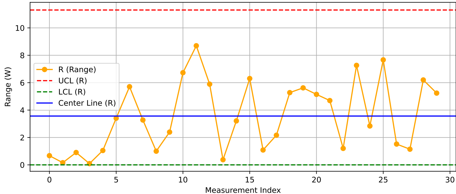
DUT - R Chart (T44_Test2O3@Test.xlsx)
