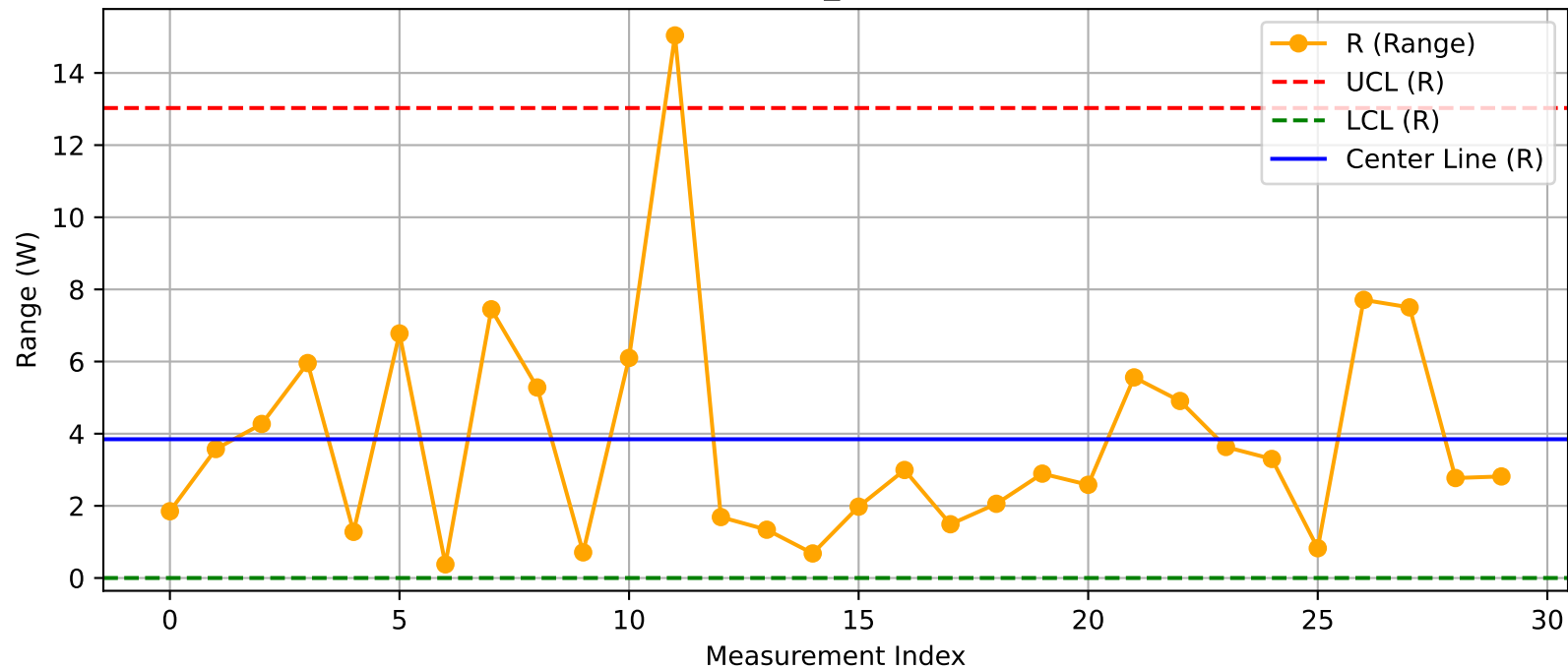
DUT - R Chart (T44_Test200@Test.xlsx)
