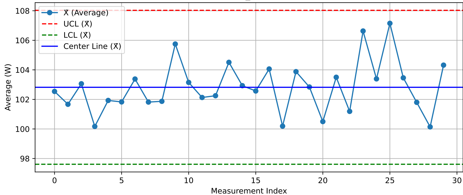
DUT - \bar{X} Chart (T29_Test200@Test.xlsx)
