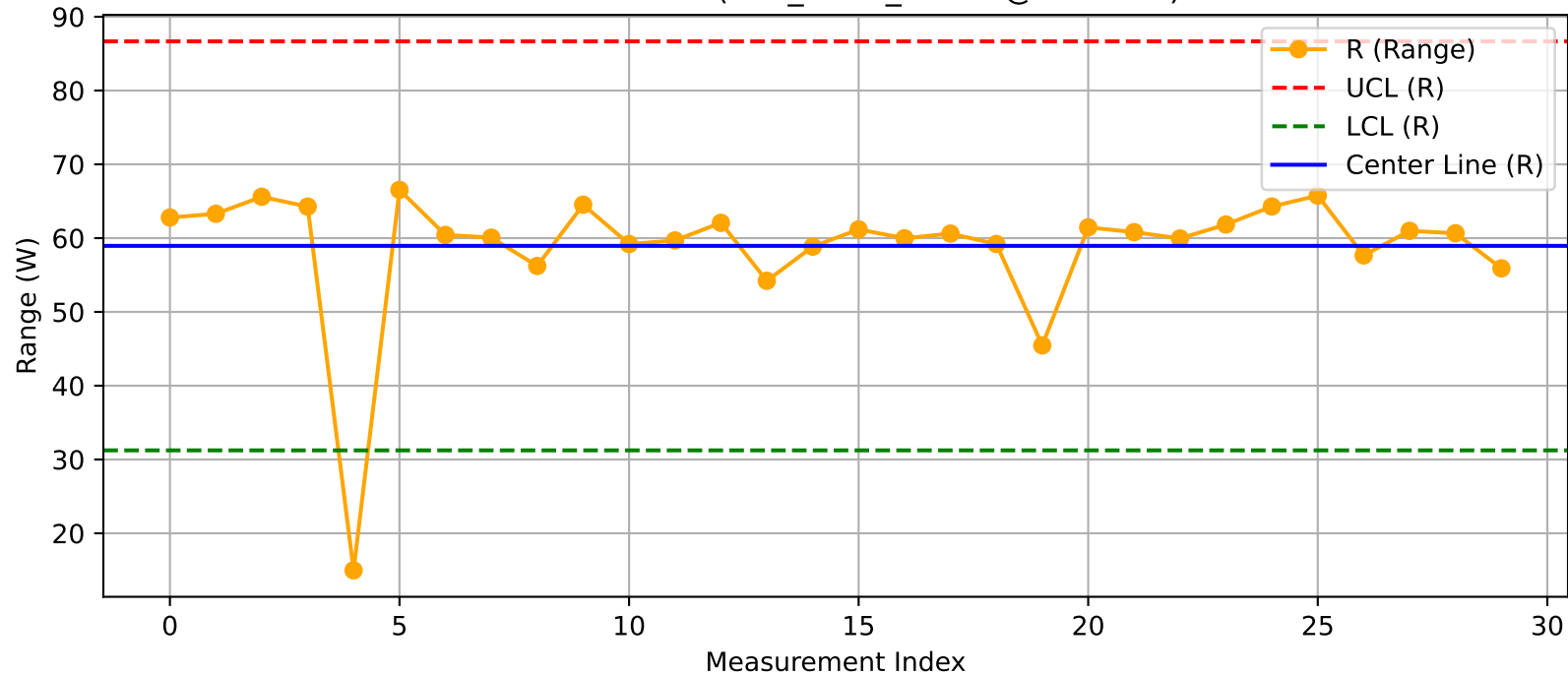
DUT - R Chart (T28_Test2_Nuitka@Test.xlsx)
