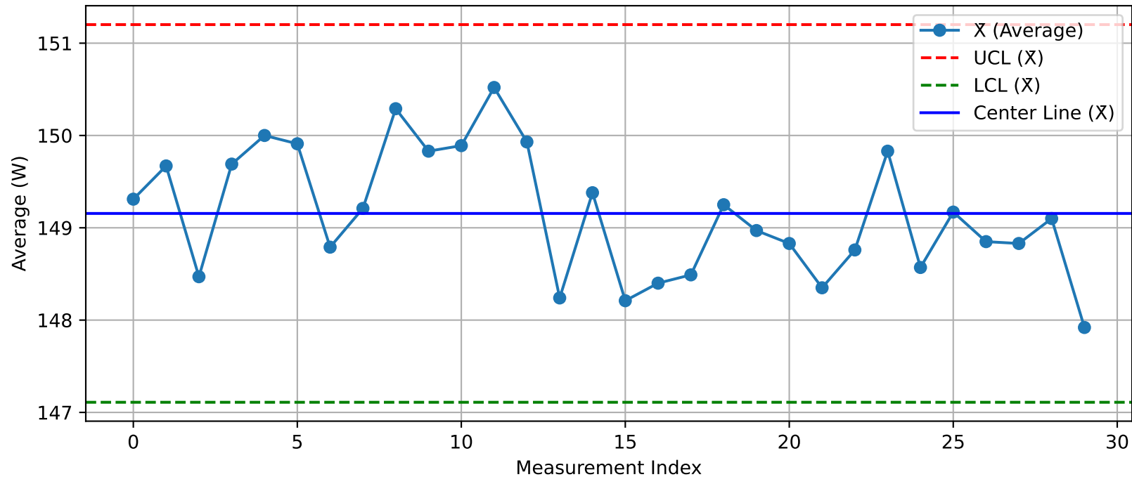
DUT - \bar{X} Chart (T13_Test2_Nuitka@Test.xlsx)
