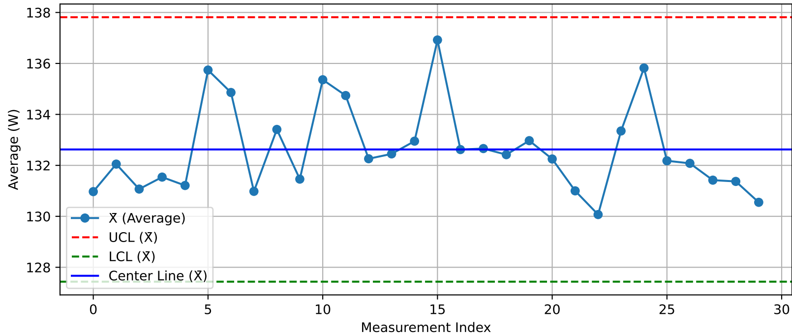
DUT - \bar{X} Chart (T32_Test2_Xint@Test.xlsx)
