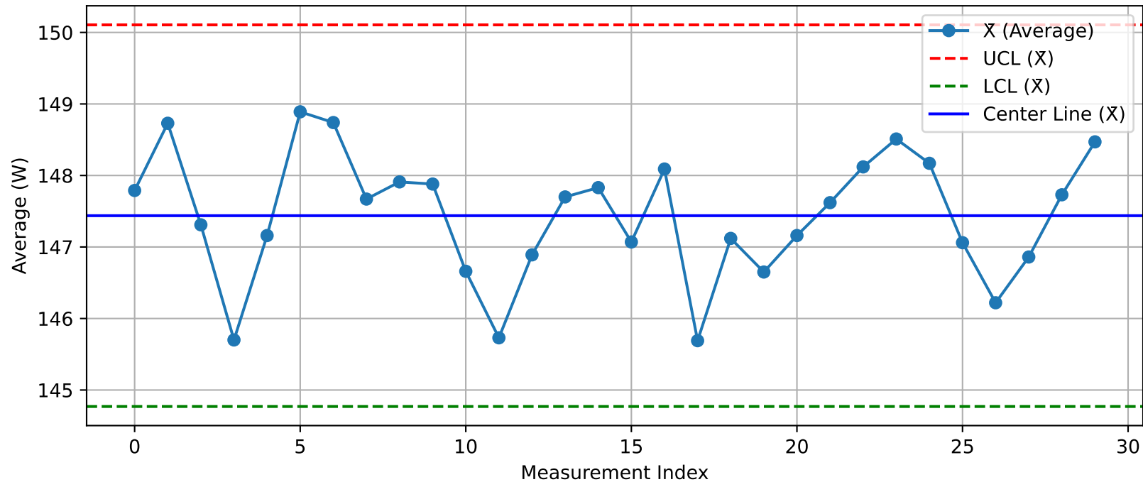
DUT - \bar{X} Chart (T5_Test1_Xint@Test.xlsx)
