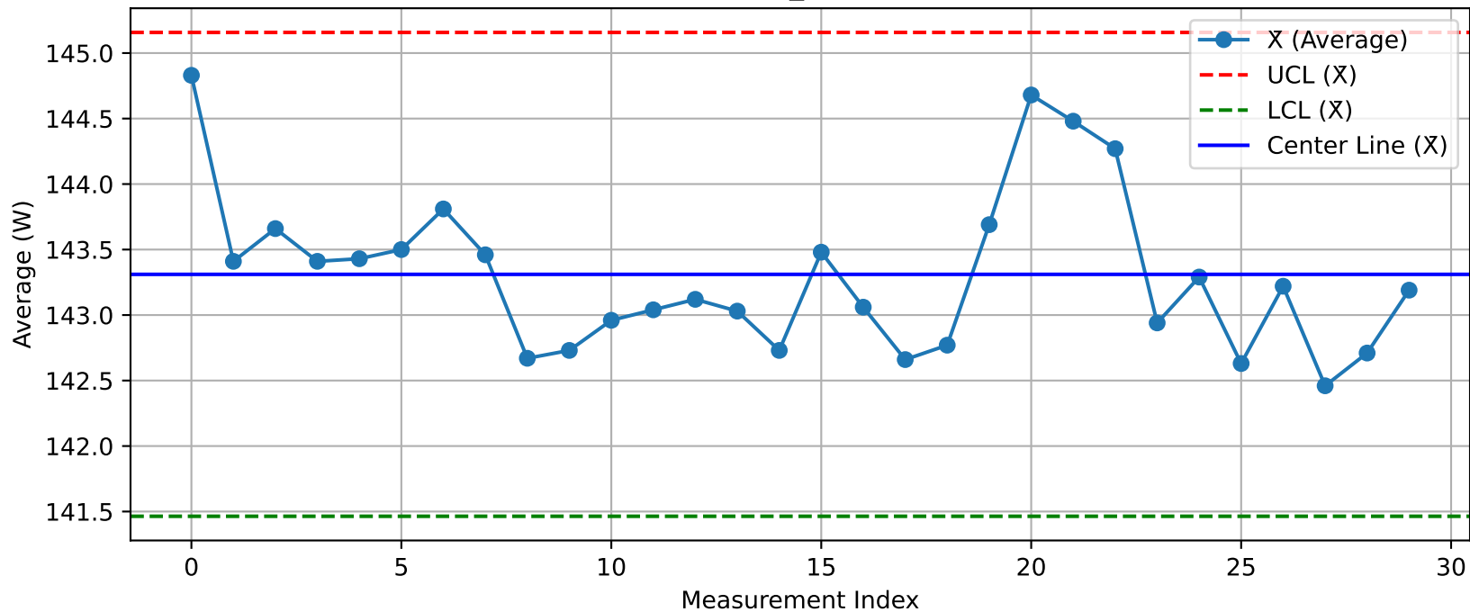
DUT - \bar{X} Chart (T51_Test200@Test.xlsx)
