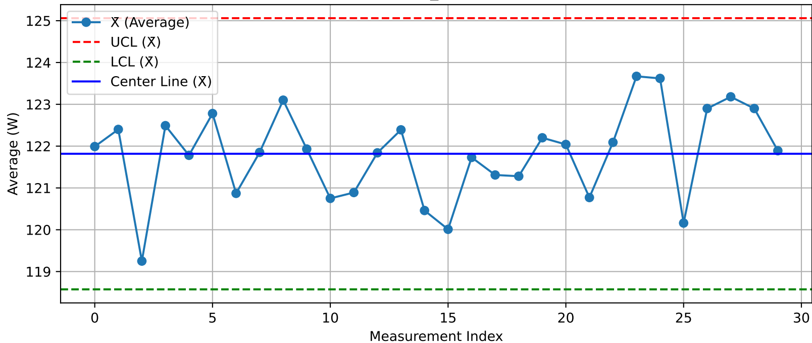
DUT - \bar{X} Chart (T20_Test203@Test.xlsx)
