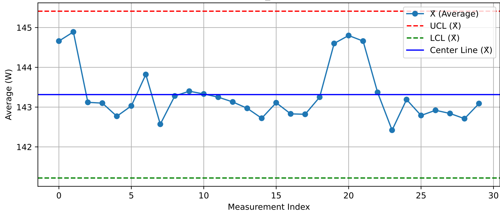
DUT - \bar{X} Chart (T51_Test100@Test.xlsx)
