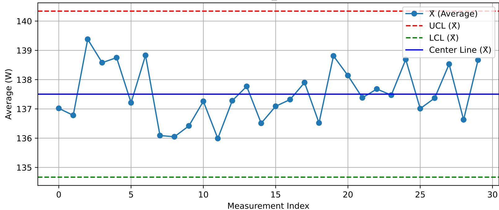
DUT - \bar{X} Chart (T17_Test1@Test.xlsx)
