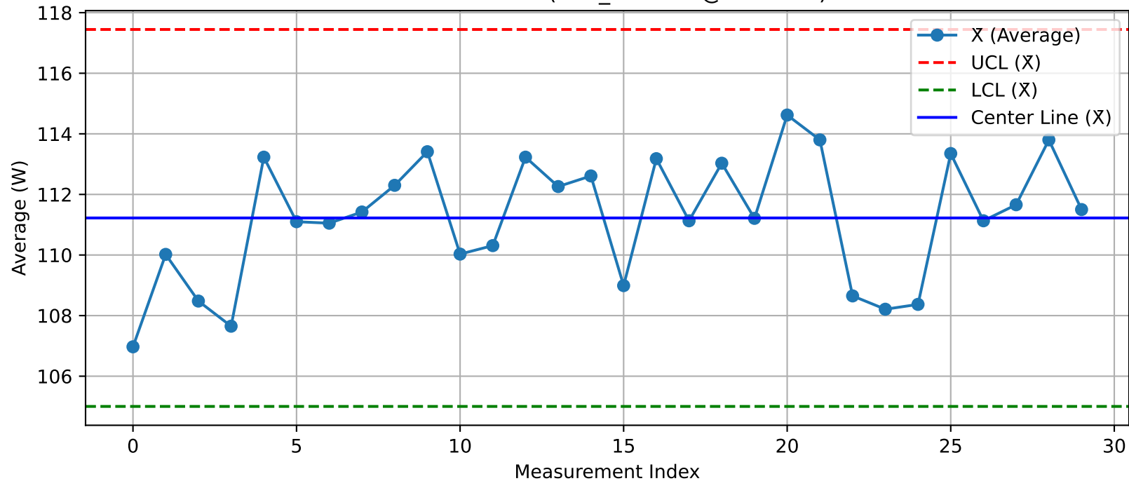
DUT - \bar{X} Chart (T17_Test100@Test.xlsx)
