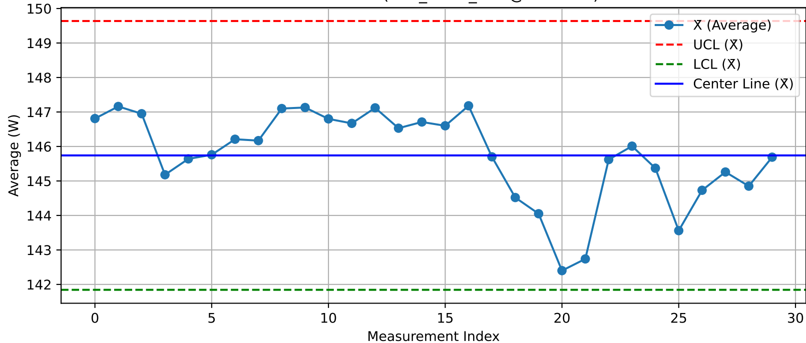
DUT - \bar{X} Chart (T31_Test2_Xint@Test.xlsx)
