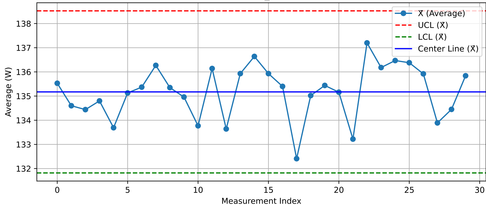
DUT - \bar{X} Chart (T44_Test2@Test.xlsx)
