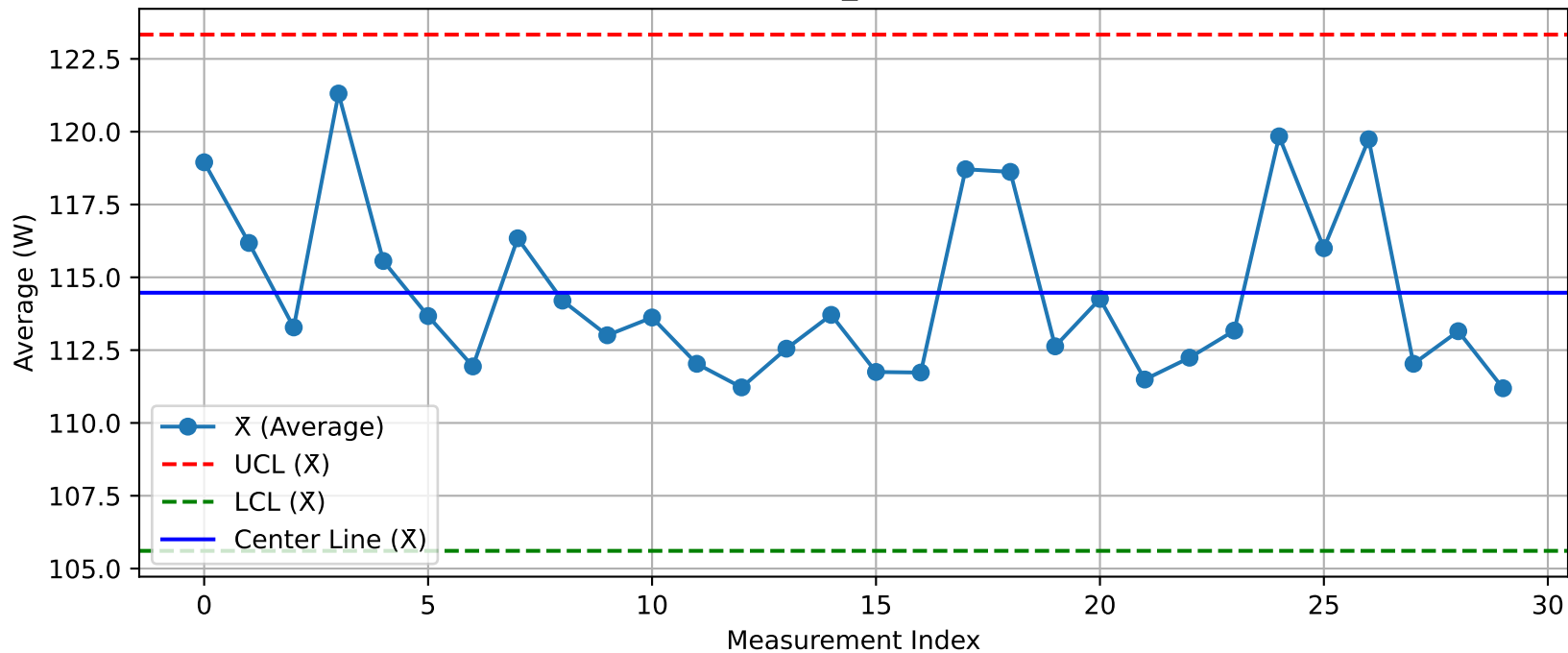
DUT - \bar{X} Chart (T28_Test203@Test.xlsx)
