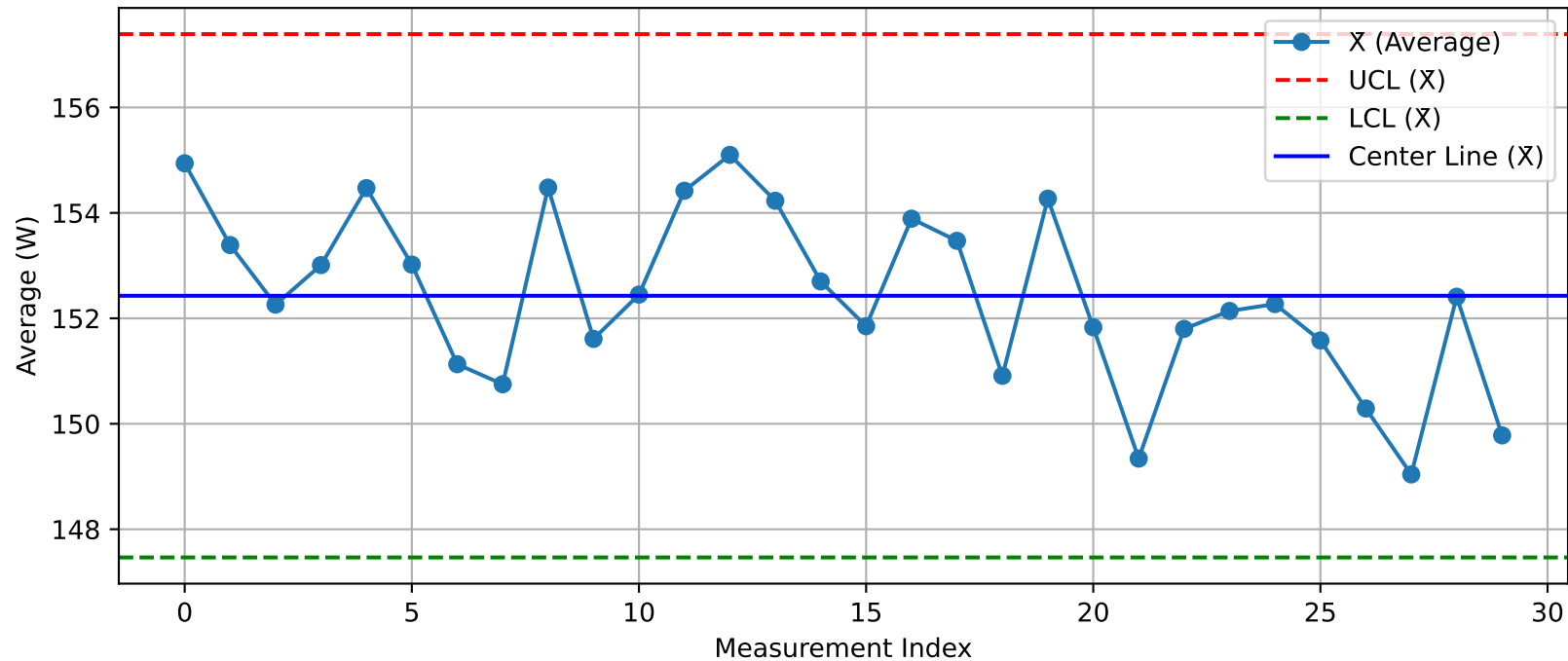
DUT - \bar{X} Chart (T19_Test1_Nuitka@Test.xlsx)
