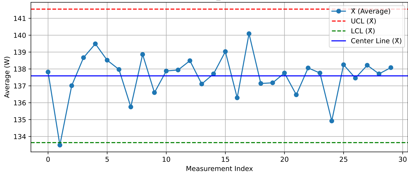
DUT - \bar{X} Chart (T20_Test200@Test.xlsx)
