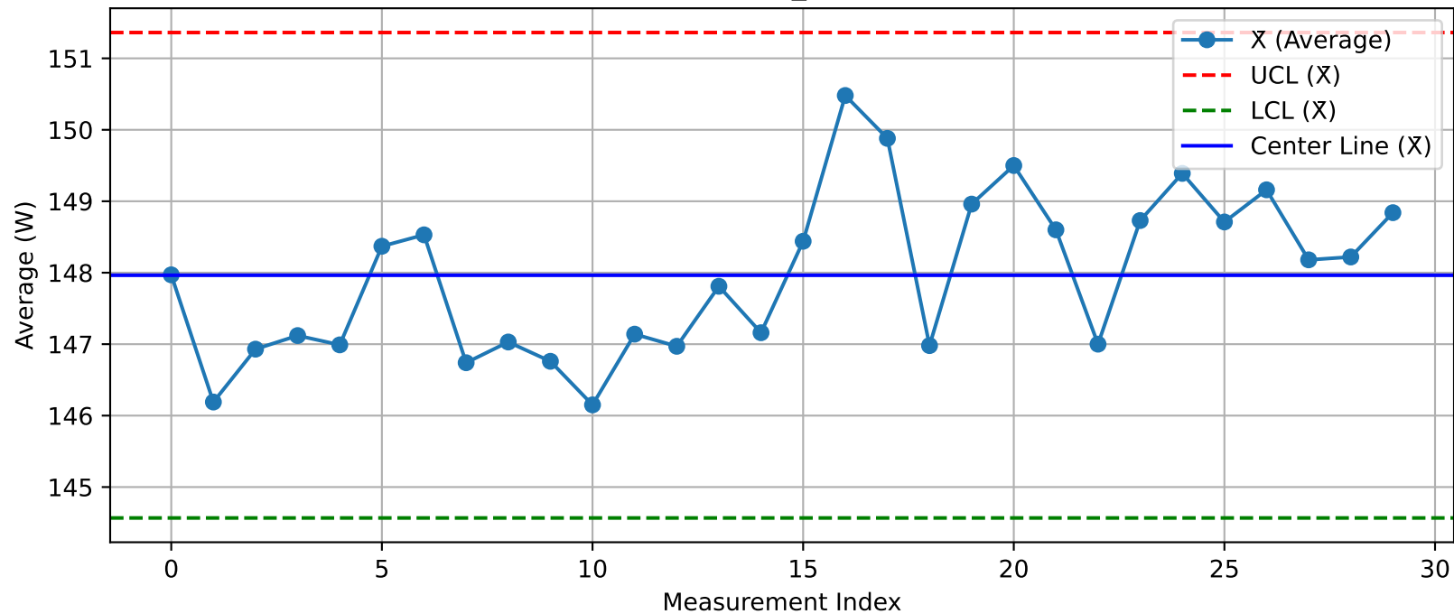
DUT - \bar{X} Chart (T12_Test2@Test.xlsx)
