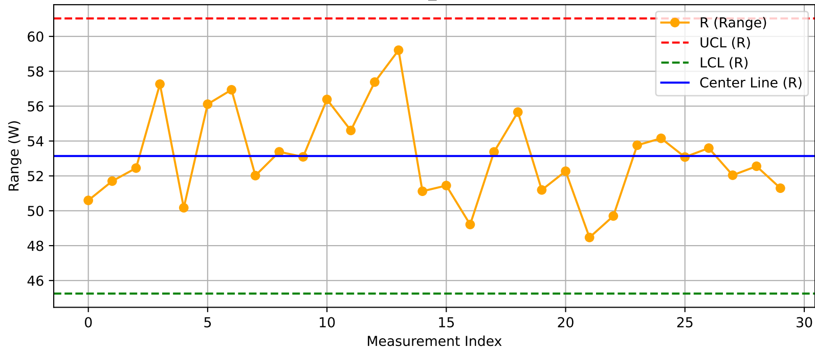
DUT - R Chart (T08_Test2O3@Test.xlsx)
