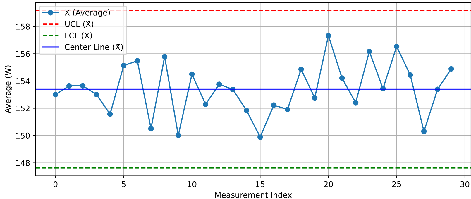
DUT - \bar{X} Chart (T17_Test2_Nuitka@Test.xlsx)
