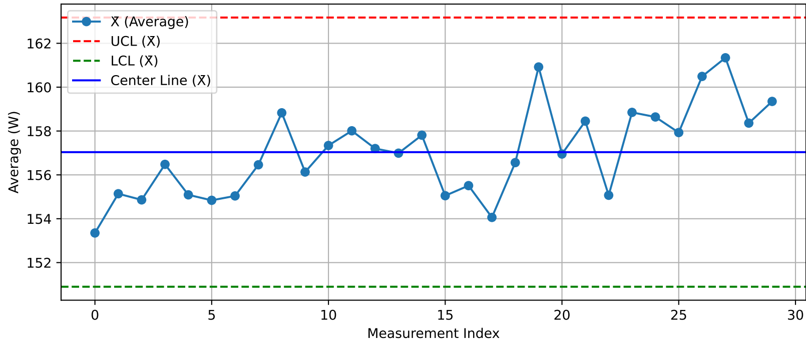
DUT - \bar{X} Chart (T51_Test1@Test.xlsx)
