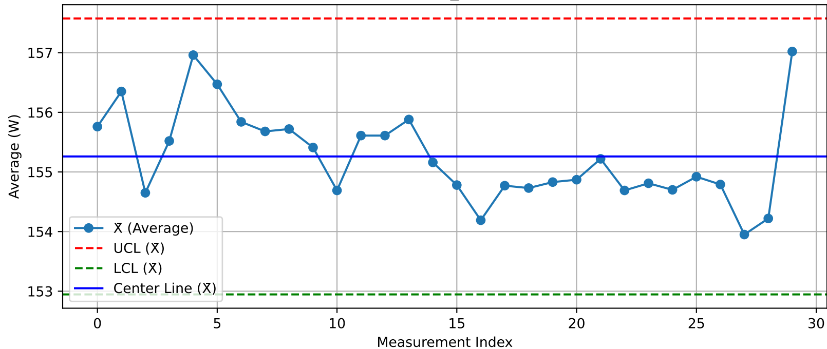
DUT - \bar{X} Chart (T13_Test1@Test.xlsx)
