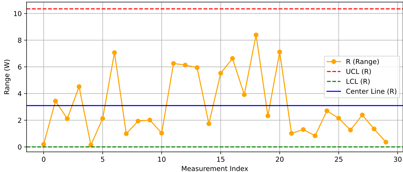
DUT - R Chart (T50_Test203@Test.xlsx)
