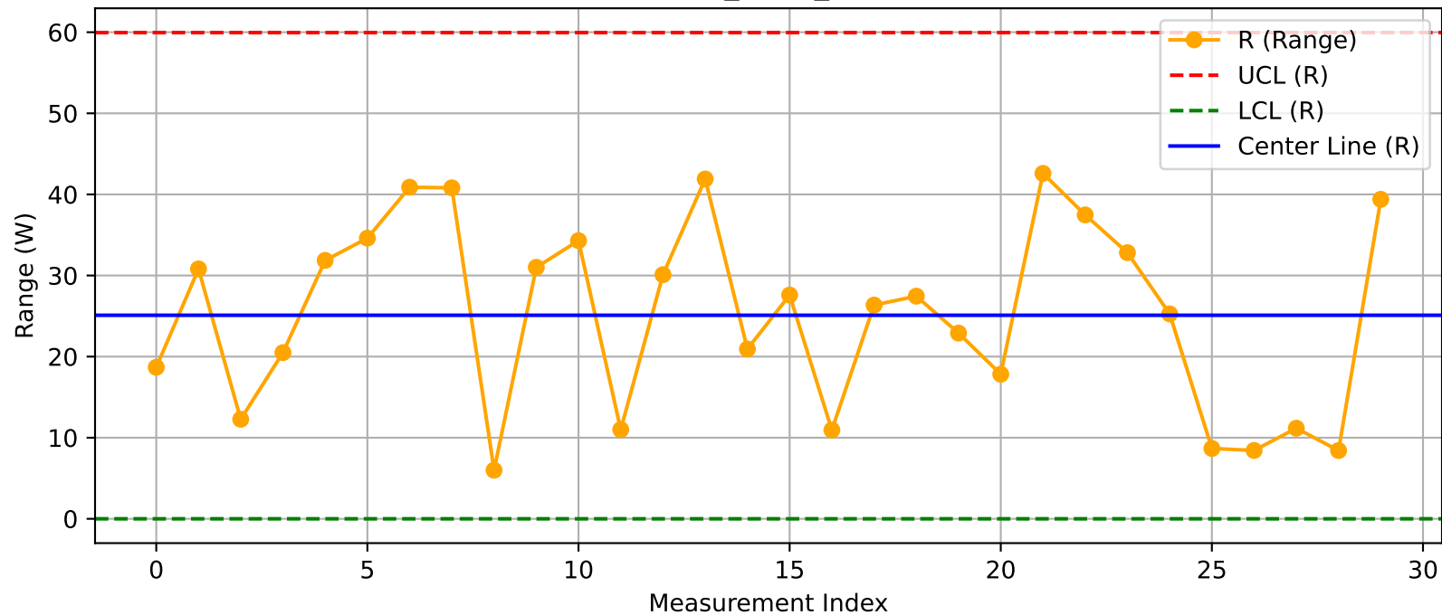
DUT - R Chart (T32_Test1_Nuitka@Test.xlsx)
