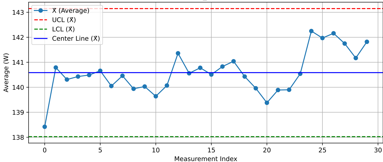
DUT - \bar{X} Chart (T50_Test200@Test.xlsx)
