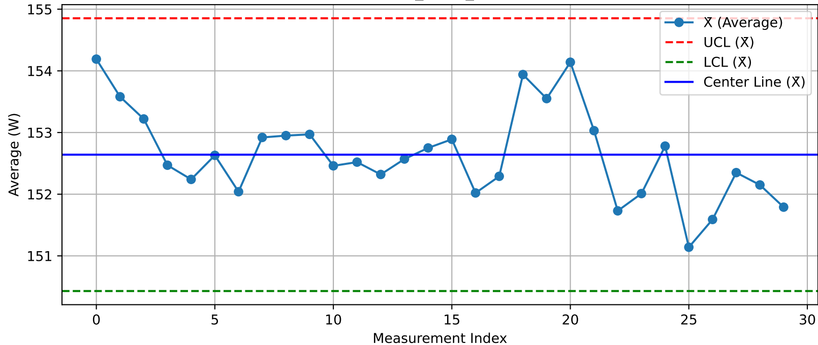
DUT - \bar{X} Chart (T31_Test1_Nuitka@Test.xlsx)
