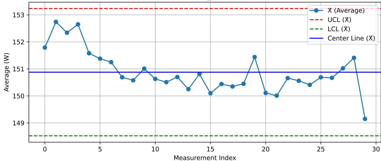
DUT - \bar{X} Chart (T40_Test1@Test.xlsx)
