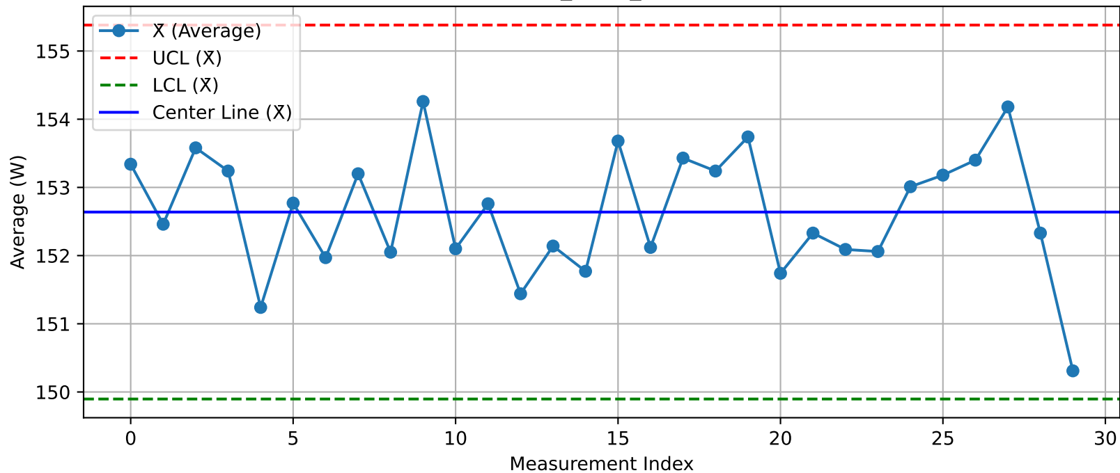
DUT - \bar{X} Chart (T8_Test2_Nuitka@Test.xlsx)
