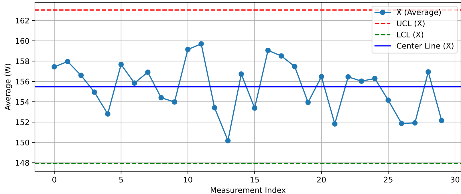
DUT - \bar{X} Chart (T29_Test2_Nuitka@Test.xlsx)
