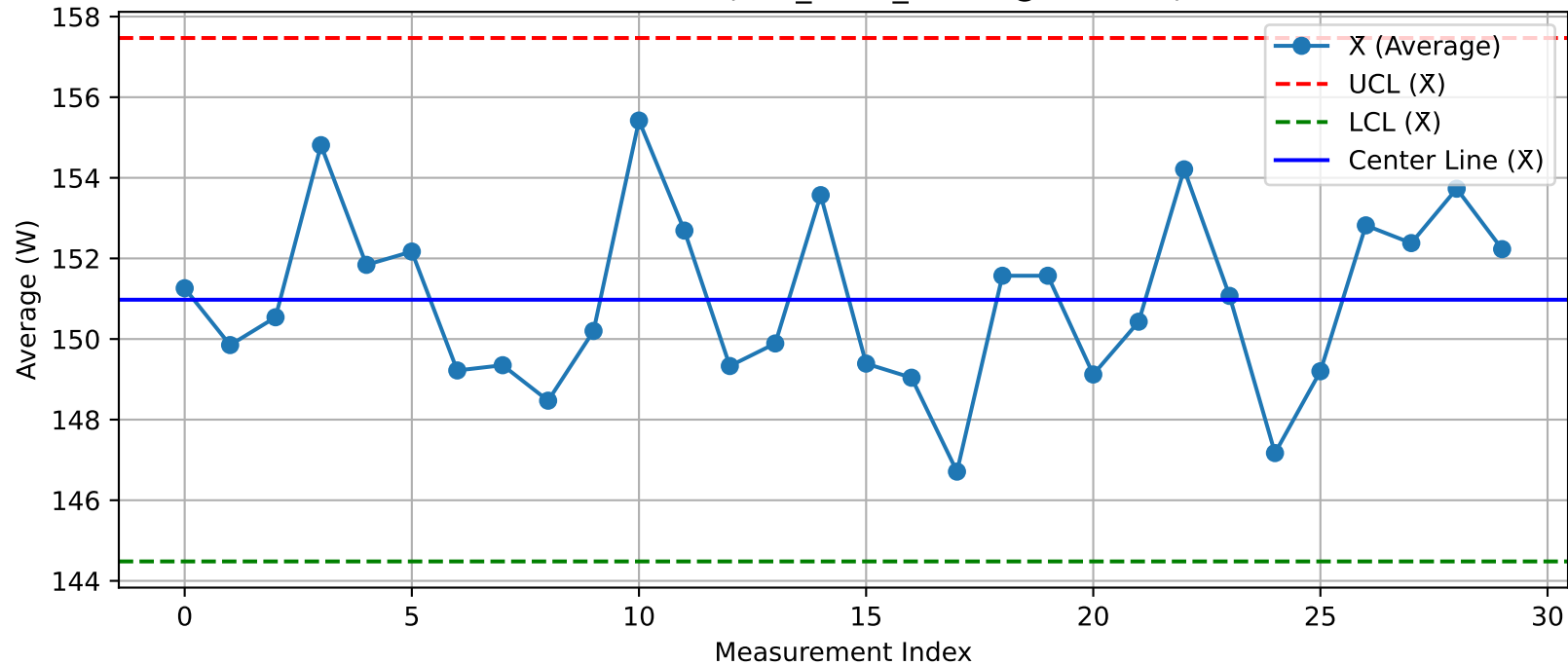
DUT - \bar{X} Chart (T16_Test2_Nuitka@Test.xlsx)
