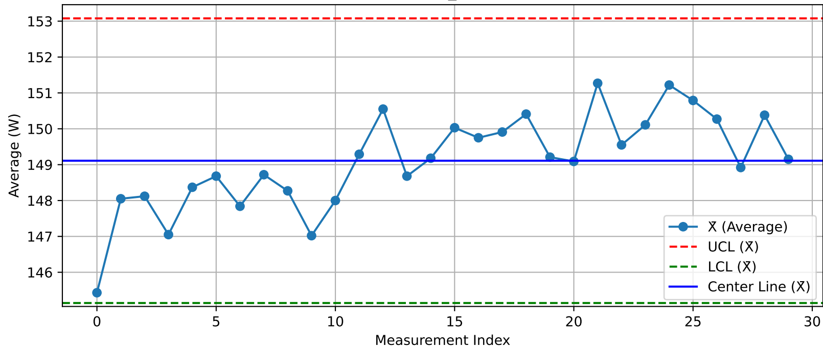
DUT - \bar{X} Chart (T36_Test1@Test.xlsx)
