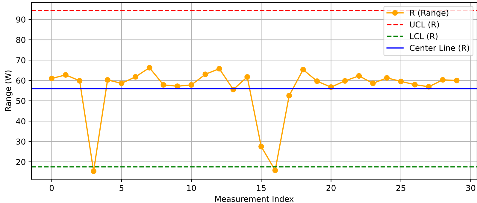
DUT - R Chart (T49_Test1_Nuitka@Test.xlsx)
