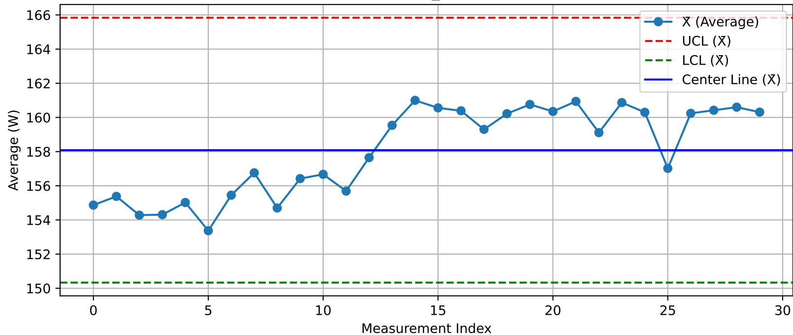
DUT - \bar{X} Chart (T20_Test2@Test.xlsx)
