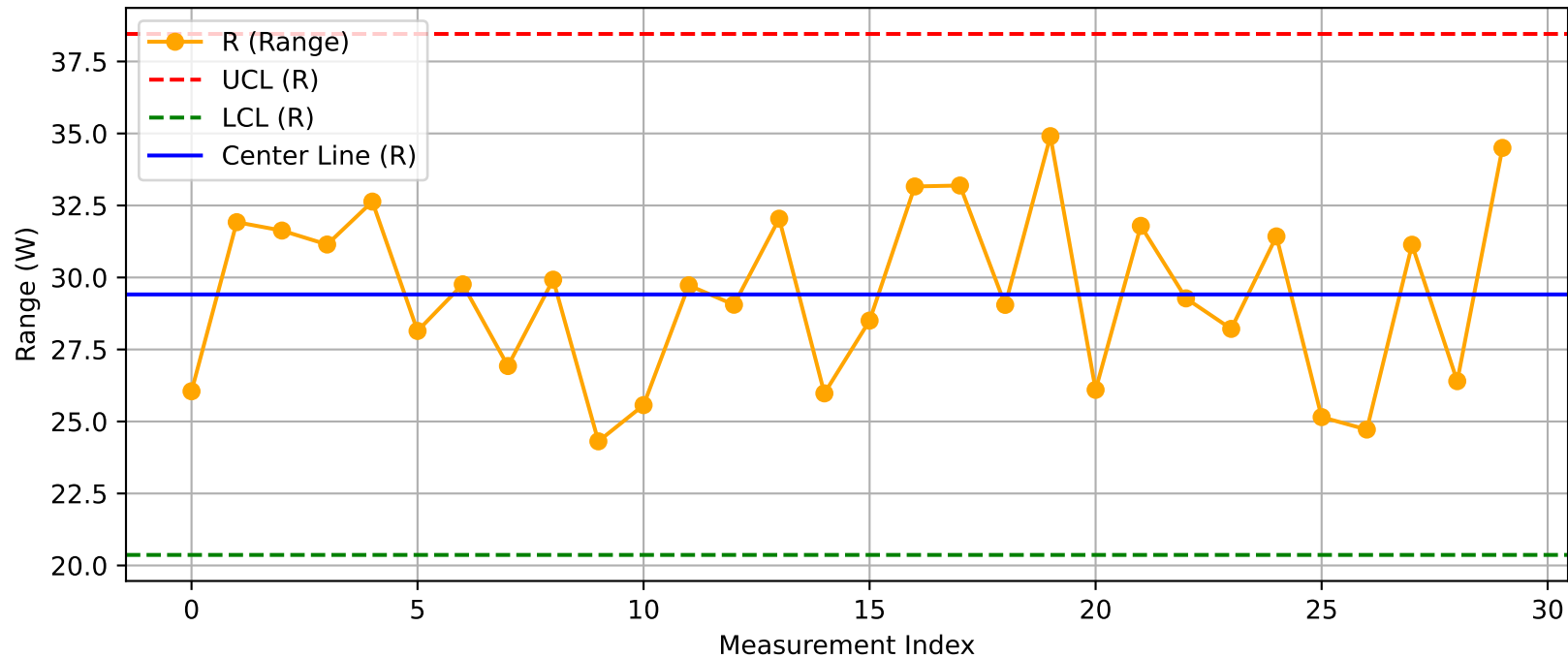
DUT - R Chart (T16_Test100@Test.xlsx)
