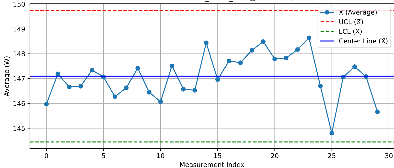
DUT - \bar{X} Chart (T50_Test1_Xint@Test.xlsx)
