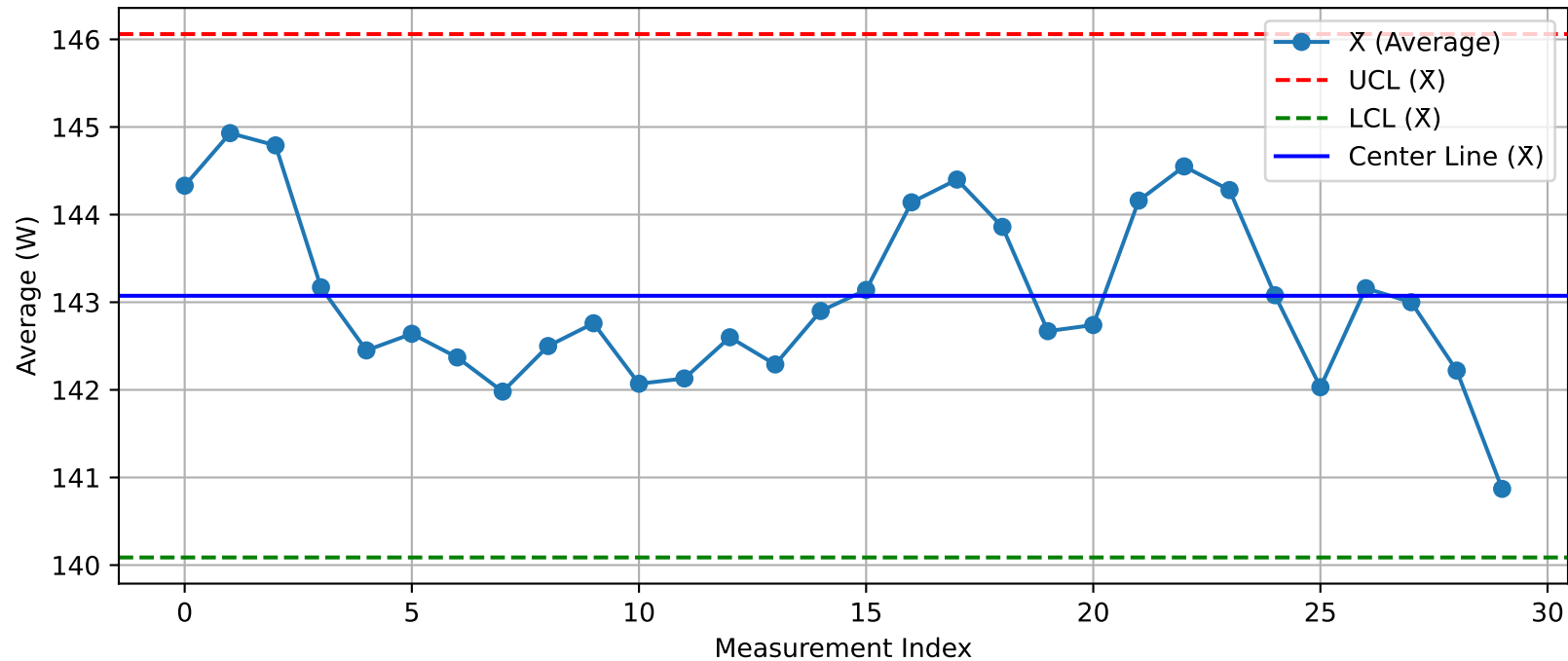
DUT - \bar{X} Chart (T51_Test2_Xint@Test.xlsx)
