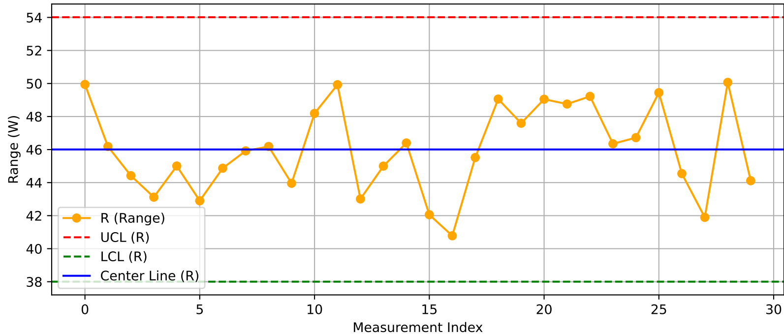
DUT - R Chart (T13_Test2O3@Test.xlsx)
