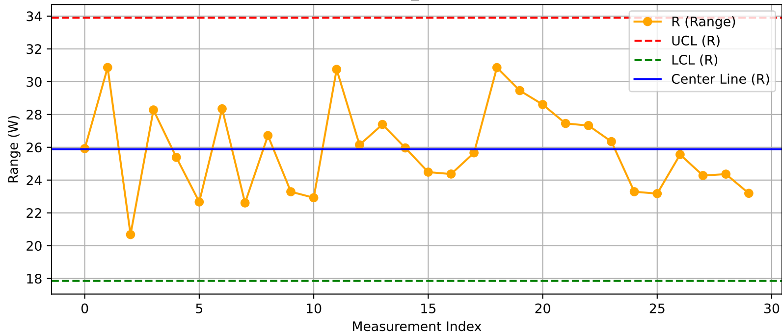
DUT - R Chart (T11_Test203@Test.xlsx)
