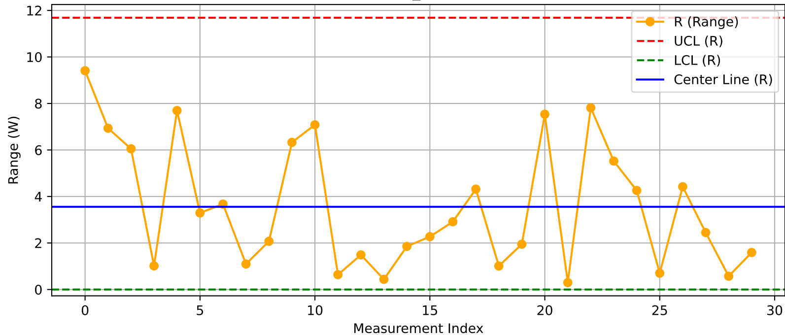
DUT - R Chart (T44_Test100@Test.xlsx)
