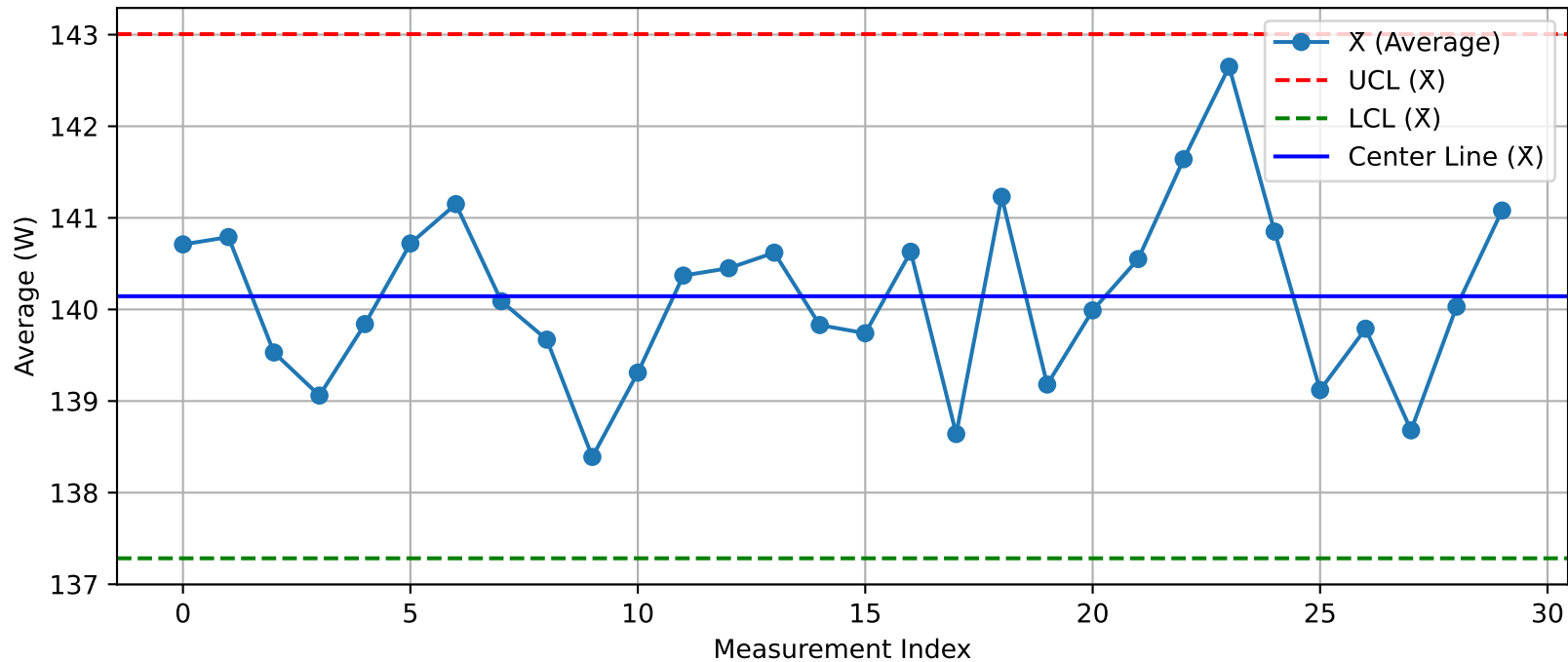
DUT - \bar{X} Chart (T9_Test2@Test.xlsx)
