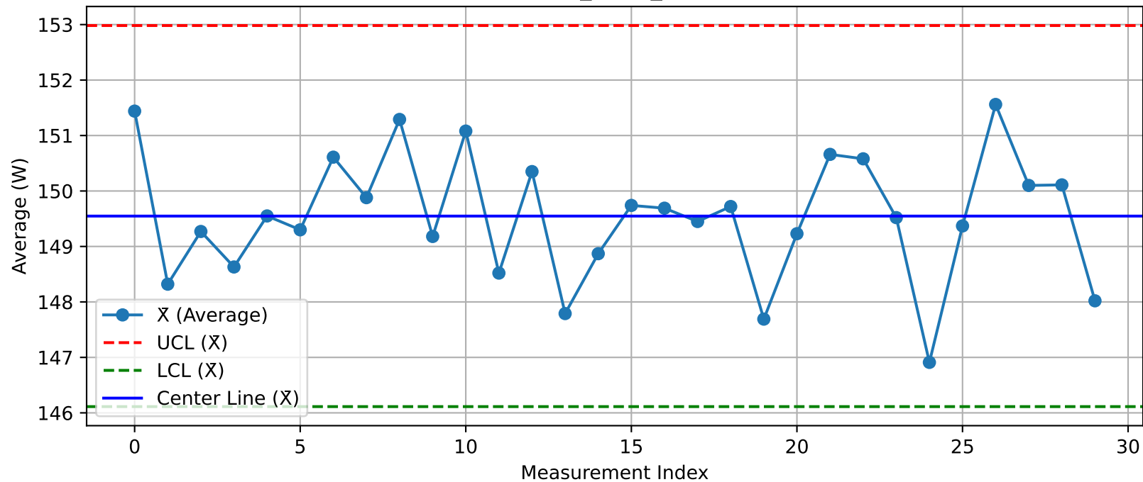
DUT - \bar{X} Chart (T25_Test2_Nuitka@Test.xlsx)
