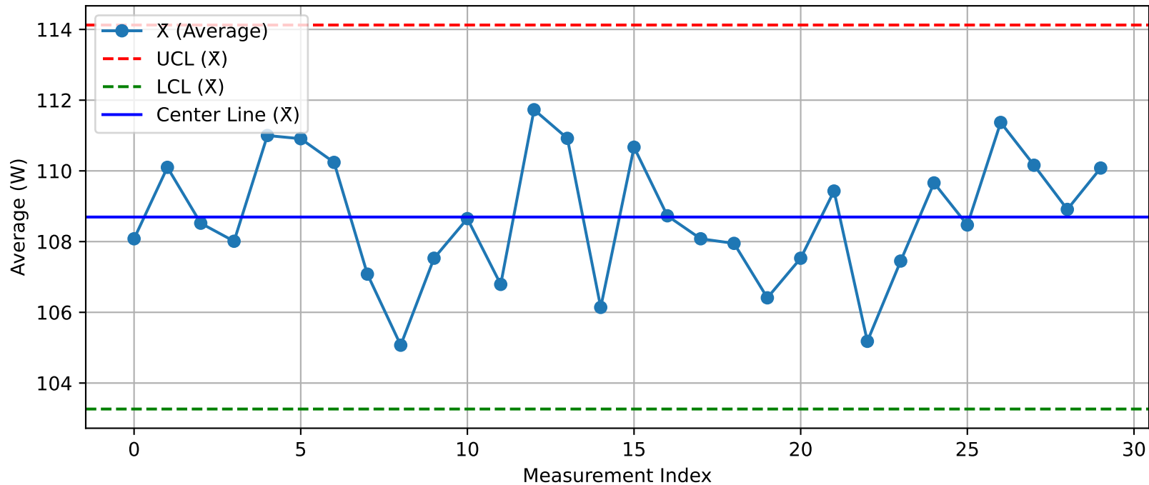
DUT - \bar{X} Chart (T16_Test103@Test.xlsx)
