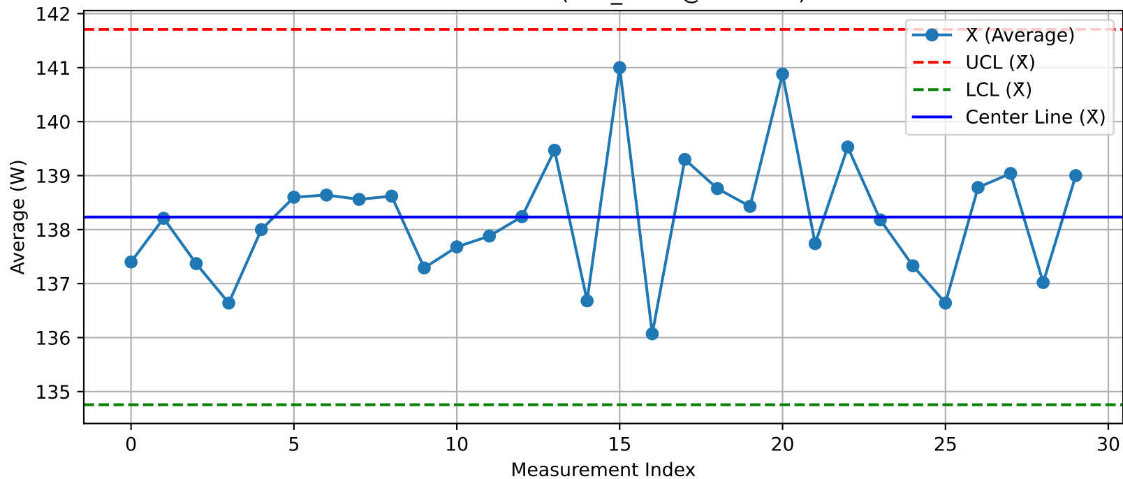
DUT - \bar{X} Chart (T12_Test2@Test.xlsx)
