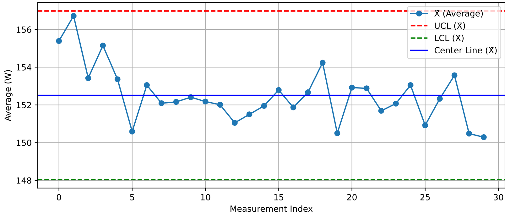
DUT - \bar{X} Chart (T7_Test2_Nuitka@Test.xlsx)
