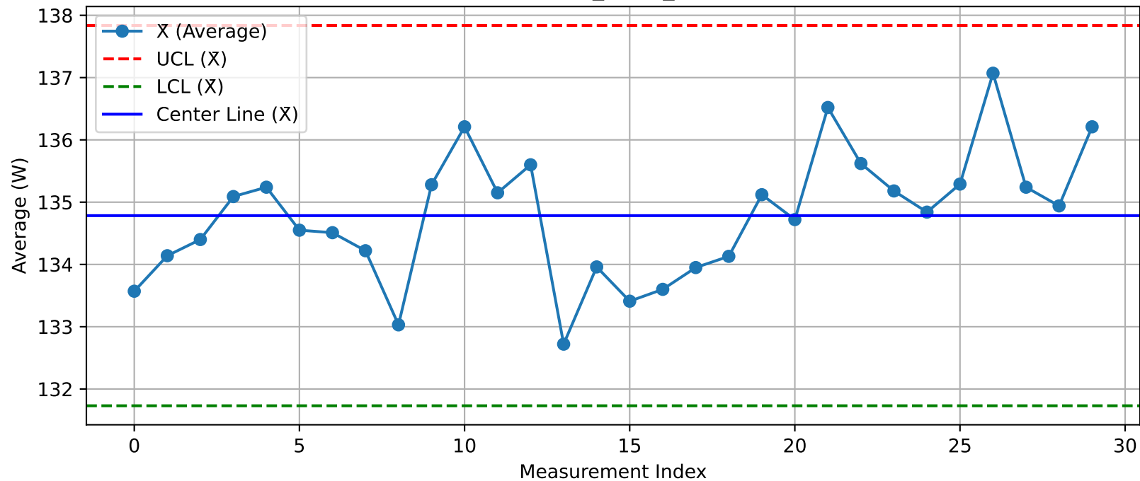
DUT - \bar{X} Chart (T13_Test2_Xint@Test.xlsx)
