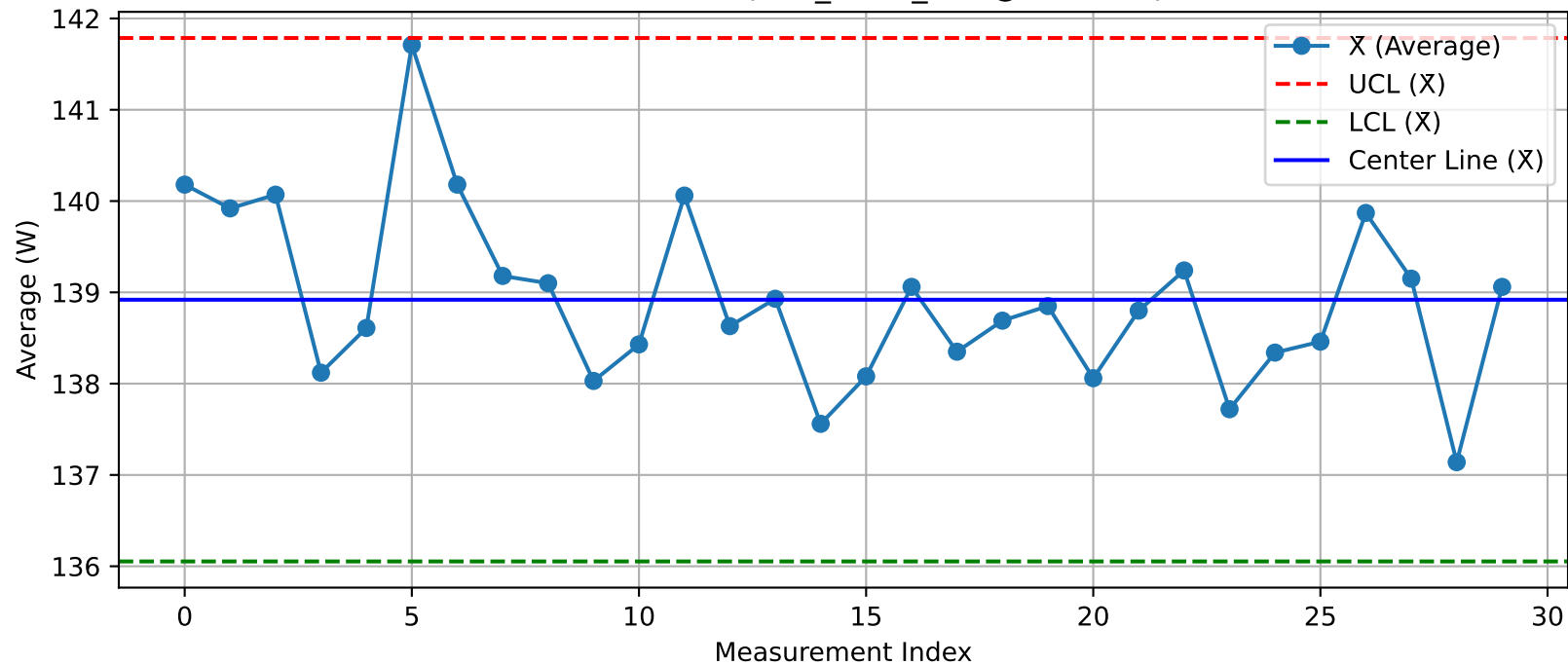
DUT - \bar{X} Chart (T40_Test2_Xint@Test.xlsx)
