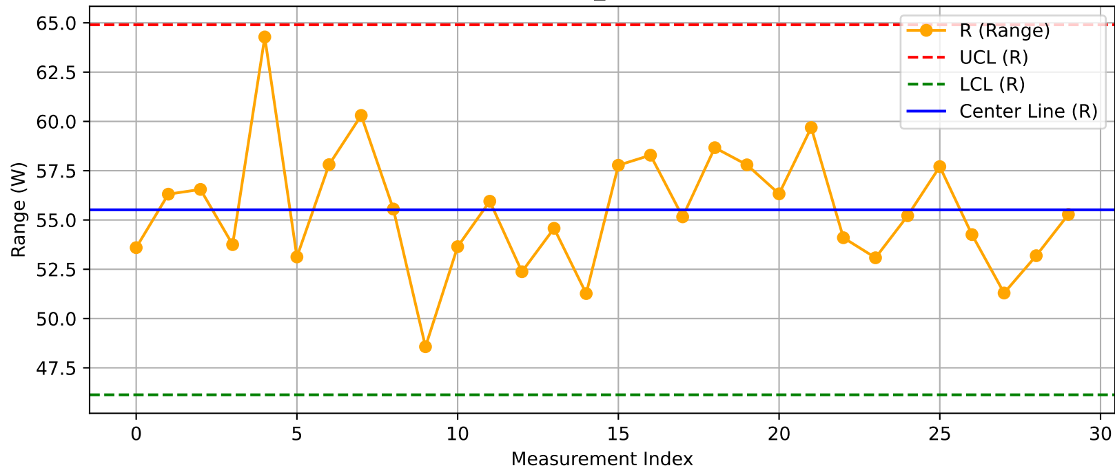
DUT - R Chart (T51_Test100@Test.xlsx)
