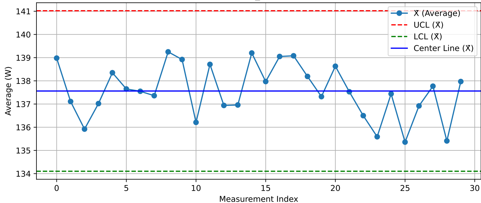
DUT - \bar{X} Chart (T40_Test1O3@Test.xlsx)
