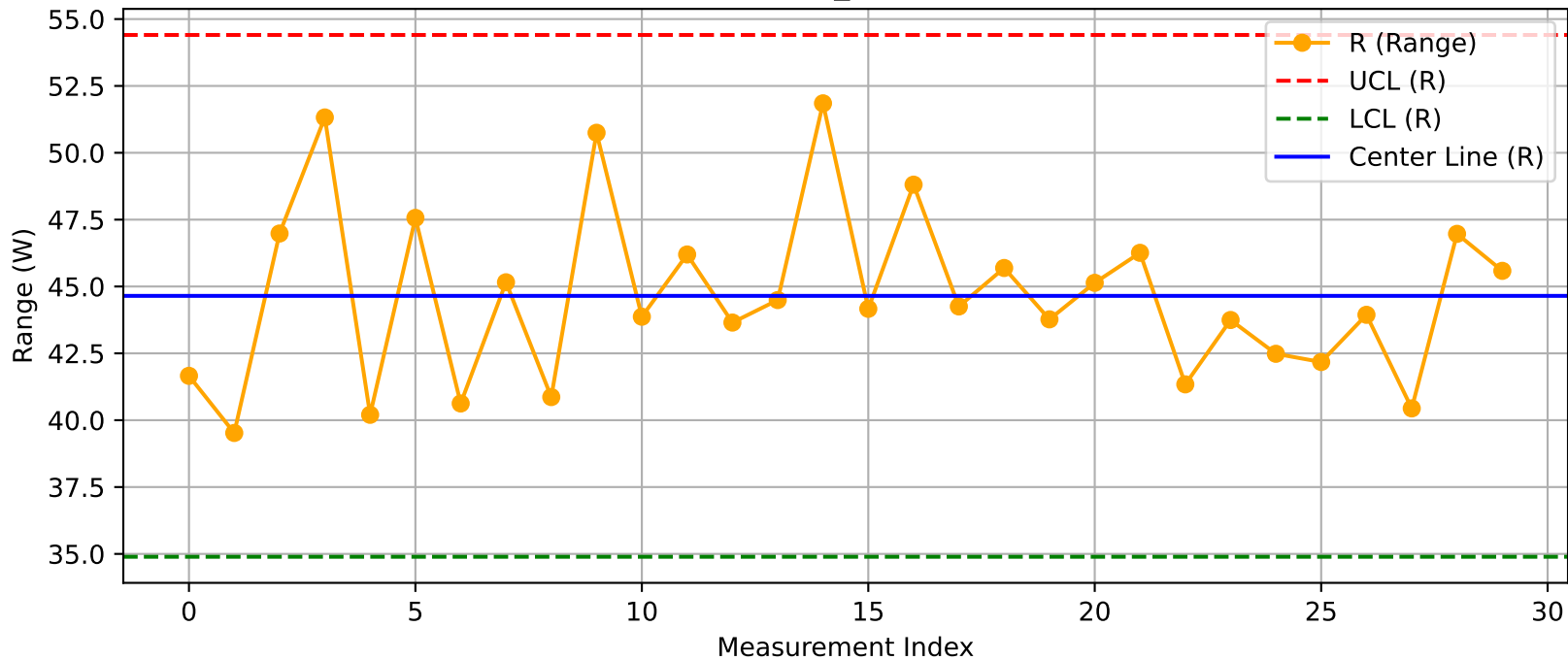
DUT - R Chart (T40_Test103@Test.xlsx)
