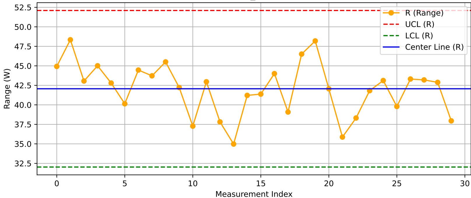
DUT - R Chart (T28_Test103@Test.xlsx)
