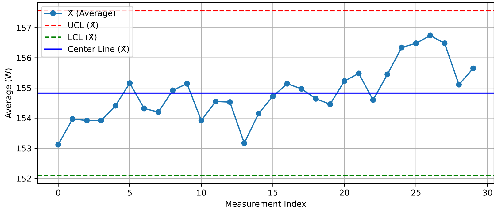
DUT - \bar{X} Chart (T50_Test1@Test.xlsx)
