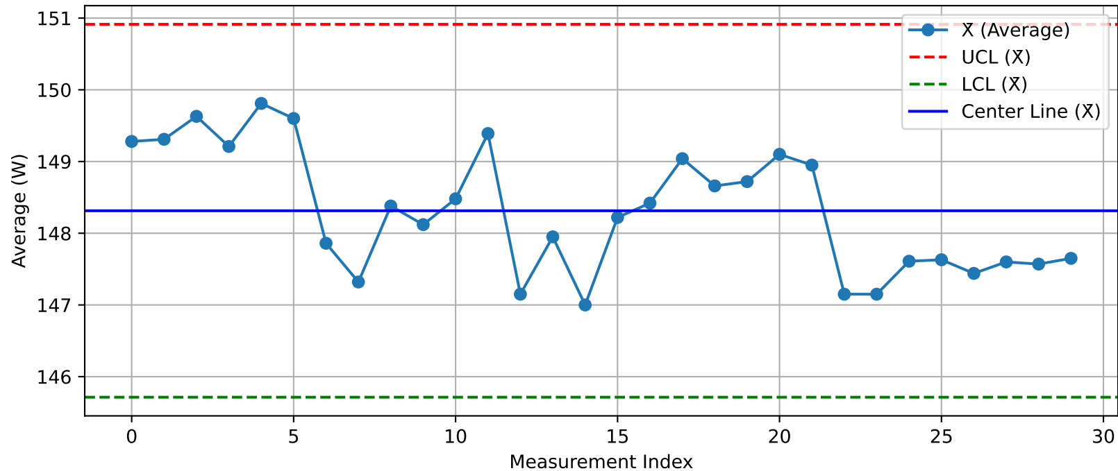
DUT - \bar{X} Chart (T36_Test1_Nuitka@Test.xlsx)
