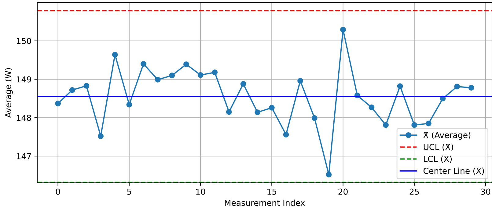
DUT - \bar{X} Chart (T28_Test1_Nuitka@Test.xlsx)
