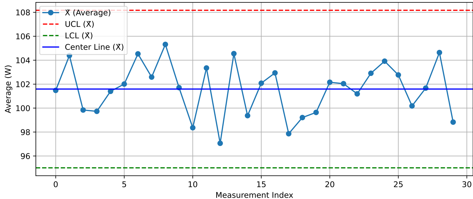
DUT - \bar{X} Chart (T29_Test103@Test.xlsx)
