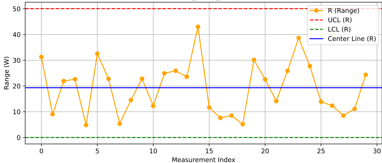
DUT - R Chart (T16_Test1_Nuitka@Test.xlsx)
