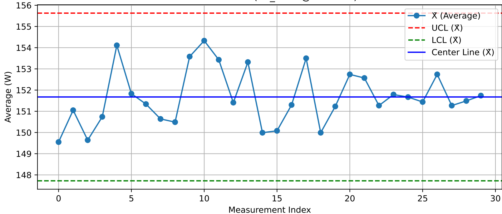
DUT - \bar{X} Chart (T5_Test1@Test.xlsx)
