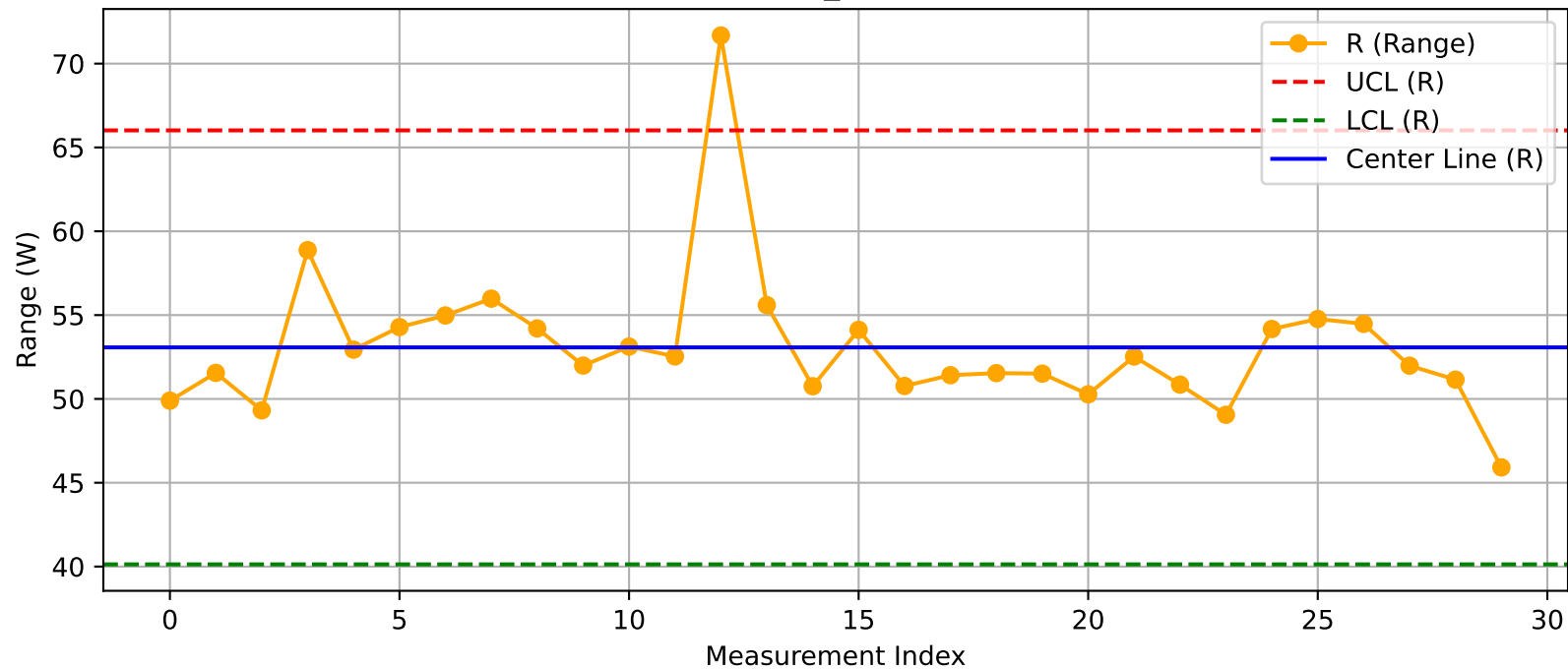
DUT - R Chart (T50_Test100@Test.xlsx)
