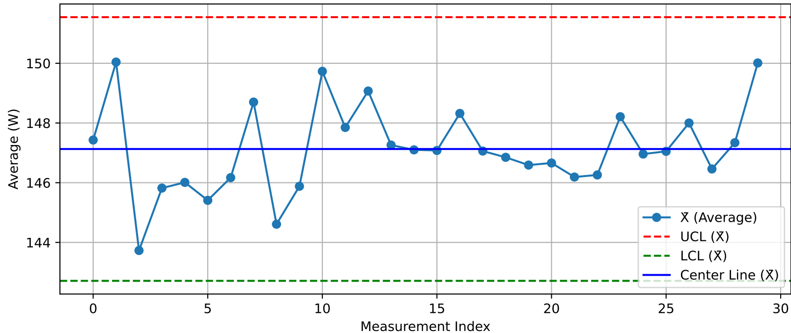
DUT - \bar{X} Chart (T12_Test2_Nuitka@Test.xlsx)
