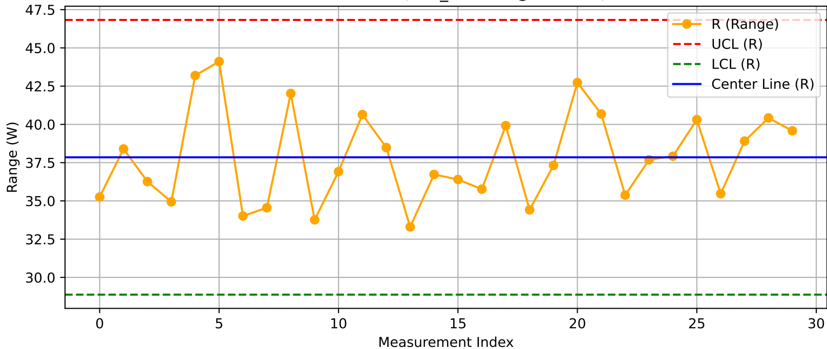
DUT - R Chart (T20_Test2O3@Test.xlsx)
