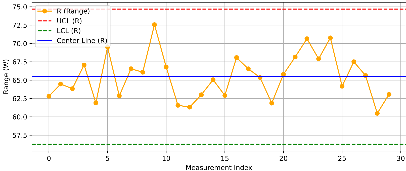
DUT - R Chart (T31_Test203@Test.xlsx)
