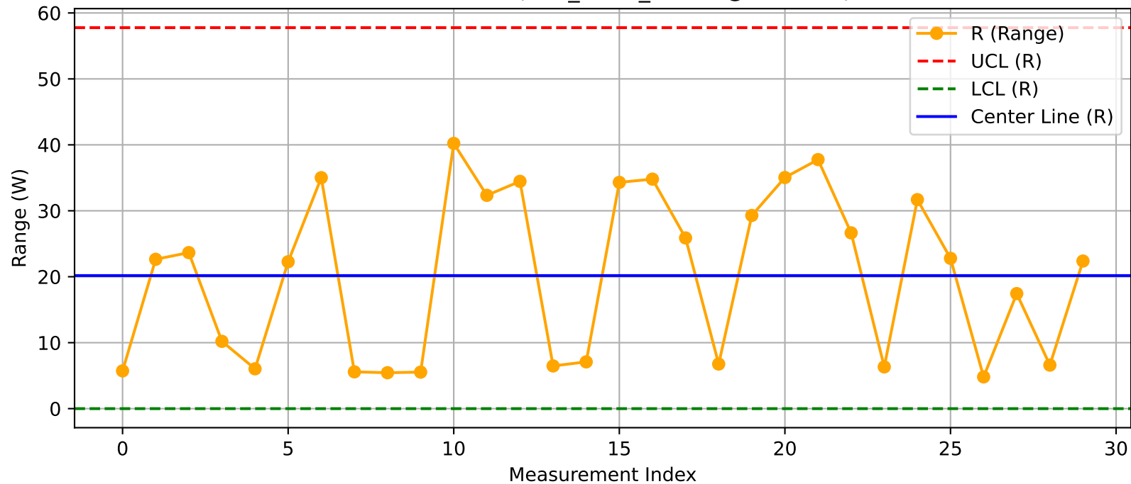
DUT - R Chart (T12_Test1_Nuitka@Test.xlsx)
