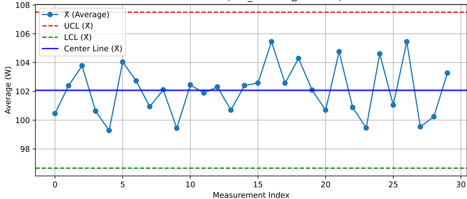
DUT - \bar{X} Chart (T32_Test203@Test.xlsx)
