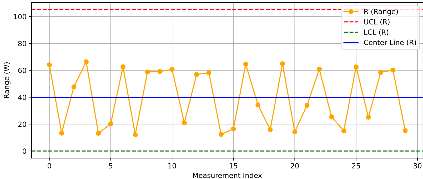
DUT - R Chart (T20_Test2_Nuitka@Test.xlsx)
