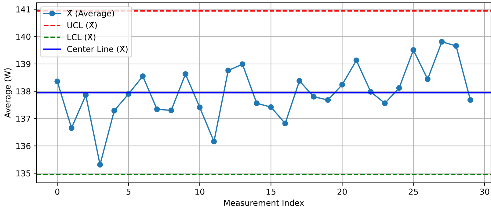
DUT - \bar{X} Chart (T08_Test200@Test.xlsx)
