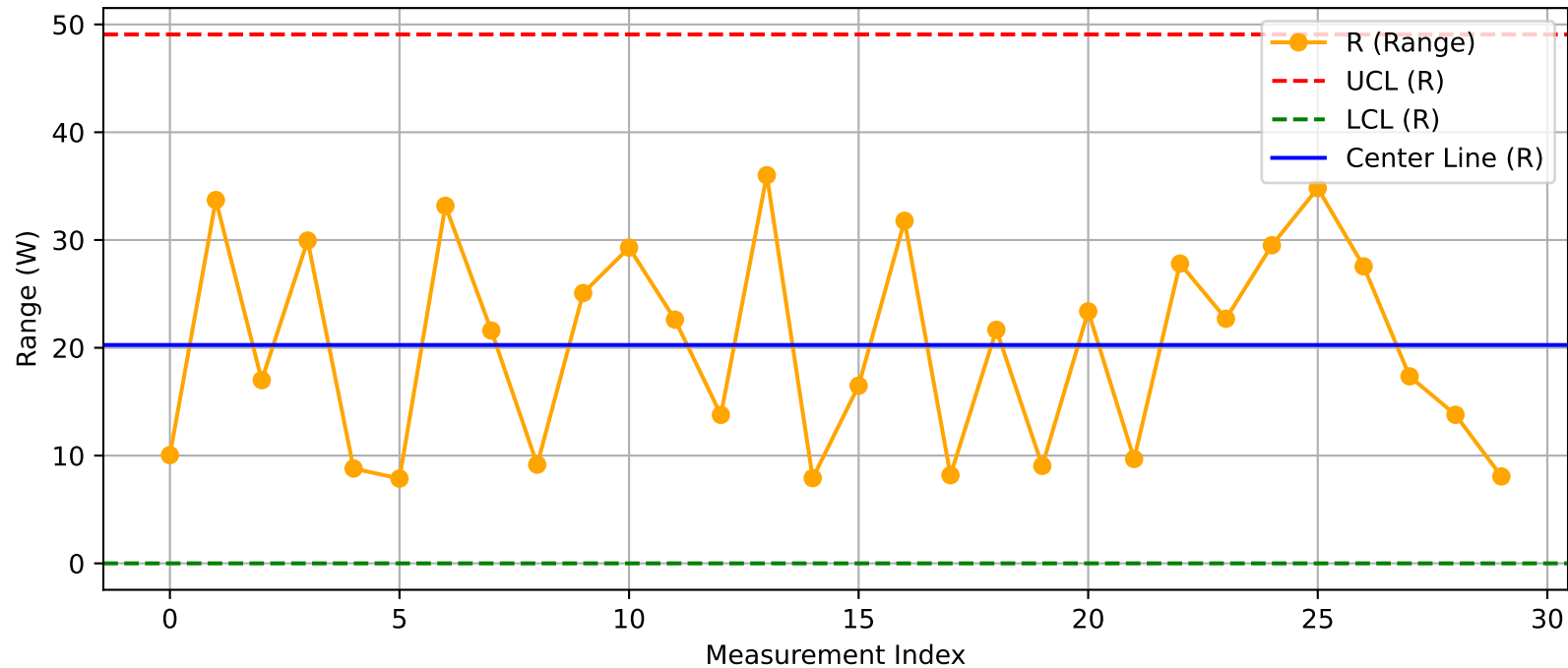
DUT - R Chart (T40_Test1_Xint@Test.xlsx)
