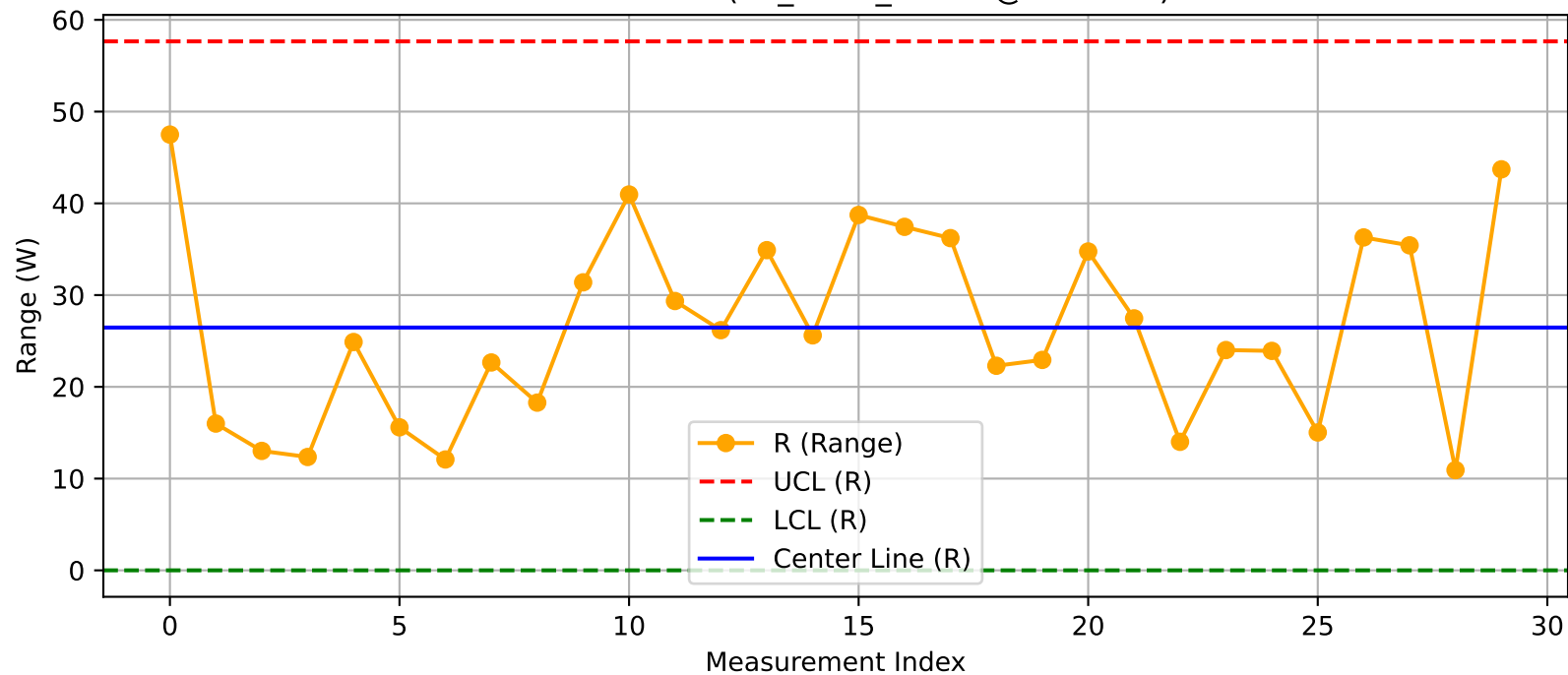
DUT - R Chart (T7_Test1_Nuitka@Test.xlsx)
