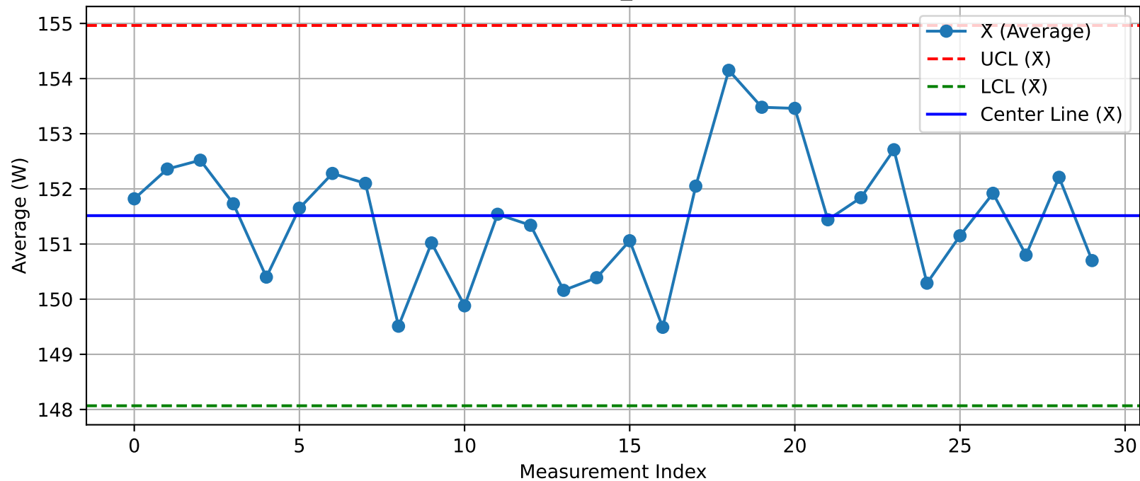
DUT - \bar{X} Chart (T40_Test2@Test.xlsx)
