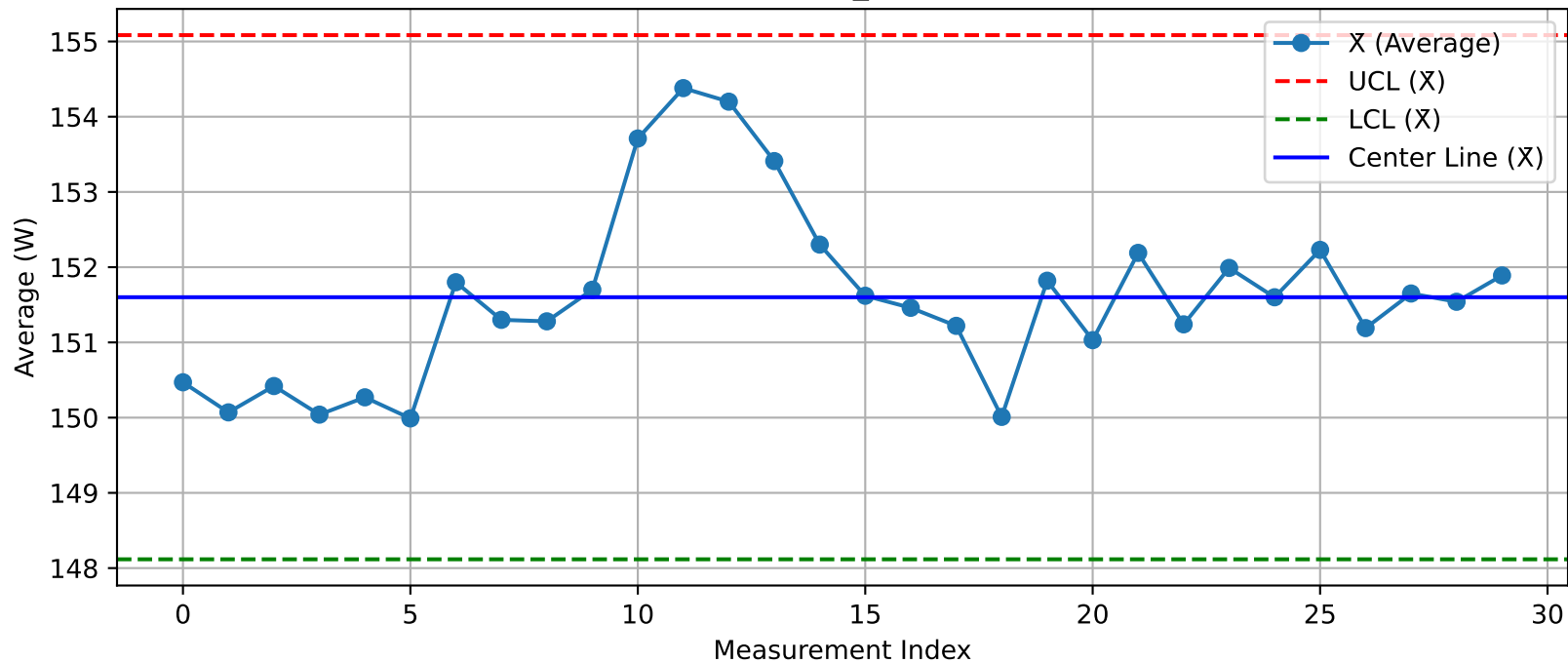
DUT - \bar{X} Chart (T31_Test2@Test.xlsx)
