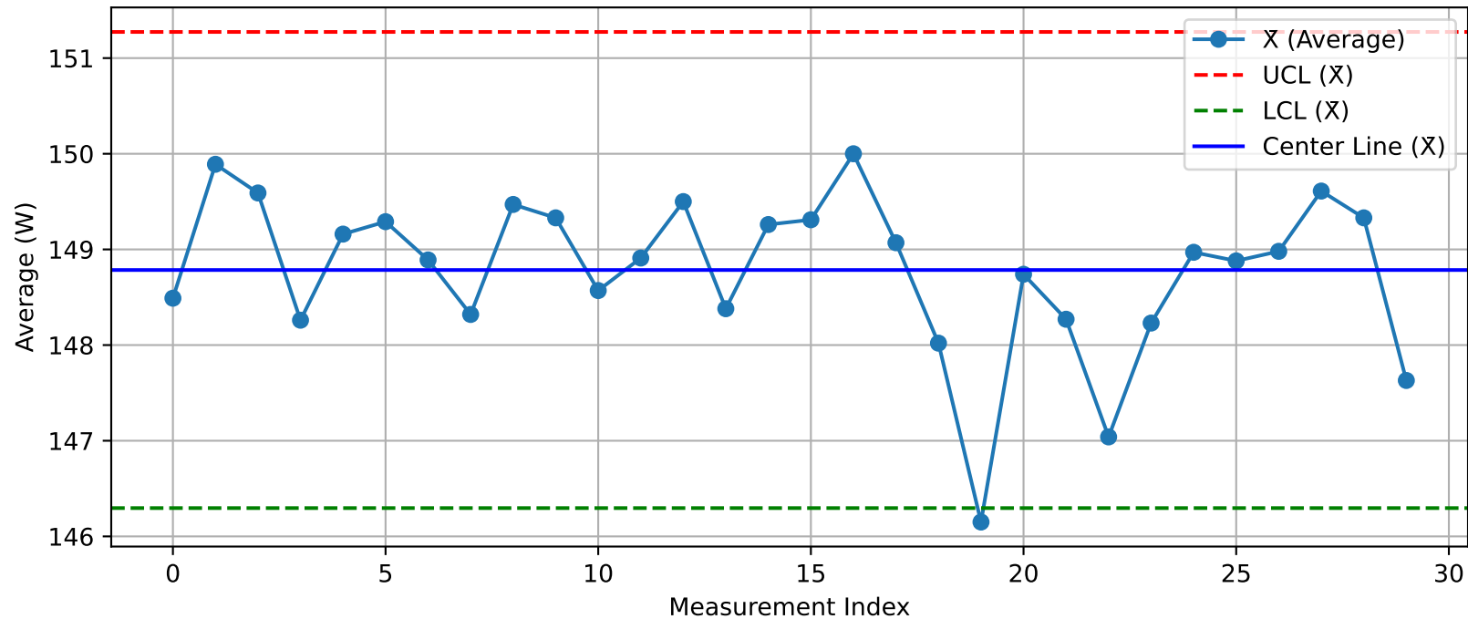
DUT - \bar{X} Chart (T40_Test1_Nuitka@Test.xlsx)
