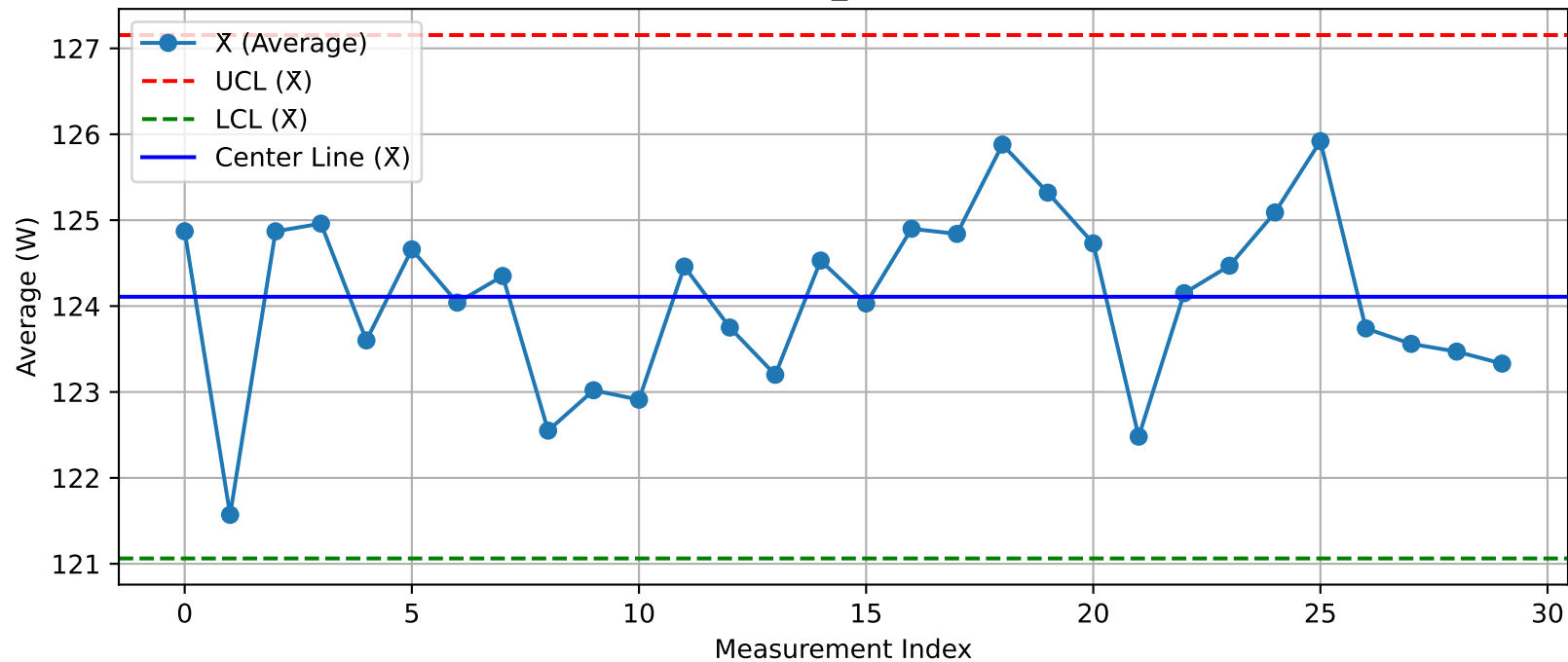
DUT - \bar{X} Chart (T11_Test100@Test.xlsx)
