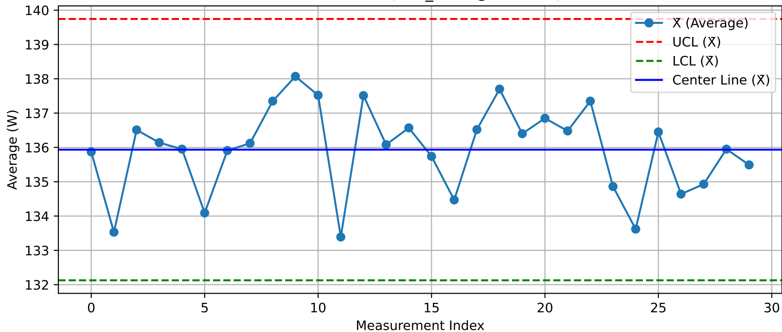
DUT - \bar{X} Chart (T33_Test2@Test.xlsx)
