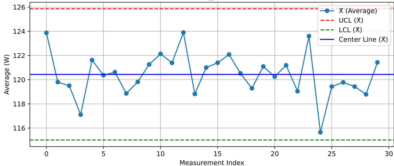
DUT - \bar{X} Chart (T19_Test103@Test.xlsx)
