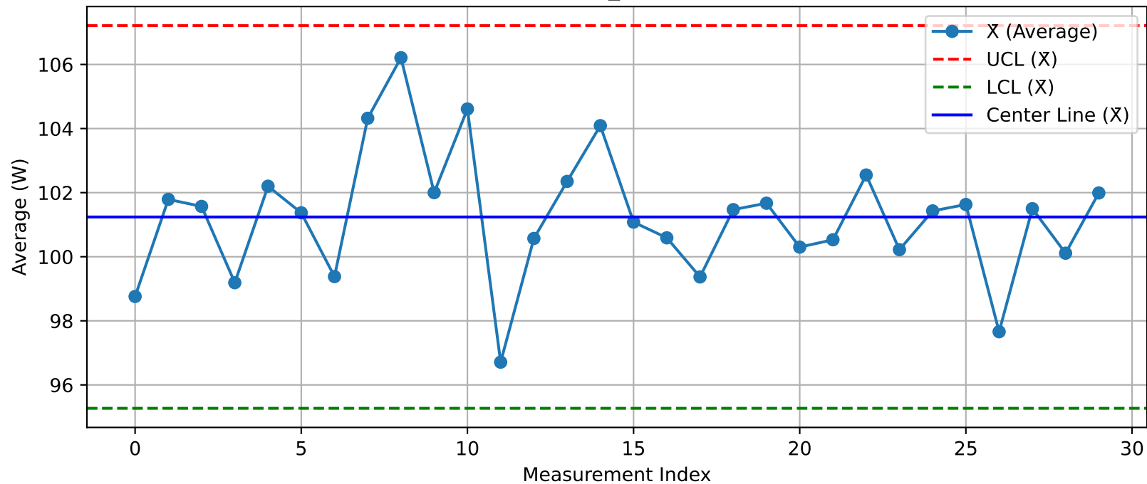
DUT - \bar{X} Chart (T32_Test103@Test.xlsx)
