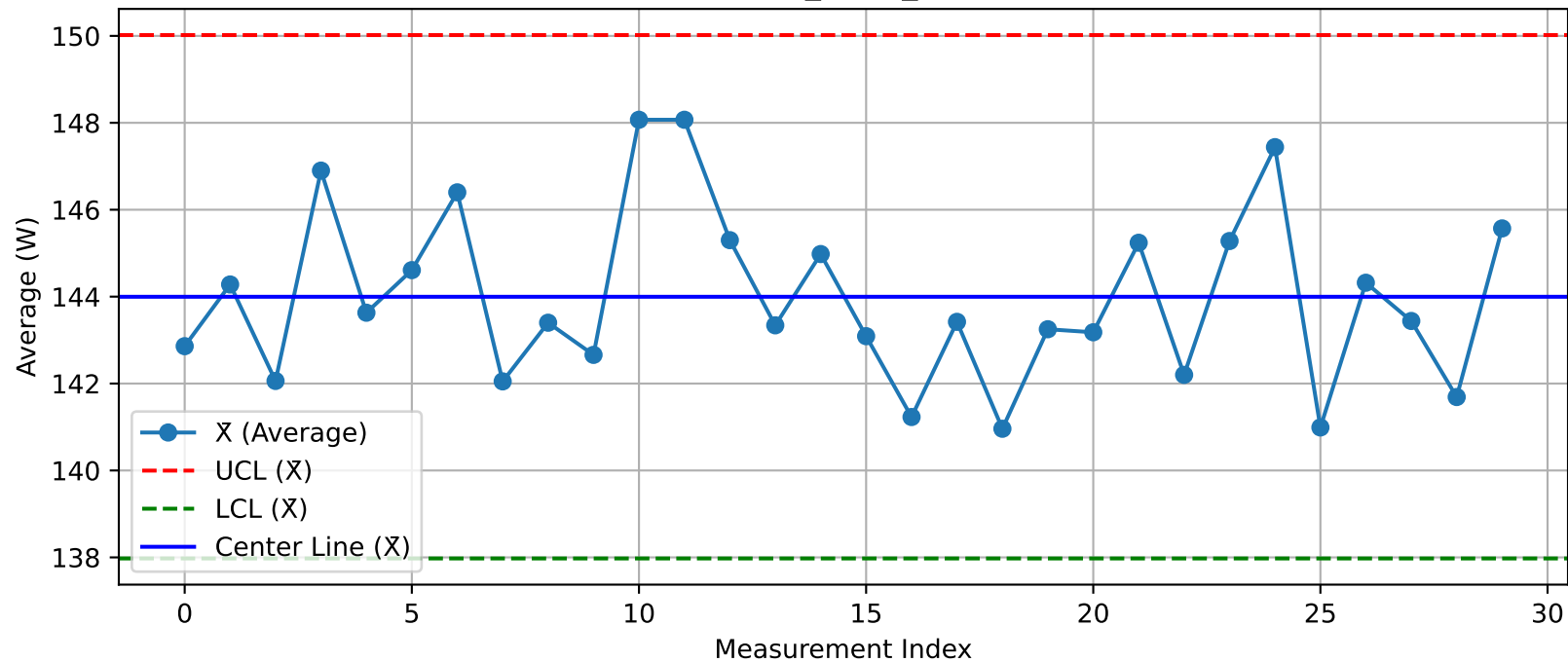
DUT - X Chart (T9_Test1_Xint@Test.xlsx)
