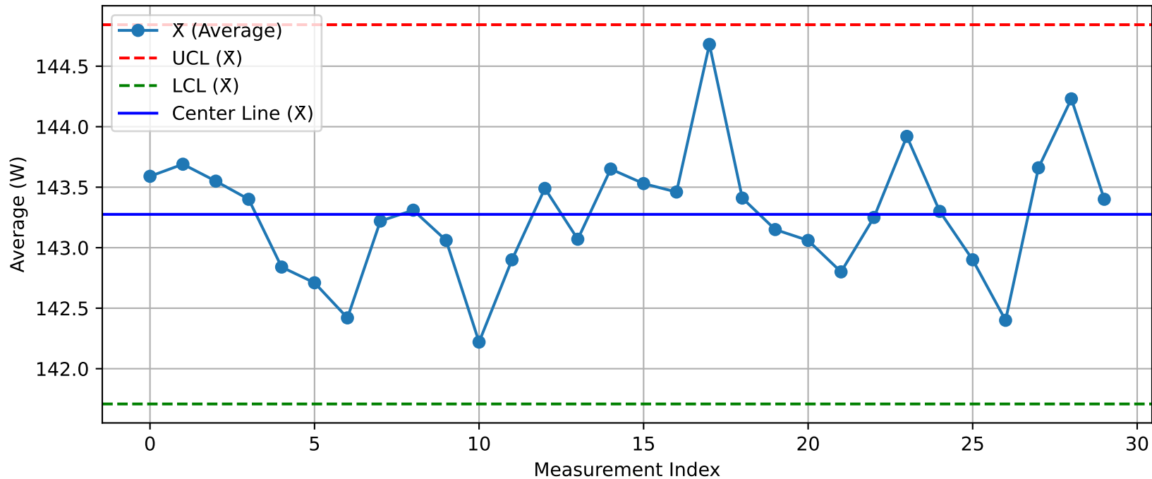
DUT - \bar{X} Chart (T36_Test2_Xint@Test.xlsx)
