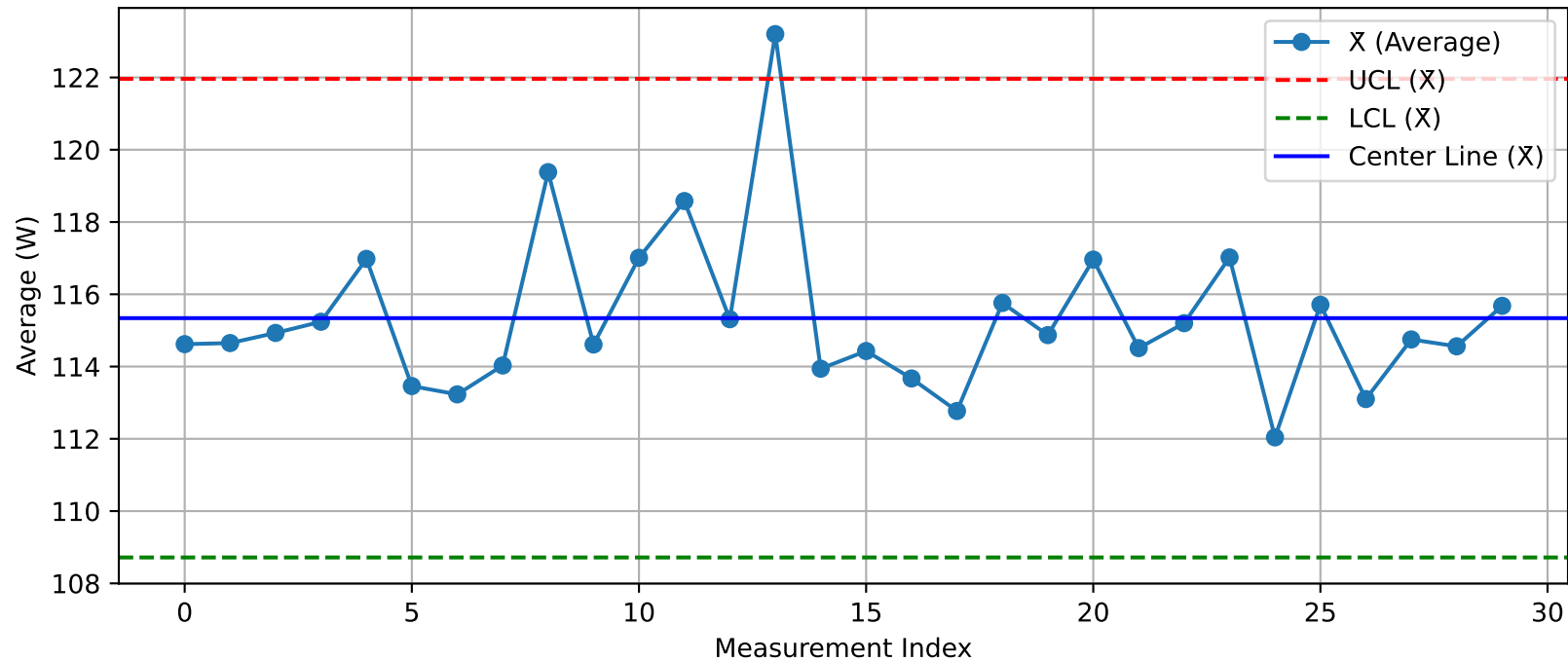
DUT - \bar{X} Chart (T49_Test2O3@Test.xlsx)
