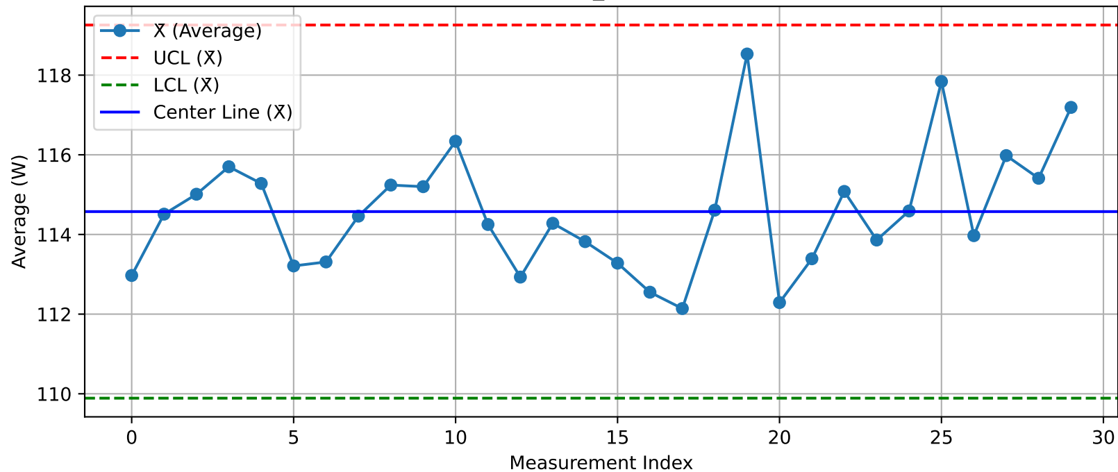
DUT - \bar{X} Chart (T16_Test100@Test.xlsx)
