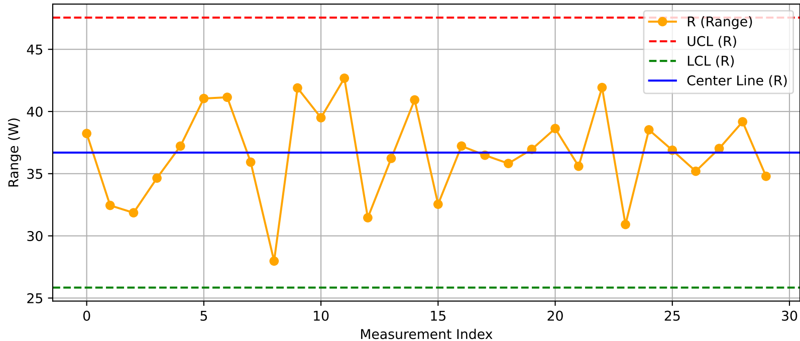
DUT - R Chart (T33_Test100@Test.xlsx)
