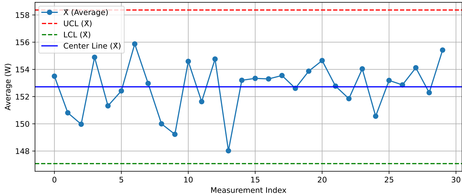
DUT - \bar{X} Chart (T17_Test1_Nuitka@Test.xlsx)
