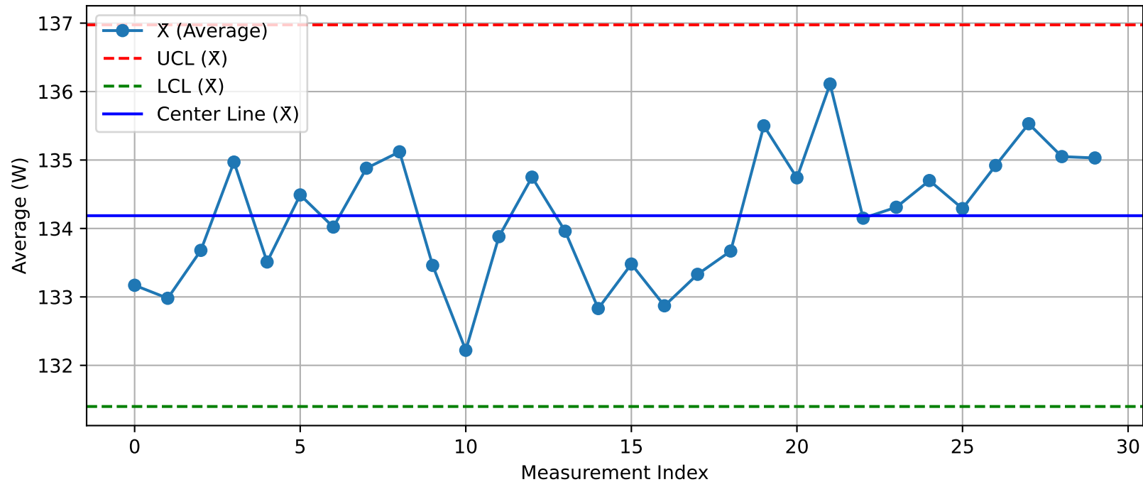
DUT - \bar{X} Chart (T40_Test1_Xint@Test.xlsx)
