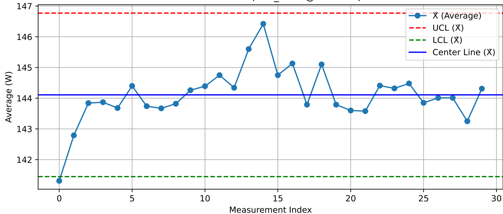
DUT - \bar{X} Chart (T51_Test1@Test.xlsx)
