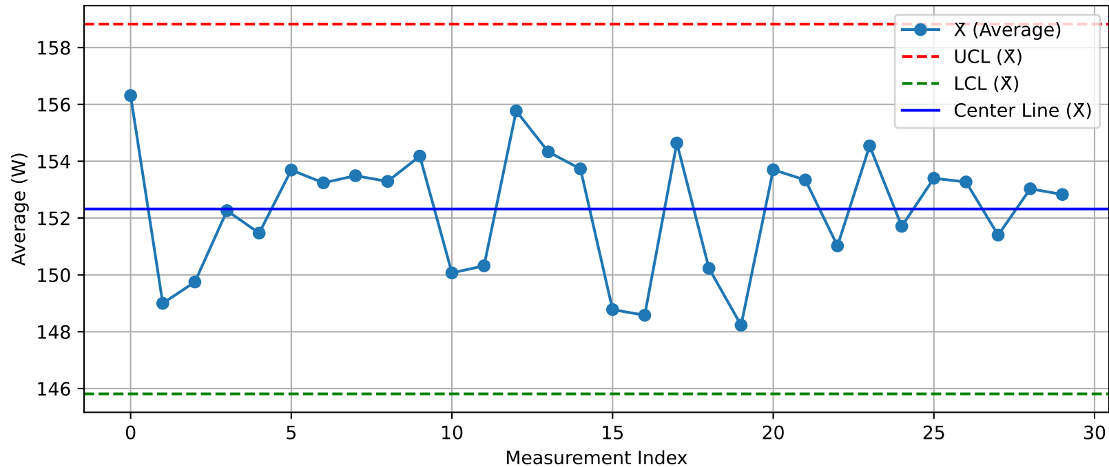
DUT - \bar{X} Chart (T50_Test2_Nuitka@Test.xlsx)
