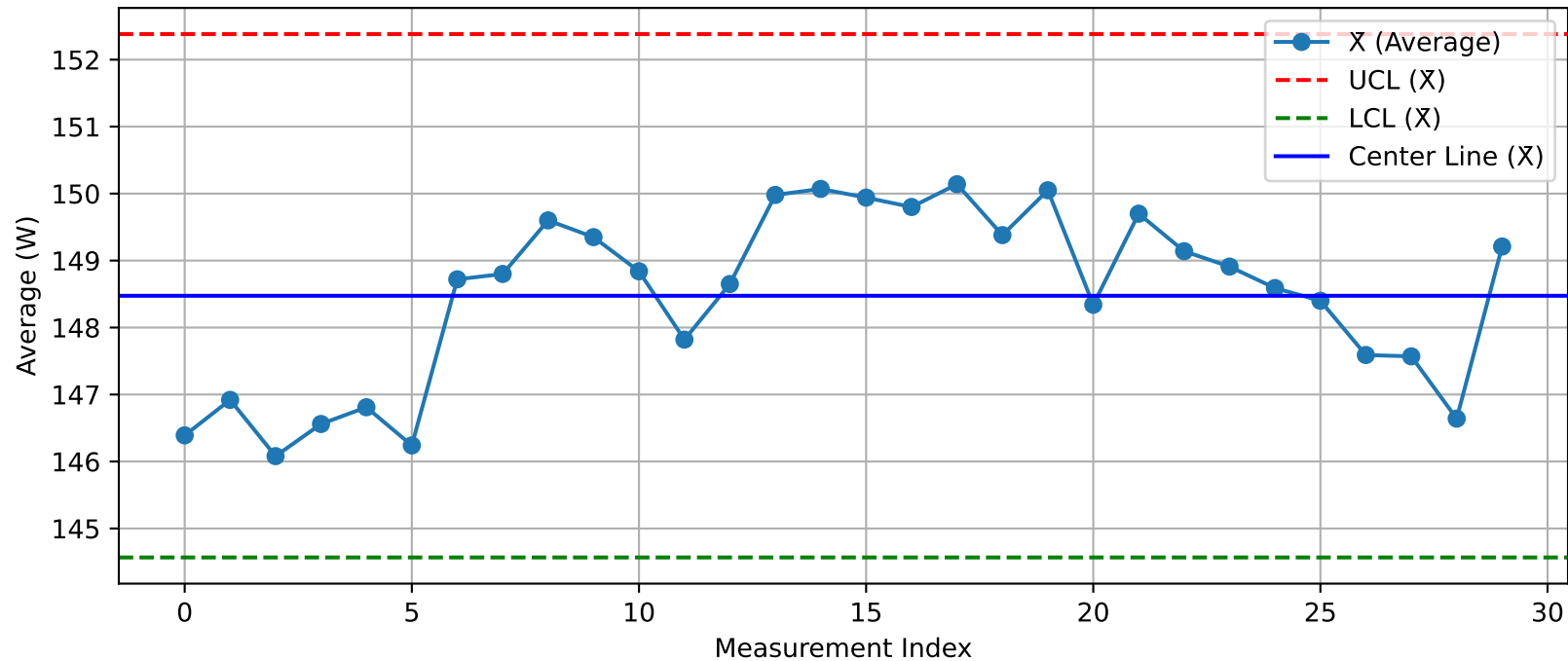
DUT - \bar{X} Chart (T10_Test1_Xint@Test.xlsx)
