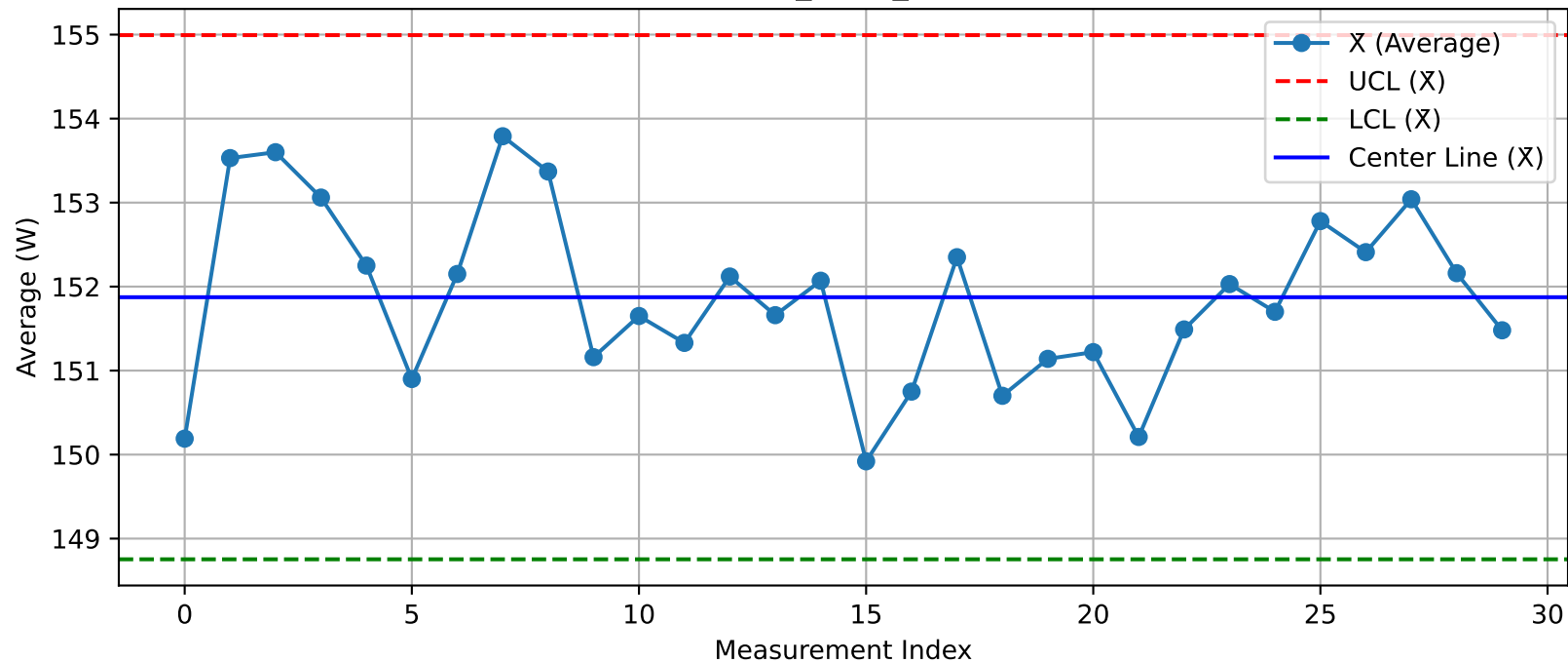
DUT - \bar{X} Chart (T25_Test1_Nuitka@Test.xlsx)
