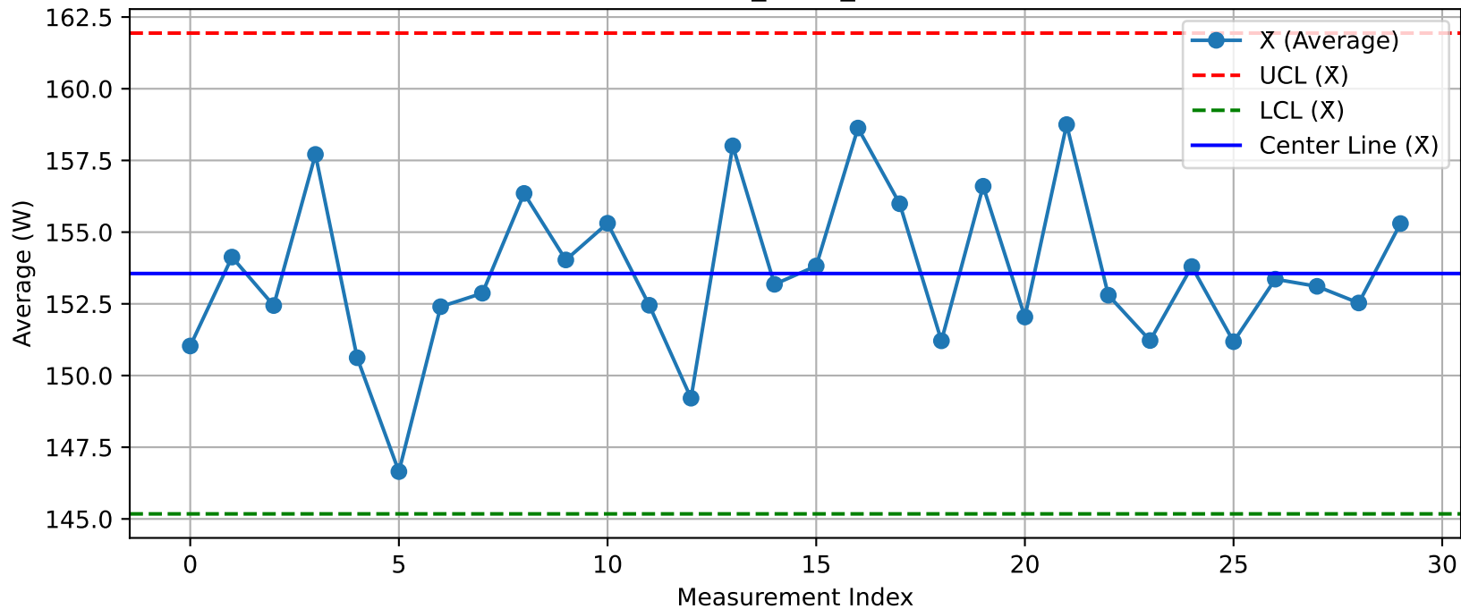
DUT - \bar{X} Chart (T29_Test1_Nuitka@Test.xlsx)
