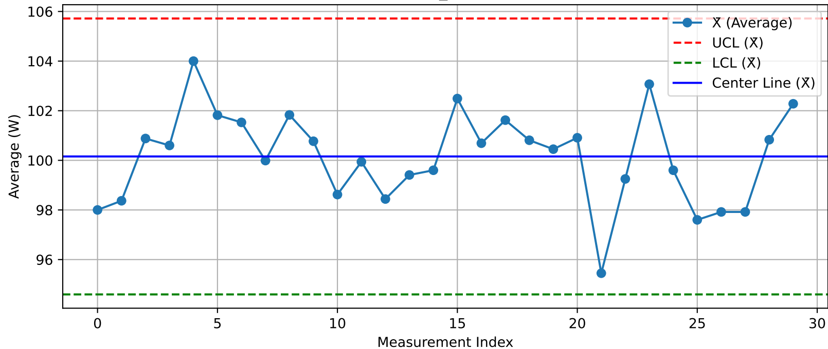
DUT - \bar{X} Chart (T10_Test2O3@Test.xlsx)
