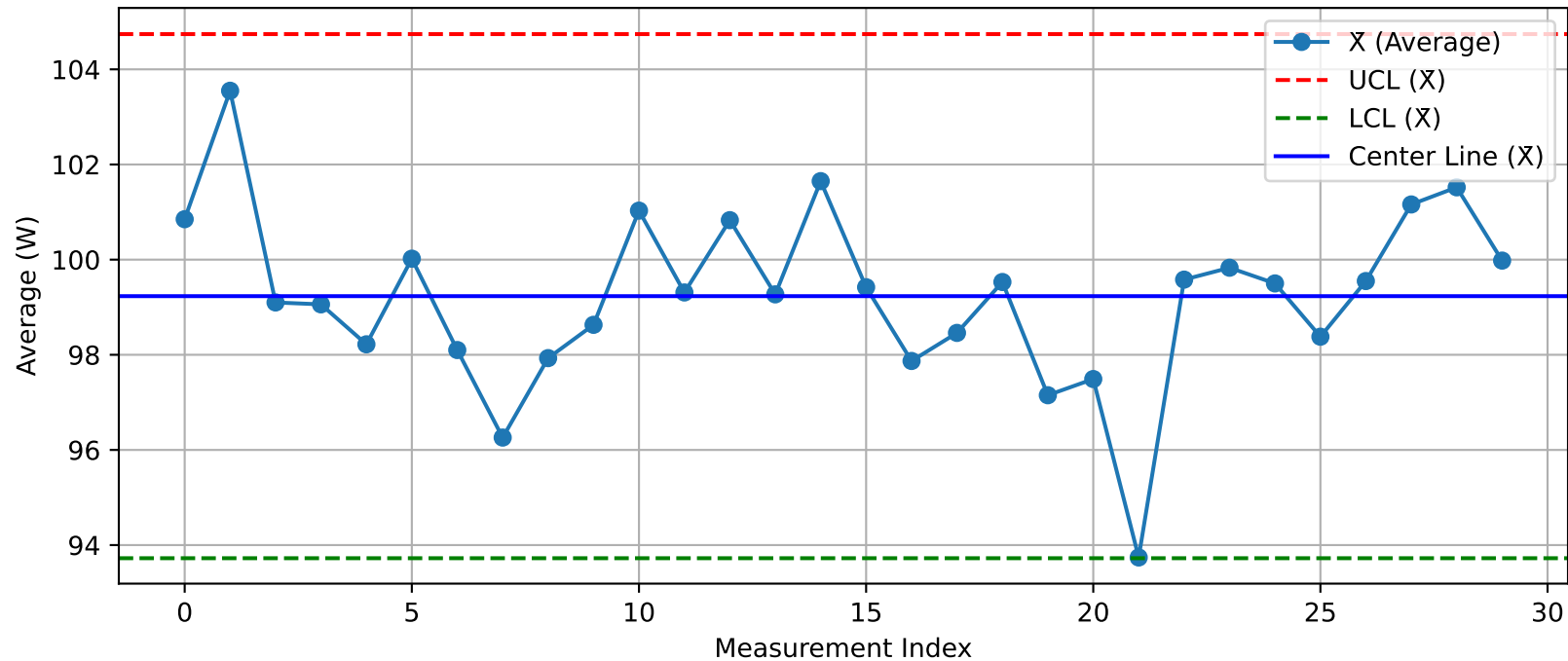
DUT - \bar{X} Chart (T50_Test103@Test.xlsx)
