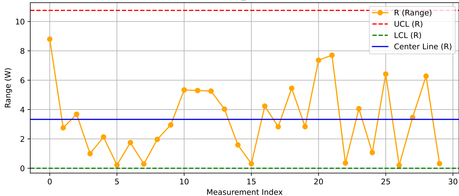
DUT - R Chart (T10_Test203@Test.xlsx)
