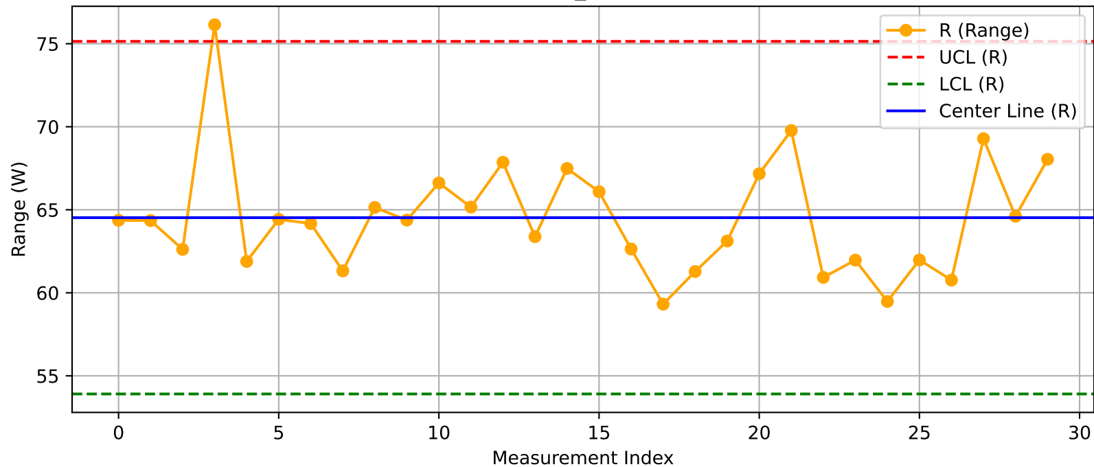
DUT - R Chart (T31_Test200@Test.xlsx)
