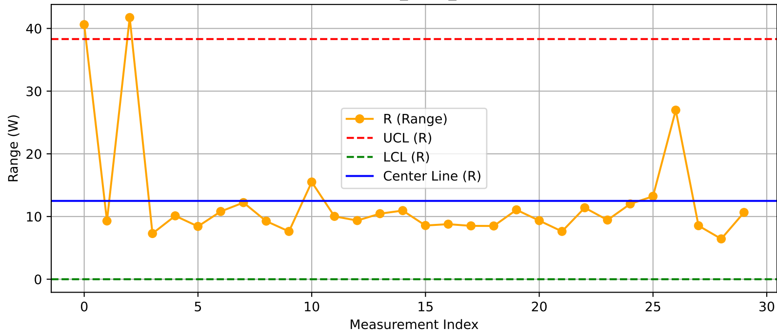
DUT - R Chart (T11_Test2_Xint@Test.xlsx)
