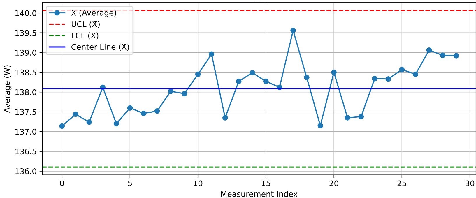
DUT - \bar{X} Chart (T40_Test200@Test.xlsx)
