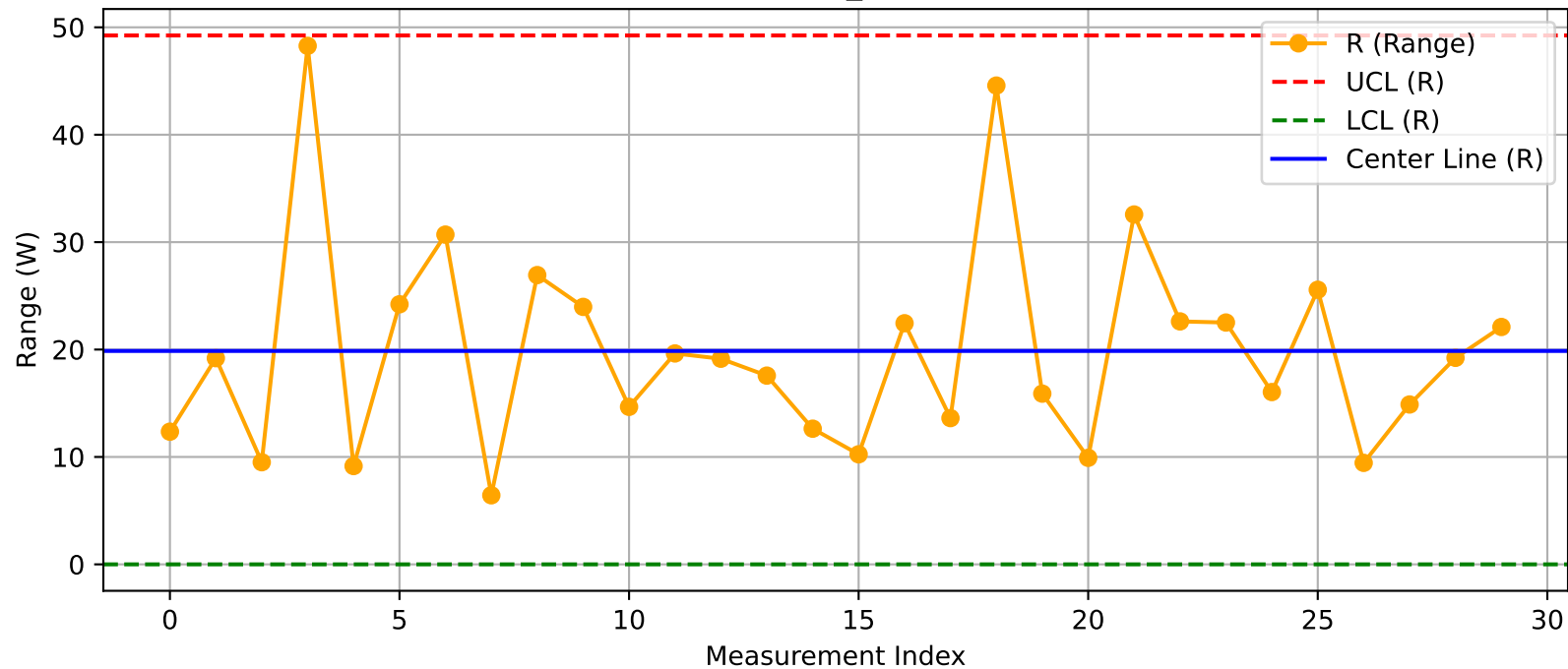
DUT - R Chart (T10_Test2@Test.xlsx)
