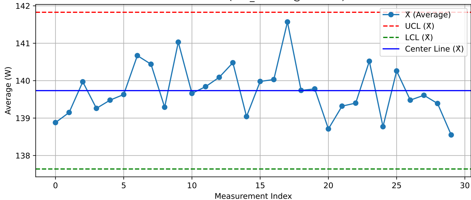
DUT - \bar{X} Chart (T13_Test100@Test.xlsx)
