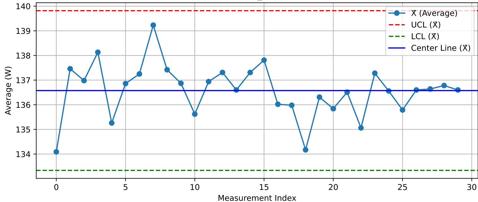
DUT - \bar{X} Chart (T7_Test1@Test.xlsx)
