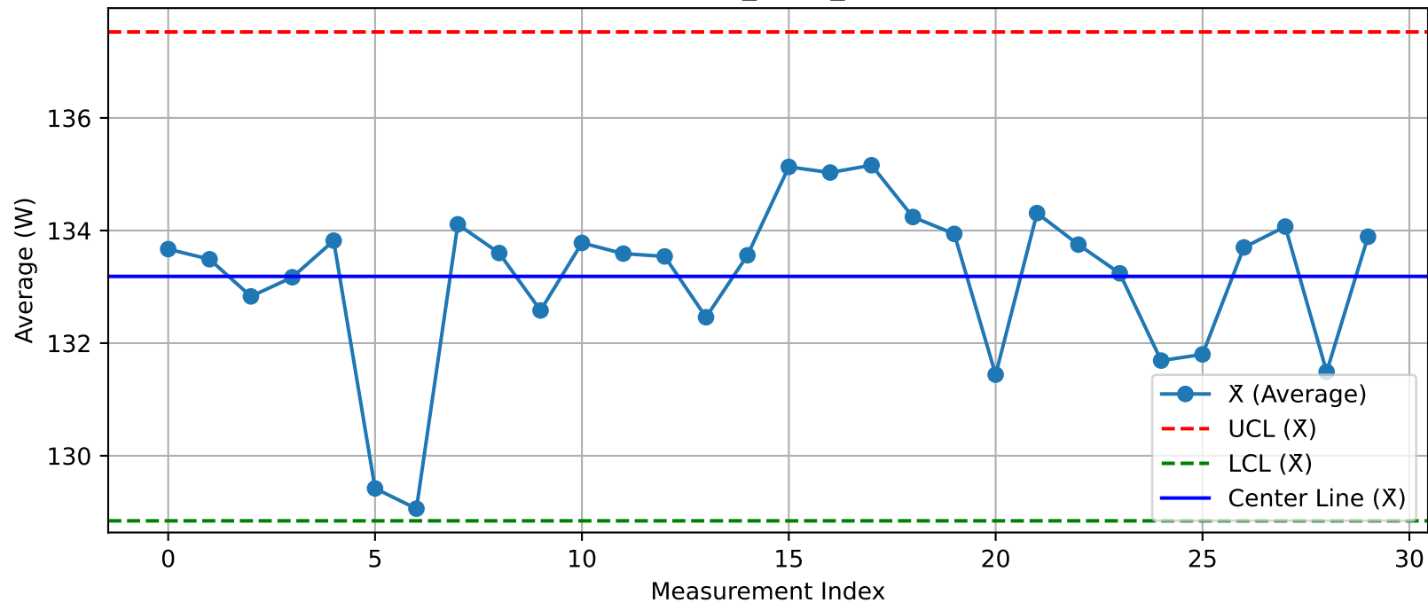
DUT - \bar{X} Chart (T29_Test1_Xint@Test.xlsx)
