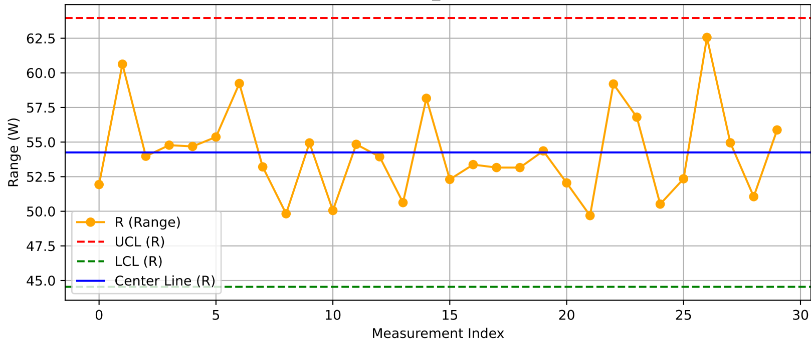
DUT - R Chart (T51_Test103@Test.xlsx)
