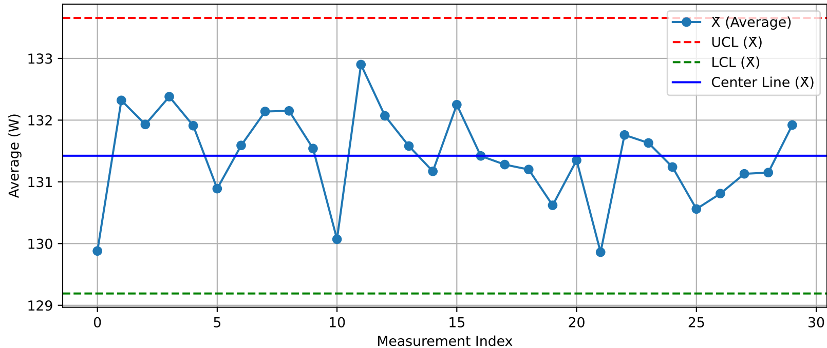
DUT - \bar{X} Chart (T12_Test1_Xint@Test.xlsx)
