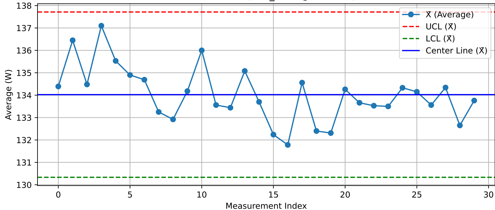
DUT - \bar{X} Chart (T19_Test2@Test.xlsx)
