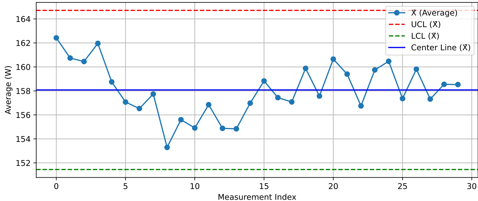
DUT - \bar{X} Chart (T20_Test2_Nuitka@Test.xlsx)
