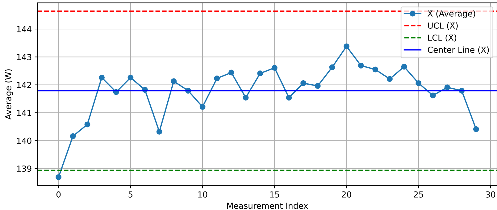
DUT - \bar{X} Chart (T40_Test100@Test.xlsx)
