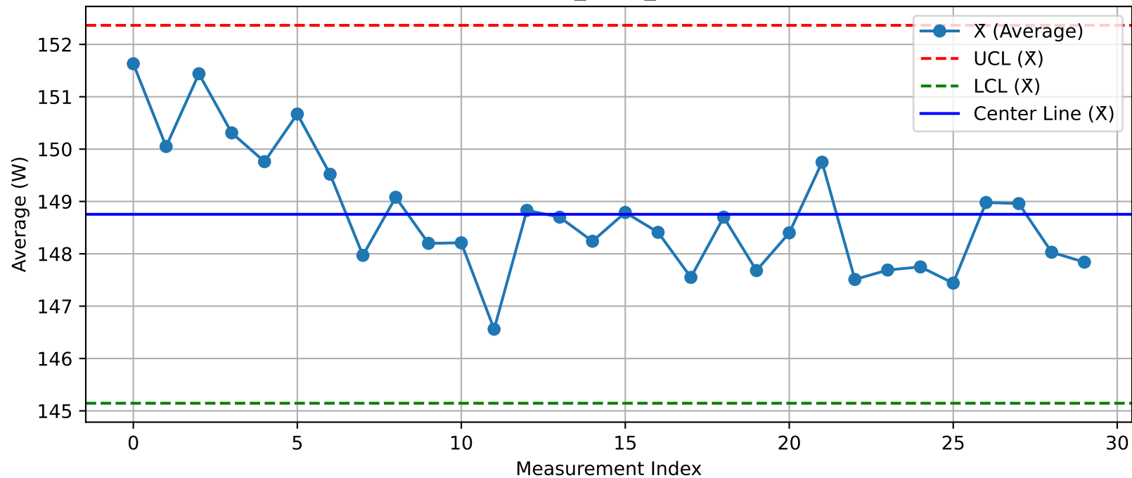
DUT - \bar{X} Chart (T26_Test2_Nuitka@Test.xlsx)
