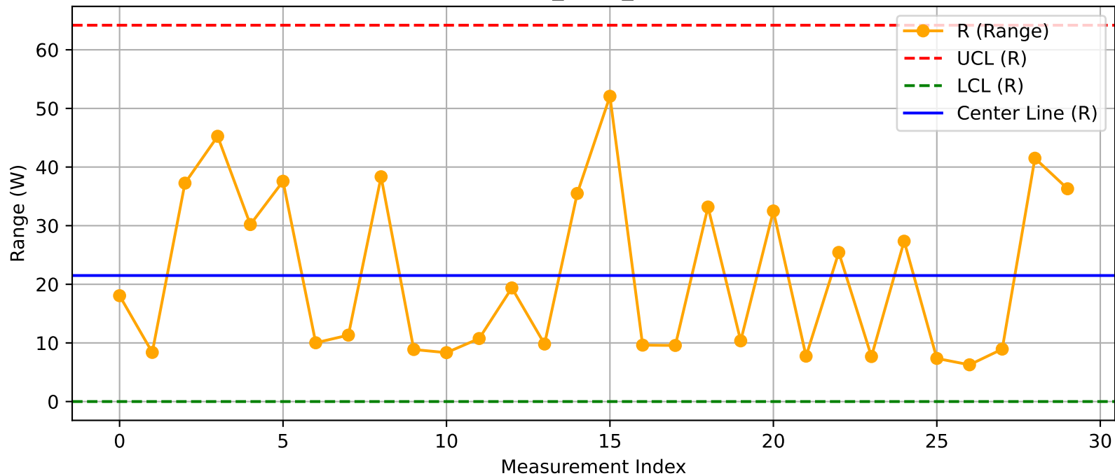
DUT - R Chart (T5_Test2_Nuitka@Test.xlsx)
