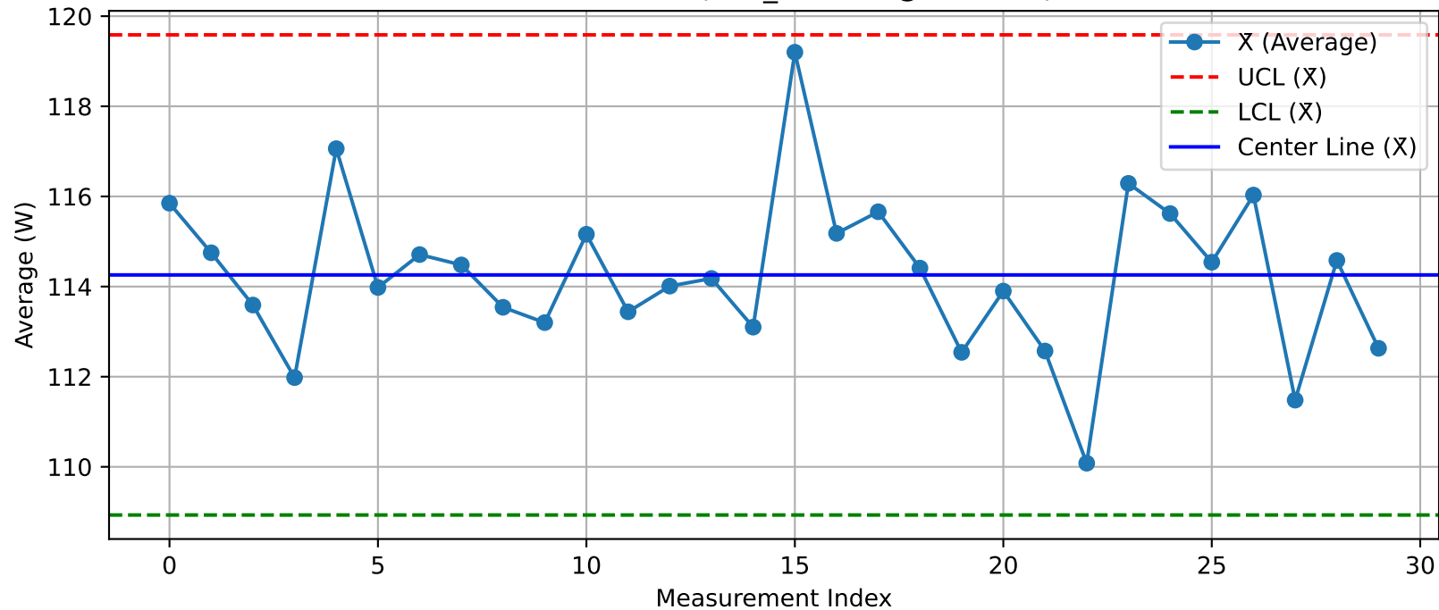
DUT - \bar{X} Chart (T26_Test2O3@Test.xlsx)
