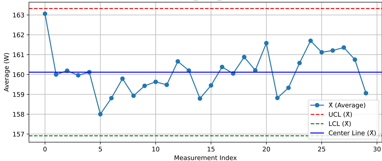
DUT - \bar{X} Chart (T10_Test1_Nuitka@Test.xlsx)
