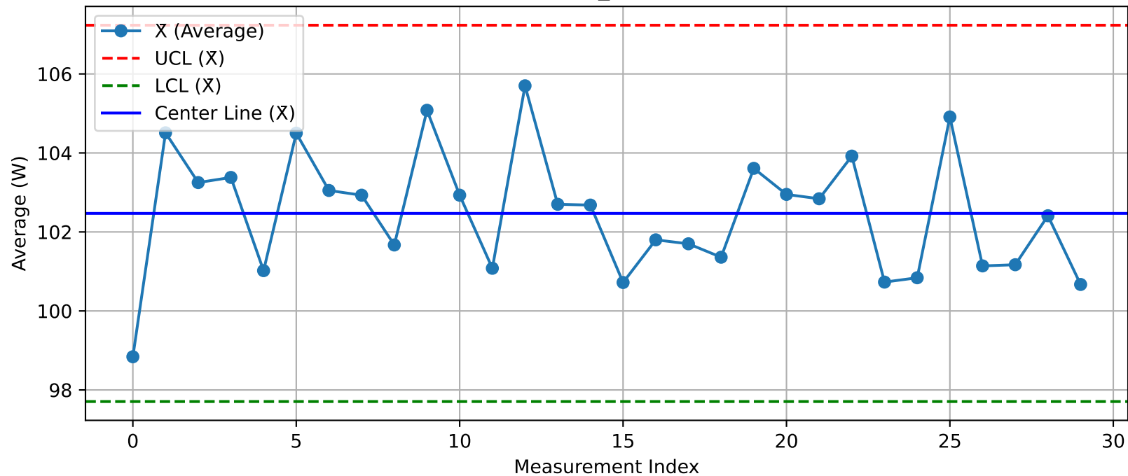
DUT - \bar{X} Chart (T29_Test100@Test.xlsx)
