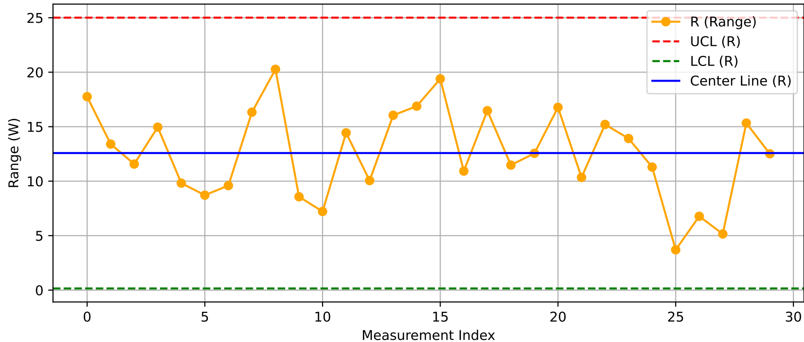
DUT - R Chart (T29_Test200@Test.xlsx)
