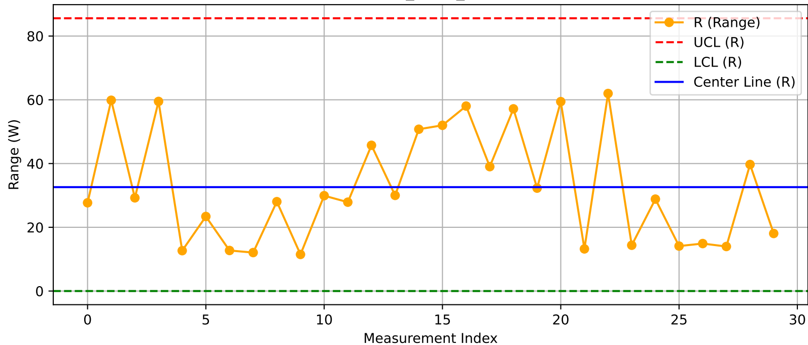
DUT - R Chart (T20_Test1_Nuitka@Test.xlsx)
