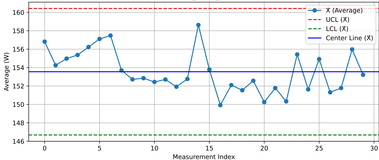
DUT - \bar{X} Chart (T20_Test1_Nuitka@Test.xlsx)
