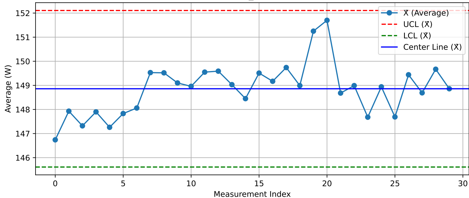
DUT - \bar{X} Chart (T05_Test100@Test.xlsx)
