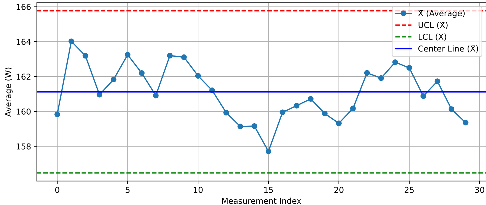
DUT - \bar{X} Chart (T33_Test1@Test.xlsx)
