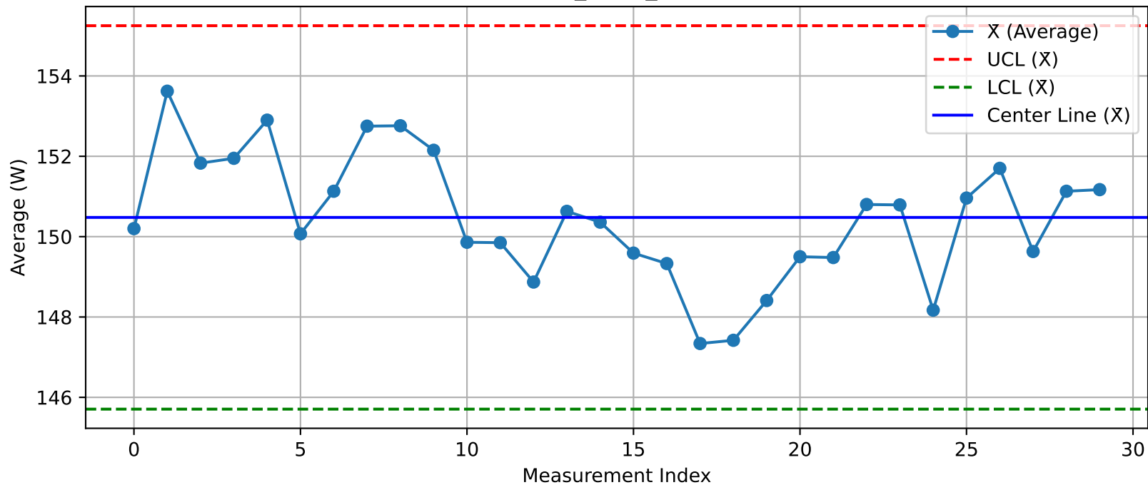
DUT - \bar{X} Chart (T8_Test1_Nuitka@Test.xlsx)
