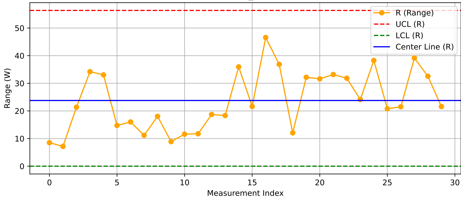
DUT - R Chart (T16_Test1@Test.xlsx)
