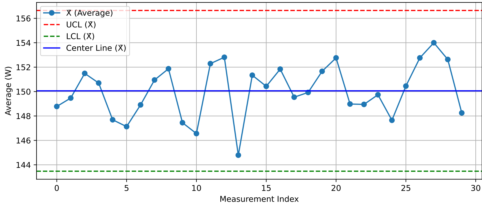
DUT - \bar{X} Chart (T32_Test1_Nuitka@Test.xlsx)
