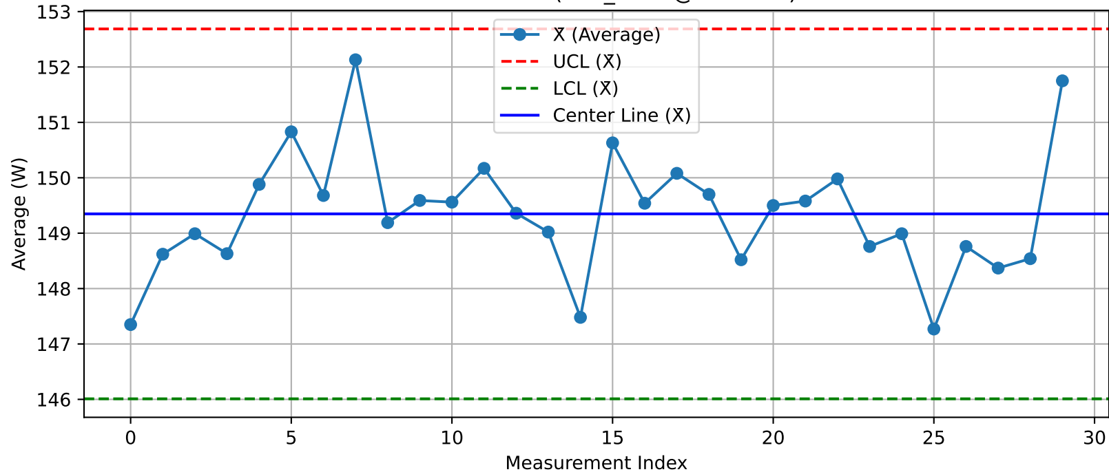
DUT - \bar{X} Chart (T50_Test1@Test.xlsx)
