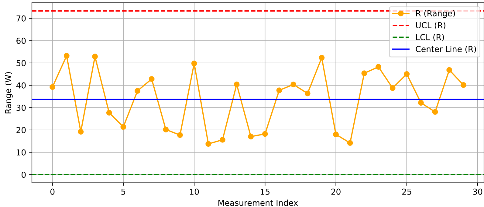
DUT - R Chart (T51_Test2_Nuitka@Test.xlsx)
