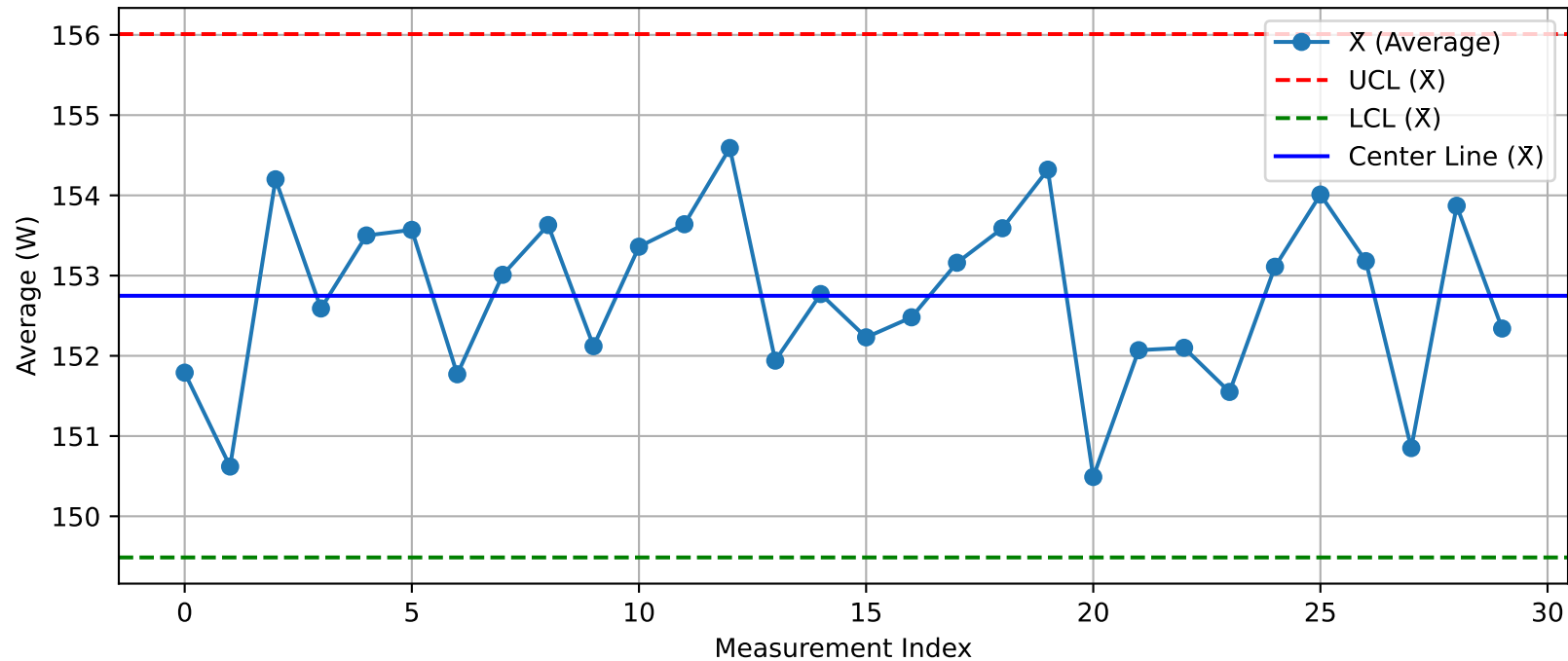
DUT - \bar{X} Chart (T16_Test2@Test.xlsx)
