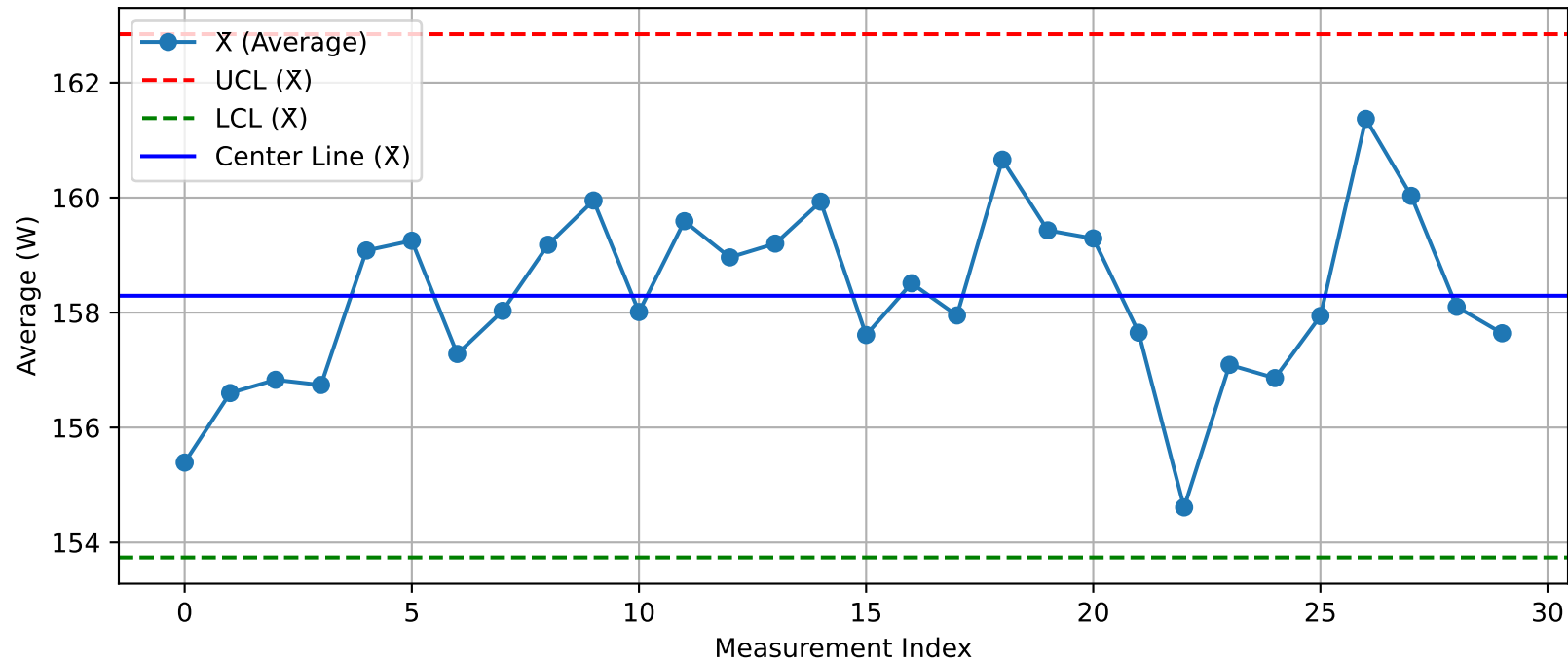
DUT - \bar{X} Chart (T51_Test2_Nuitka@Test.xlsx)
