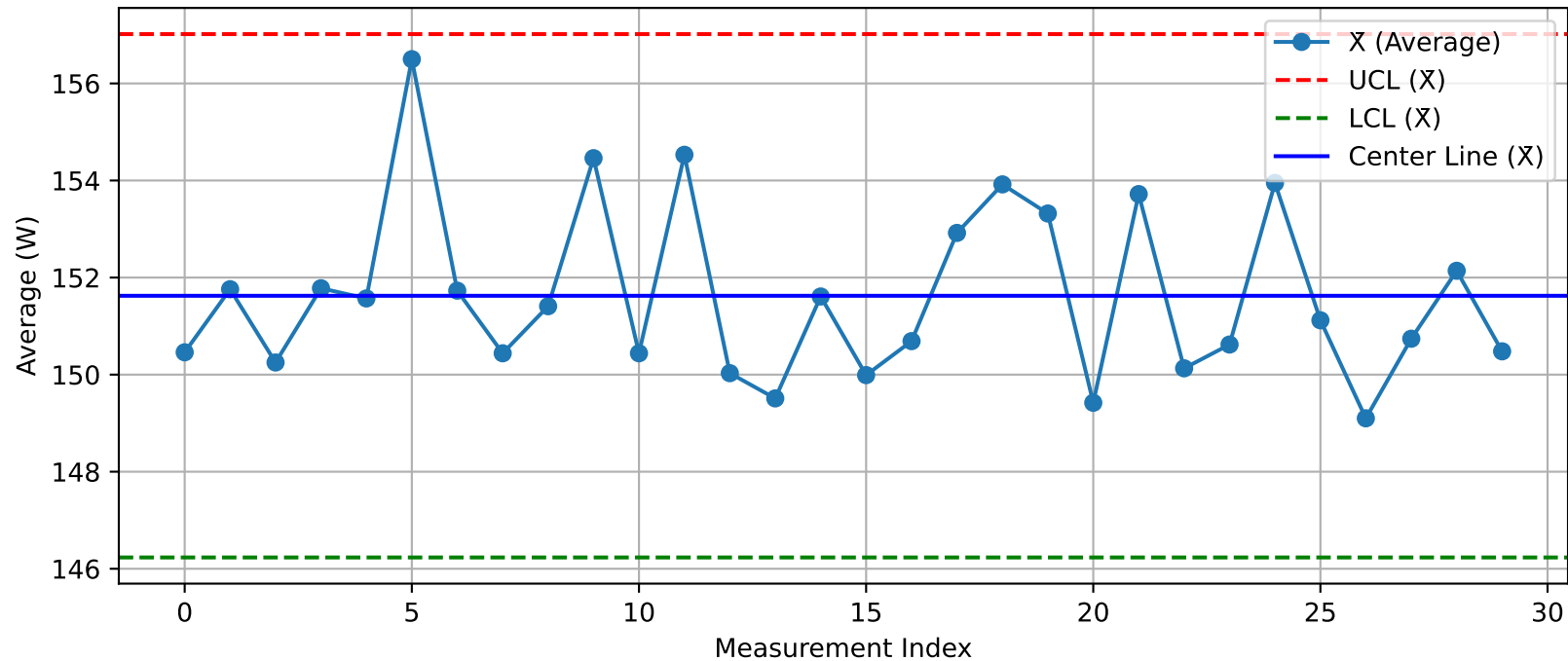
DUT - \bar{X} Chart (T10_Test2_Nuitka@Test.xlsx)
