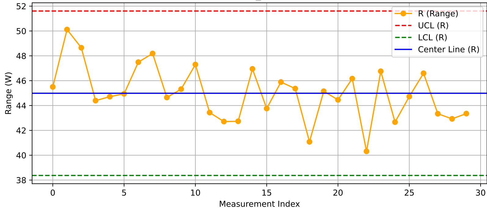
DUT - R Chart (T13_Test200@Test.xlsx)
