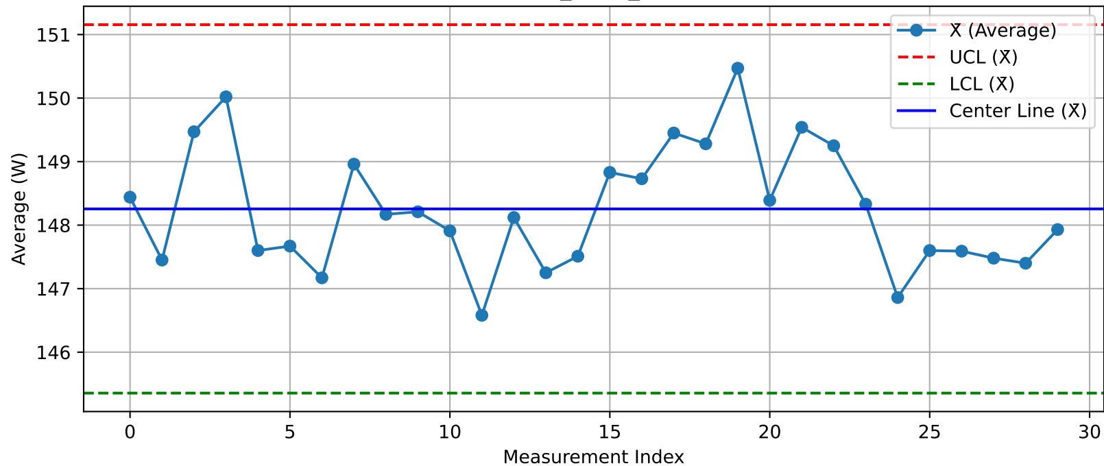
DUT - \bar{X} Chart (T28_Test2_Nuitka@Test.xlsx)
