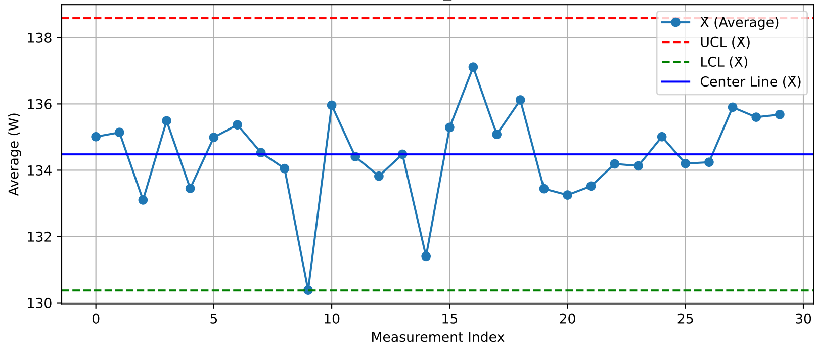
DUT - \bar{X} Chart (T32_Test2@Test.xlsx)
