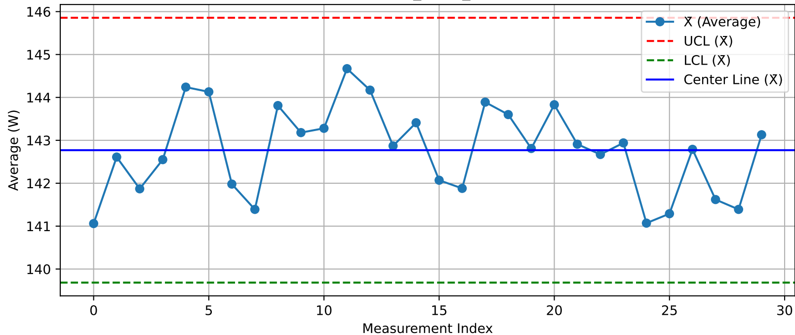
DUT - \bar{X} Chart (T25_Test1_Xint@Test.xlsx)
