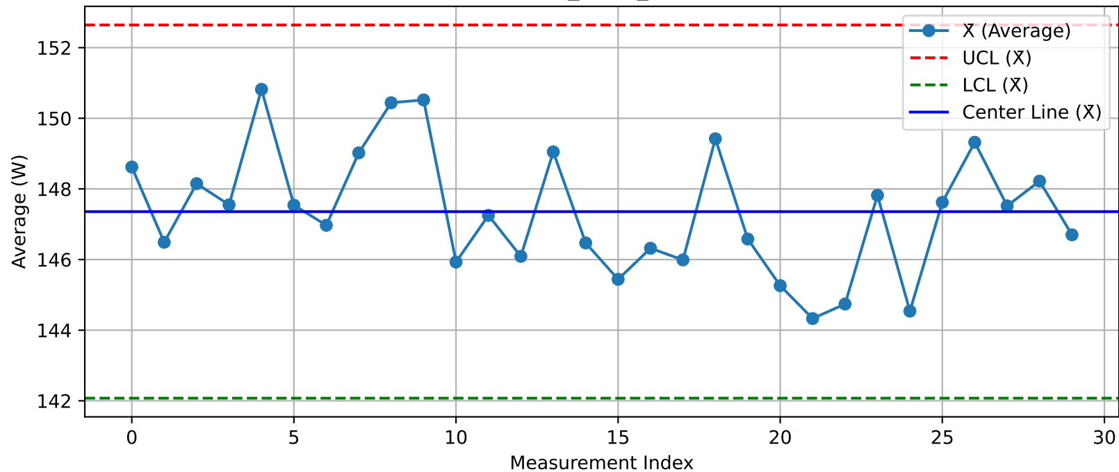
DUT - \bar{X} Chart (T12_Test1_Nuitka@Test.xlsx)
