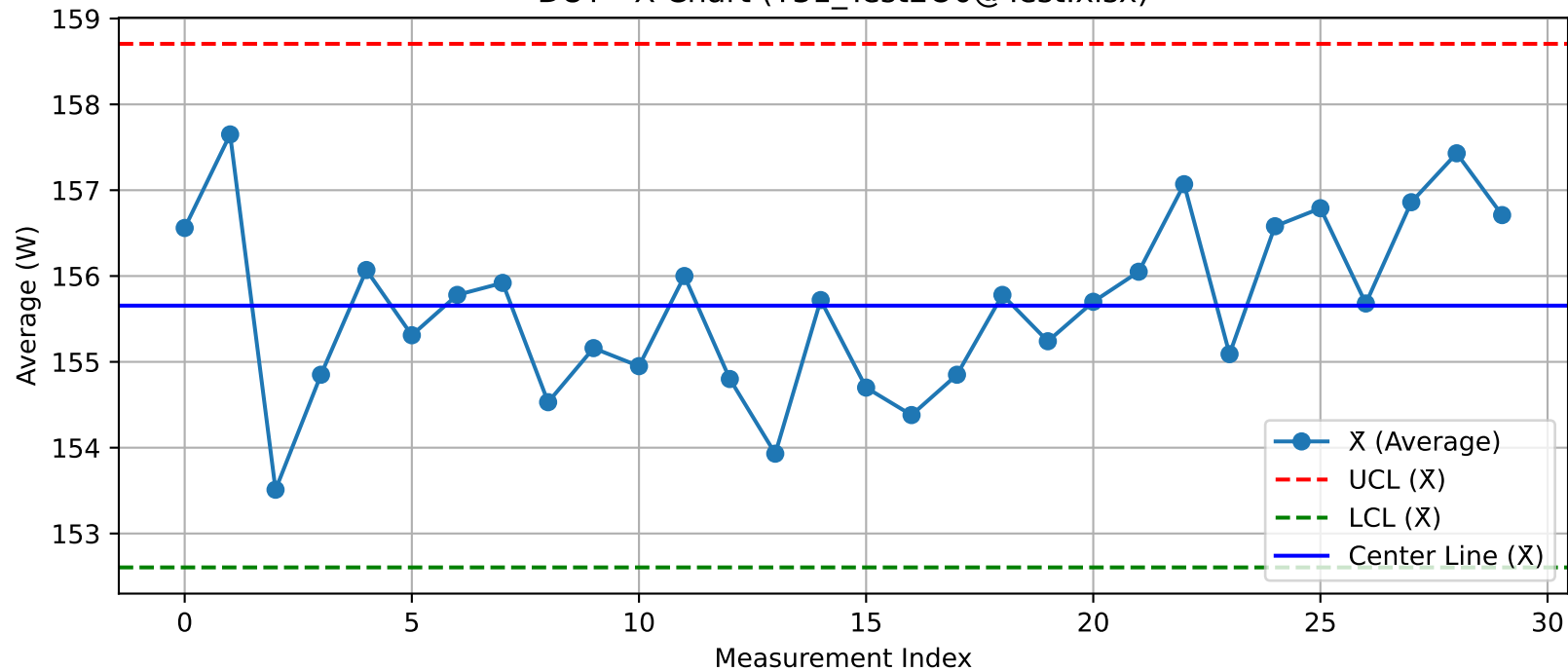
DUT - \bar{X} Chart (T31_Test200@Test.xlsx)
