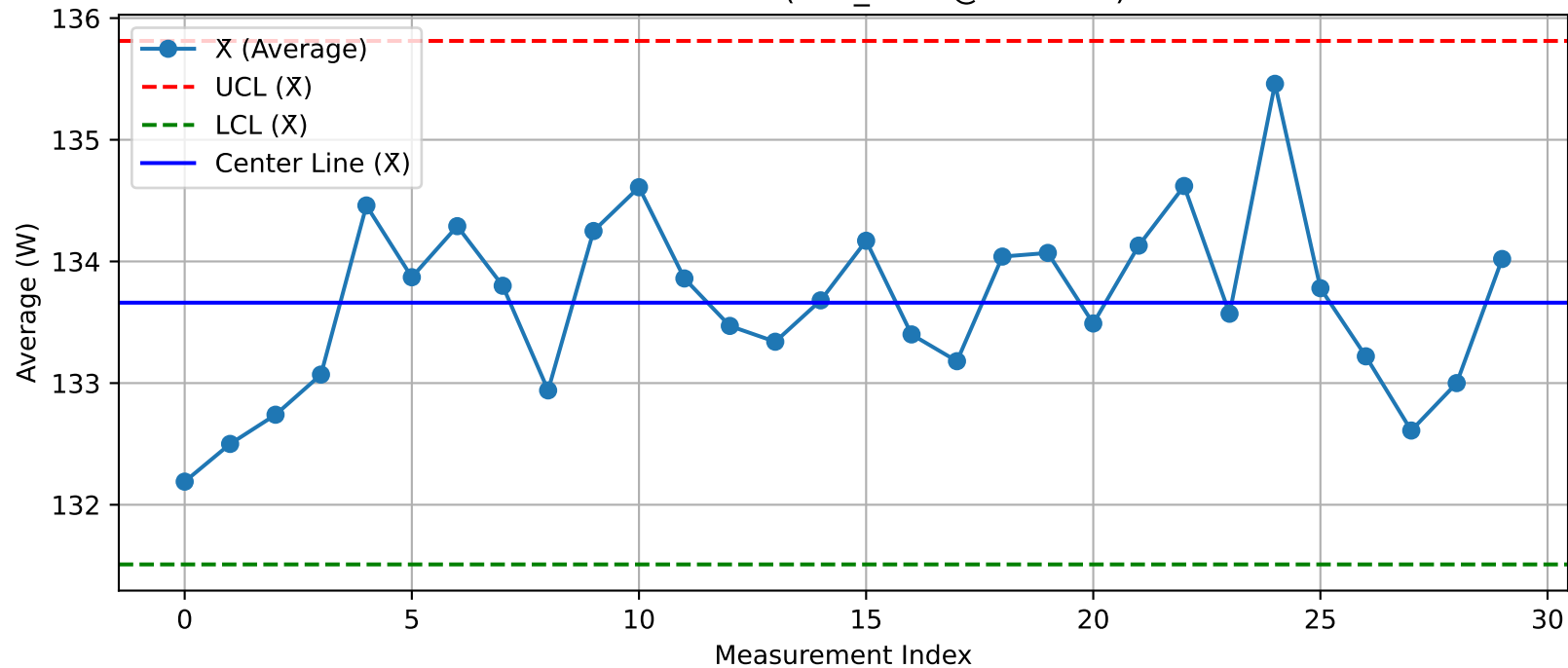
DUT - \bar{X} Chart (T13_Test1@Test.xlsx)
