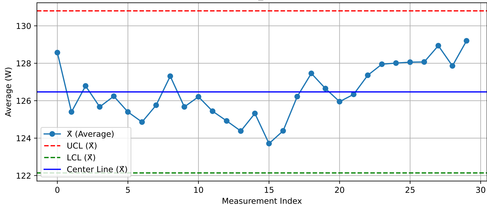
DUT - \bar{X} Chart (T04_Test200@Test.xlsx)
