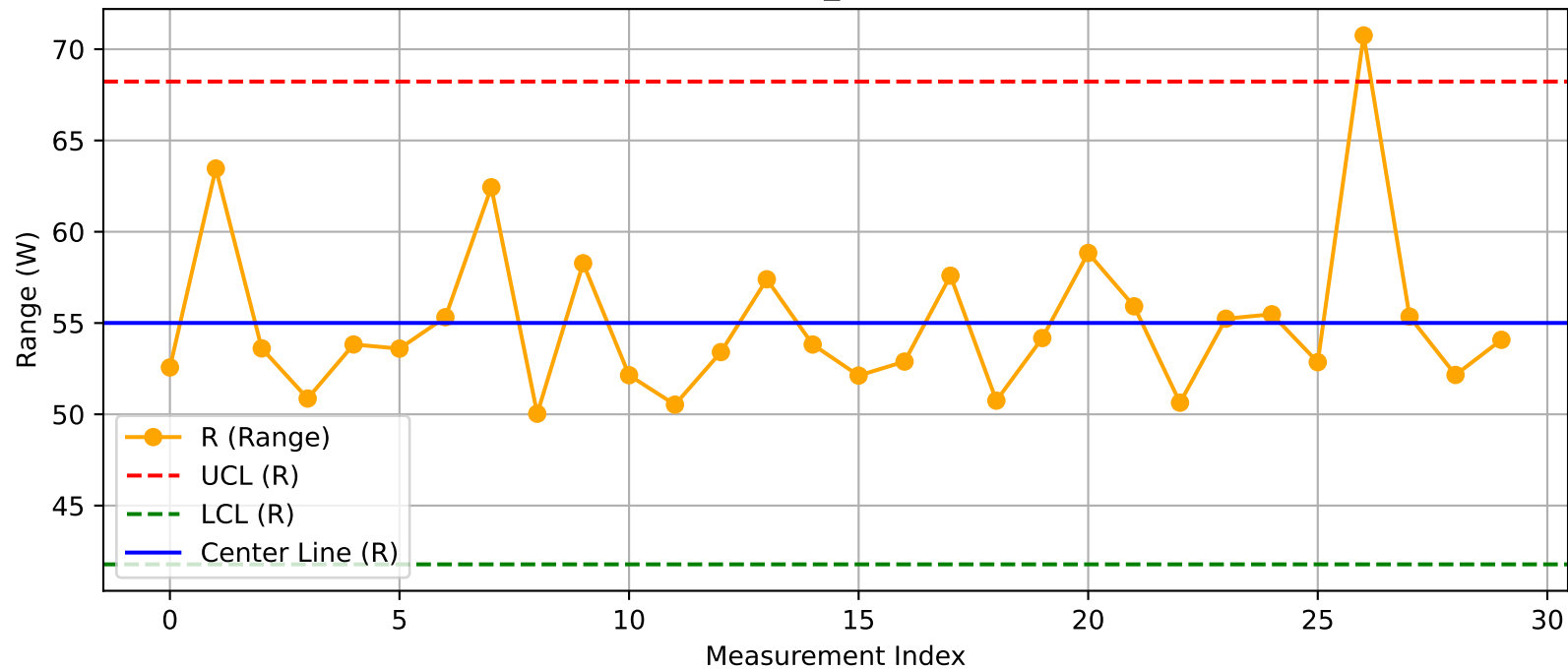
DUT - R Chart (T05_Test100@Test.xlsx)
