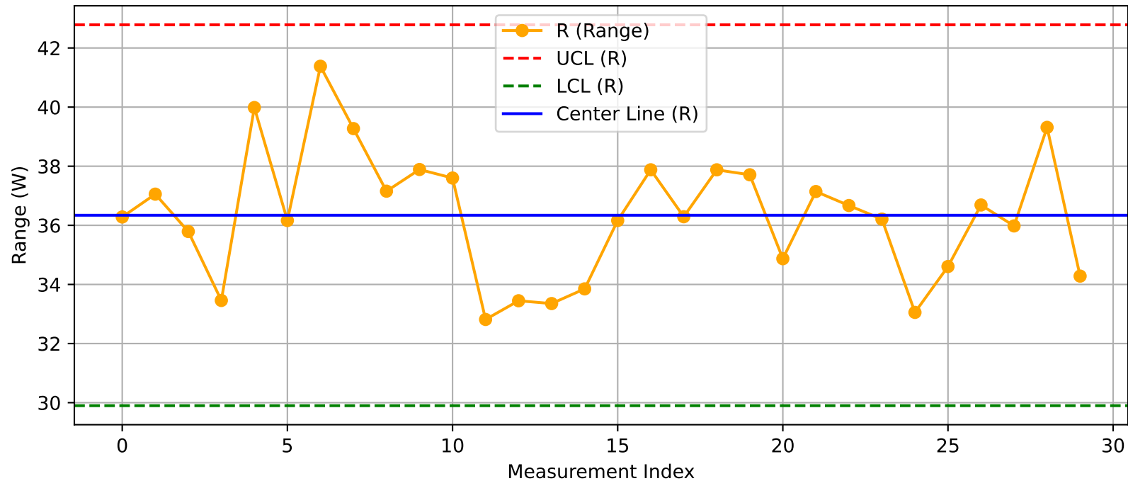
DUT - R Chart (T07_Test2O3@Test.xlsx)
