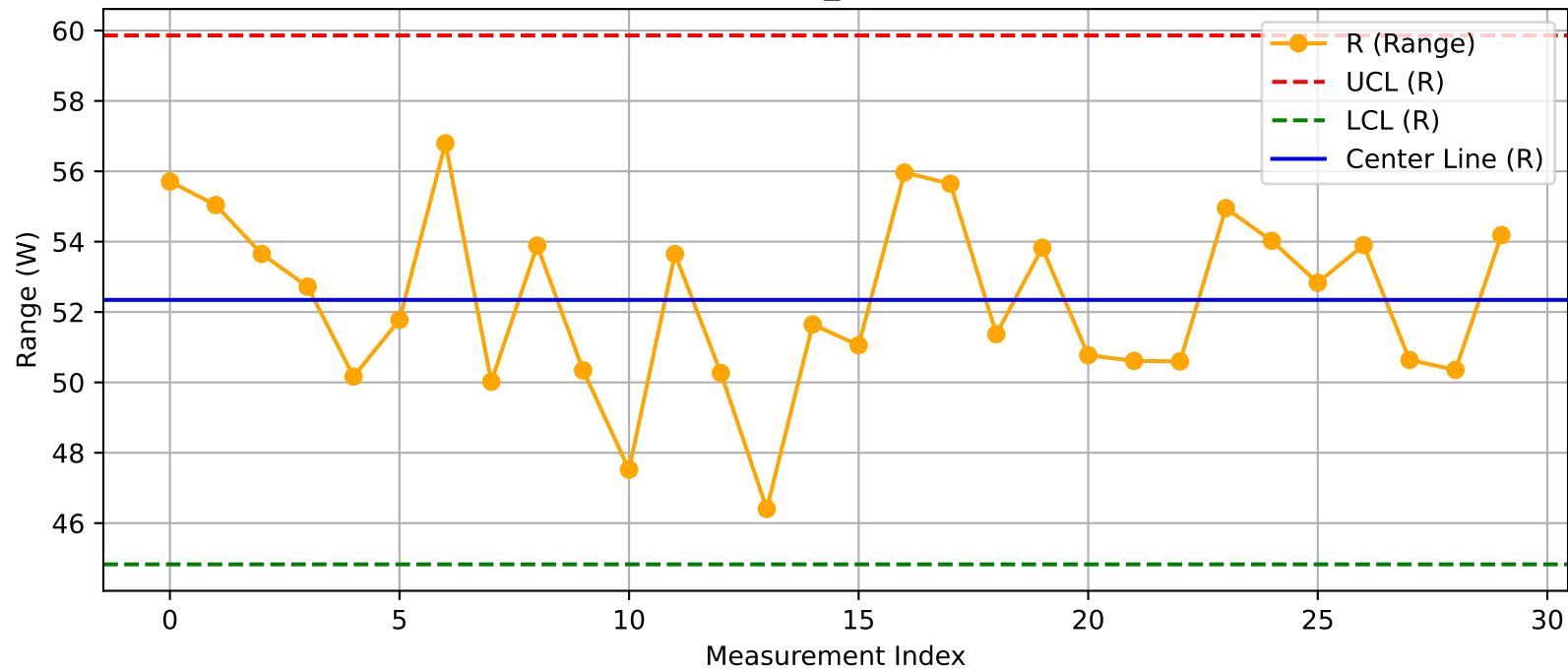
DUT - R Chart (T08_Test100@Test.xlsx)
