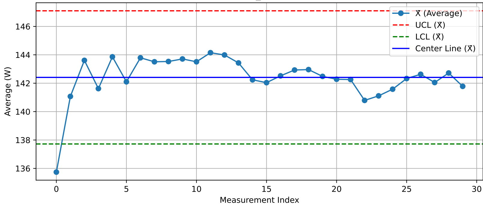
DUT - \bar{X} Chart (T08_Test100@Test.xlsx)
