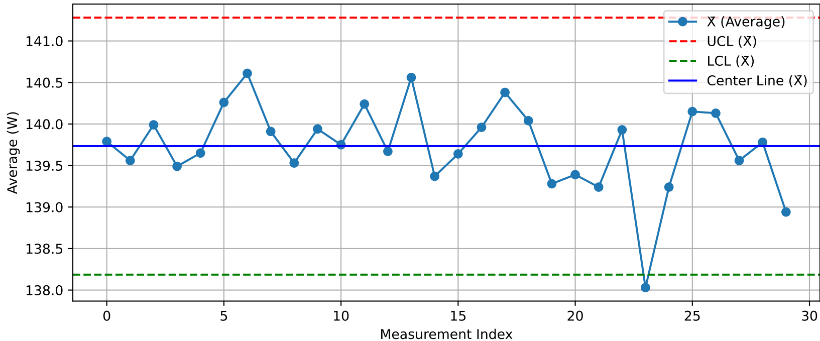
DUT - \bar{X} Chart (T08_Test103@Test.xlsx)
