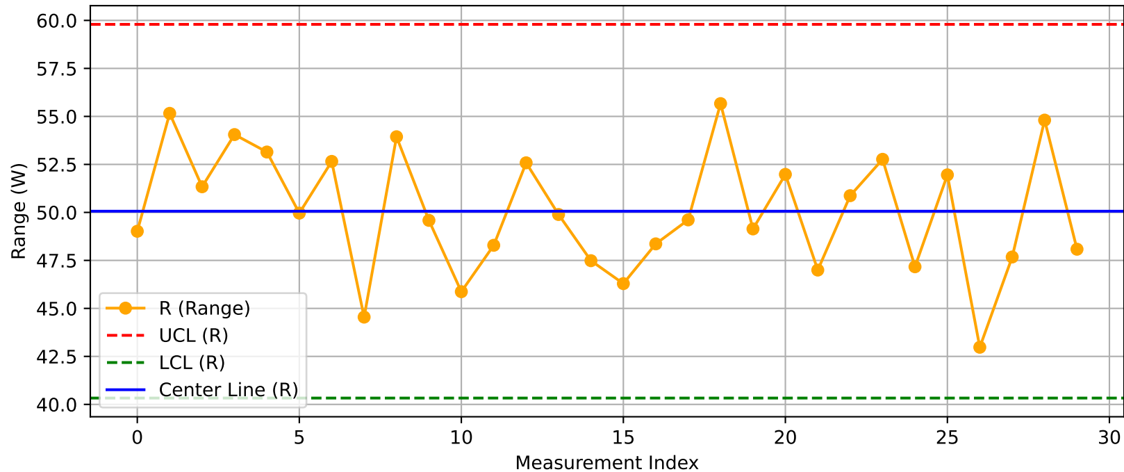
DUT - R Chart (T08_Test200@Test.xlsx)
