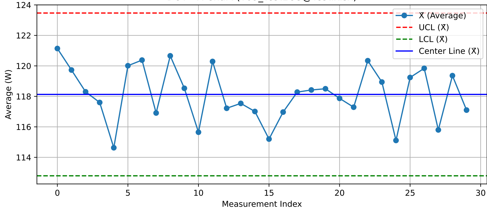
DUT - \bar{X} Chart (T09_Test103@Test.xlsx)
