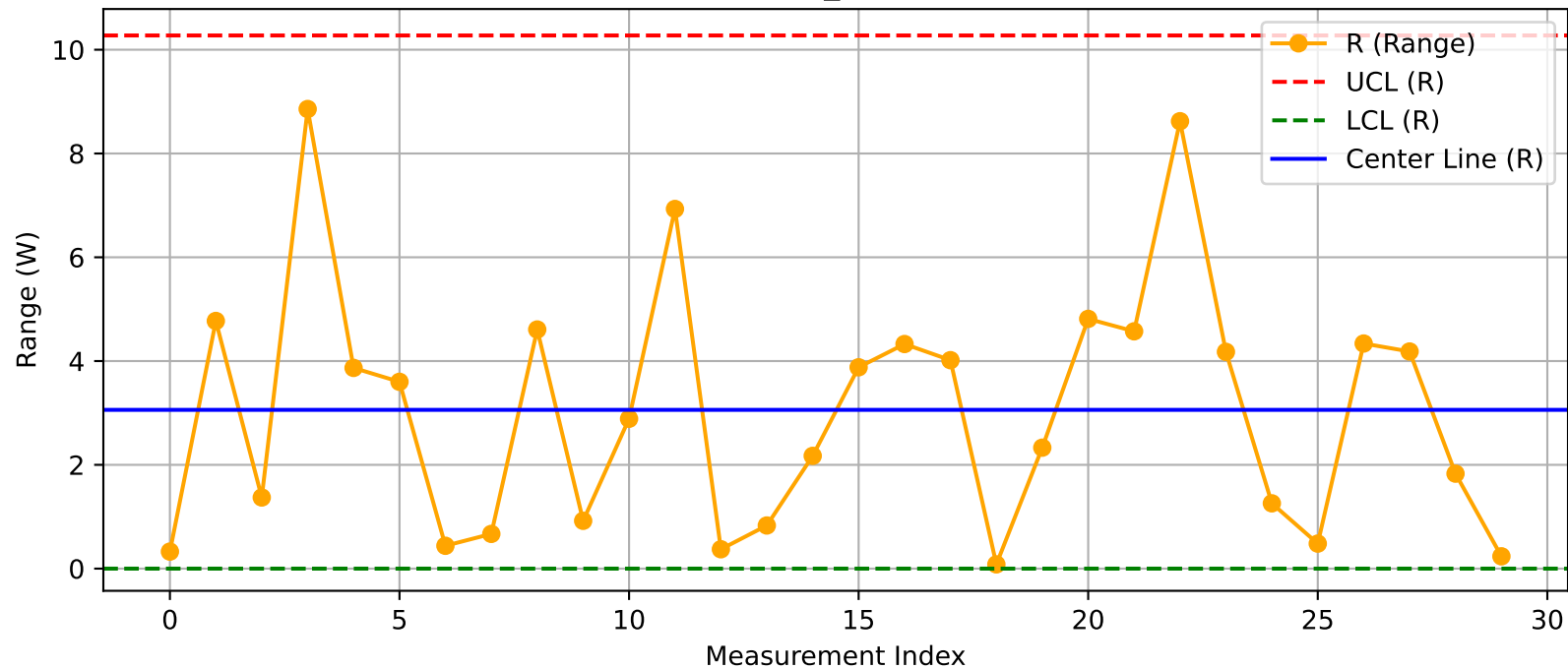
DUT - R Chart (T09_Test2O3@Test.xlsx)
