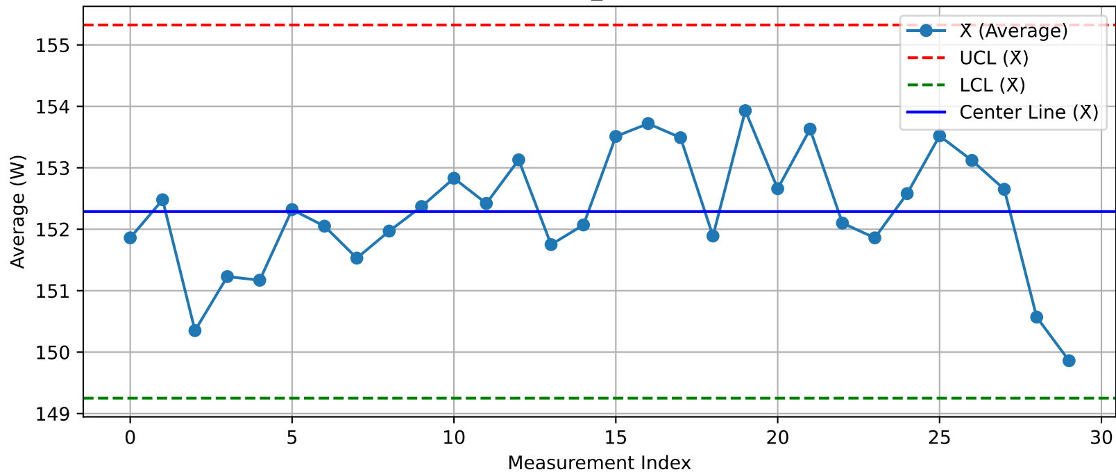
DUT - \bar{X} Chart (T10_Test1O3@Test.xlsx)
