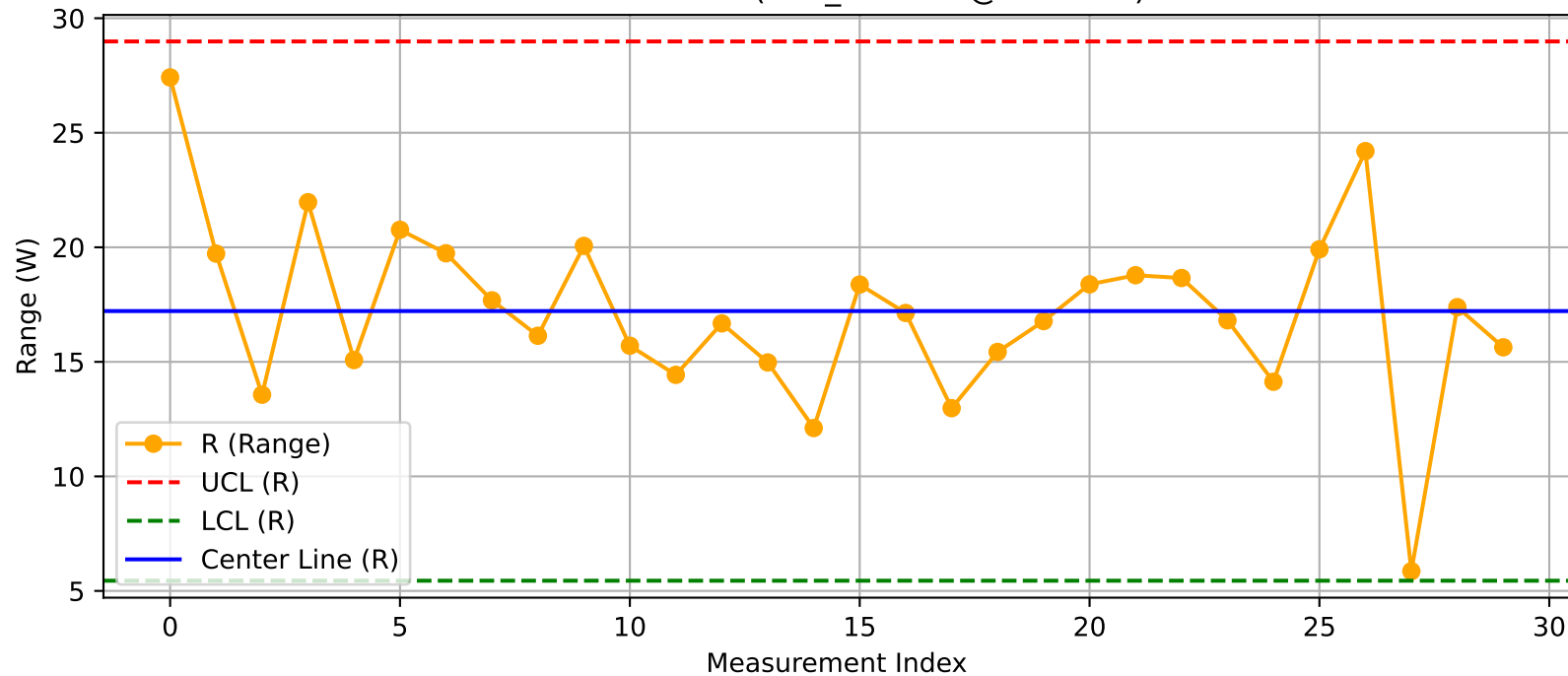
DUT - R Chart (T10_Test200@Test.xlsx)
