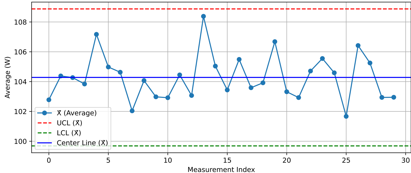
DUT - \bar{X} Chart (T10_Test203@Test.xlsx)
