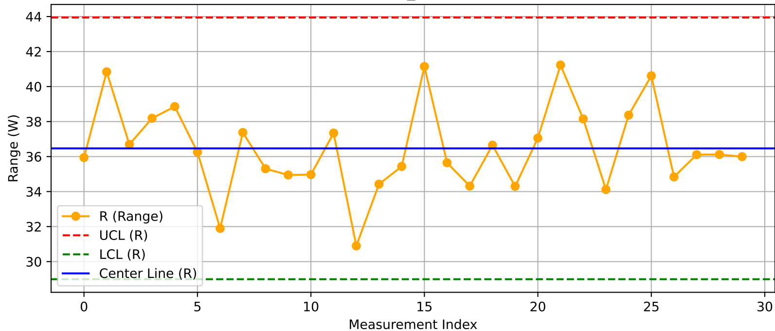
DUT - R Chart (T11_Test103@Test.xlsx)
