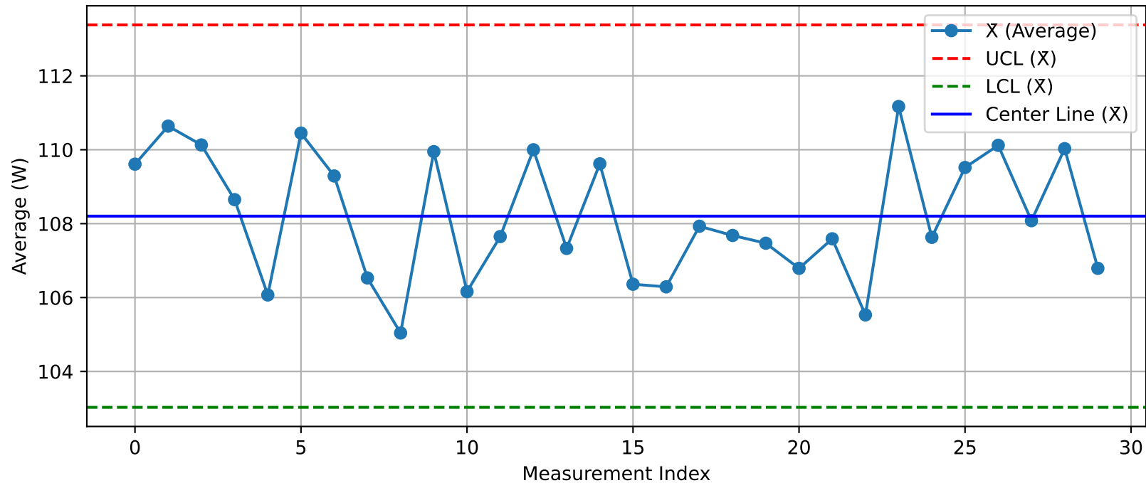
DUT - \bar{X} Chart (T11_Test203@Test.xlsx)
