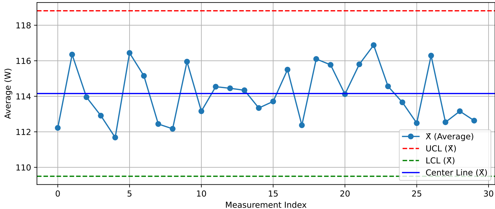
DUT - \bar{X} Chart (T12_Test100@Test.xlsx)
