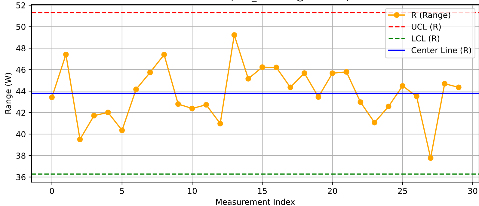
DUT - R Chart (T13_Test203@Test.xlsx)
