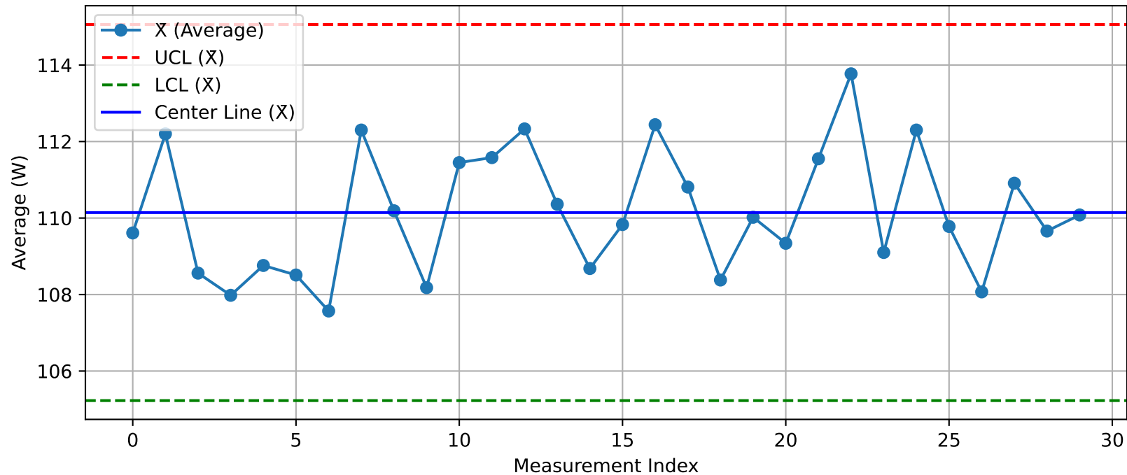
DUT - \bar{X} Chart (T16_Test200@Test.xlsx)
